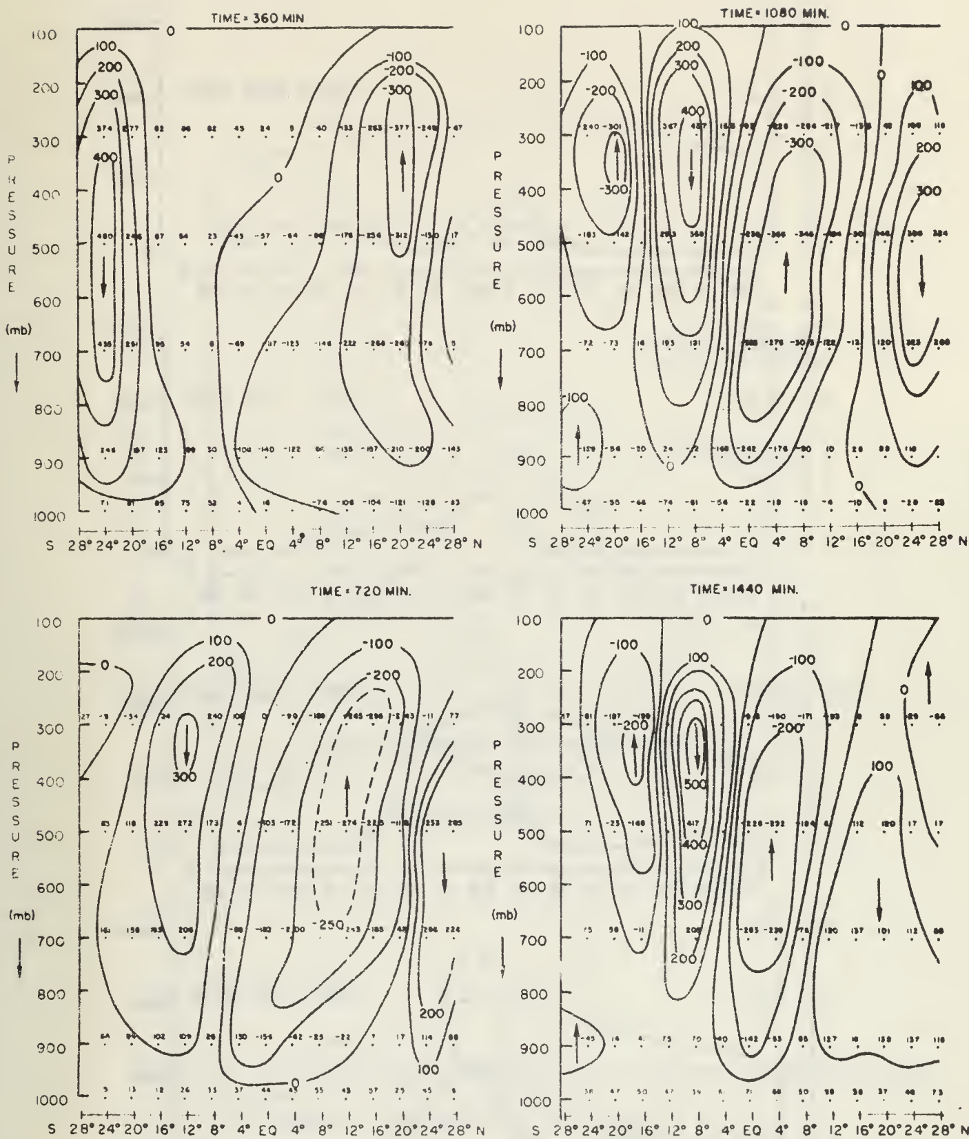
Fig. 12. Vertical cross-section of vertical motion ( 10^{-5} millibar/sec) at 6, 12, 18 and 24 hours of forecast time. This cross section is taken in a south-north plane at 152^{\circ}\text{W} longitude, and it intersects the ITCZ.
