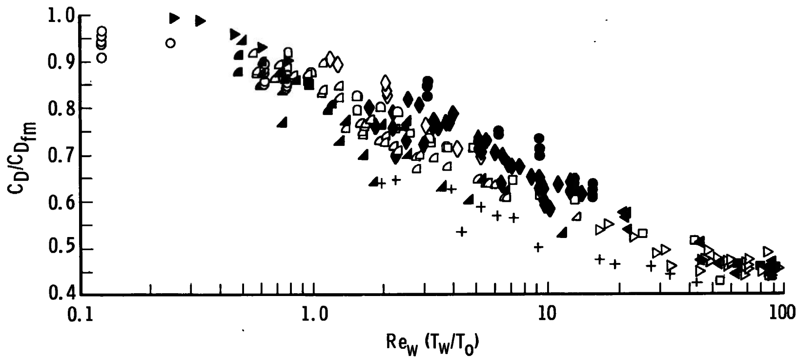
Fig. 4 Correlation with Re_w (T_w/T_o) (Related to \bar{V}_\infty^{-2} )
