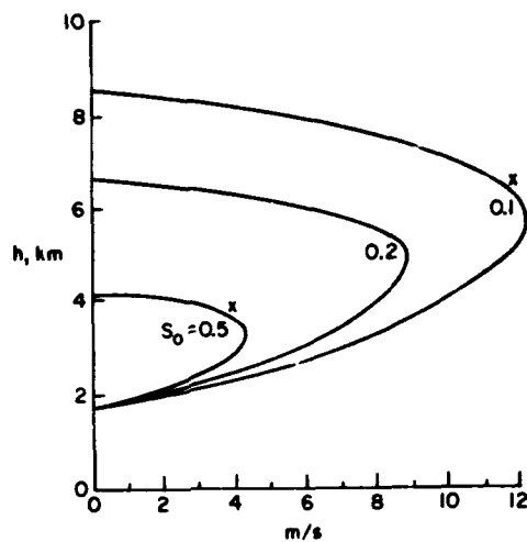
Figure 1. The Rate of Ascending Currents in Clouds vs Height on 6 June 1959, Based on the Data of Calculations. The "x" sign indicates the actual values of the maximum rate based on the data of range-finding observations
