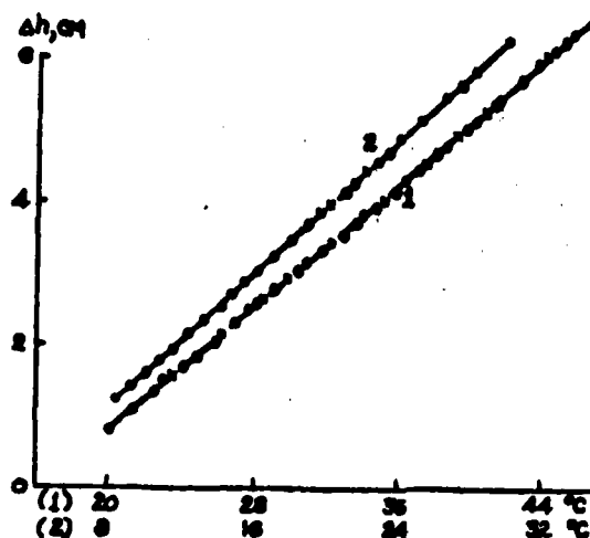
Fig. 6. Dilatometric curves for the solutions: 1) 20 mol-% cyclohexane + 80% aniline; 2) 20 mol-% methanol + 80% mesitylene; \bullet = heating; \circ = cooling; \times = repeated heating; \Delta h = height of the liquid level in the dilatometer neck.
