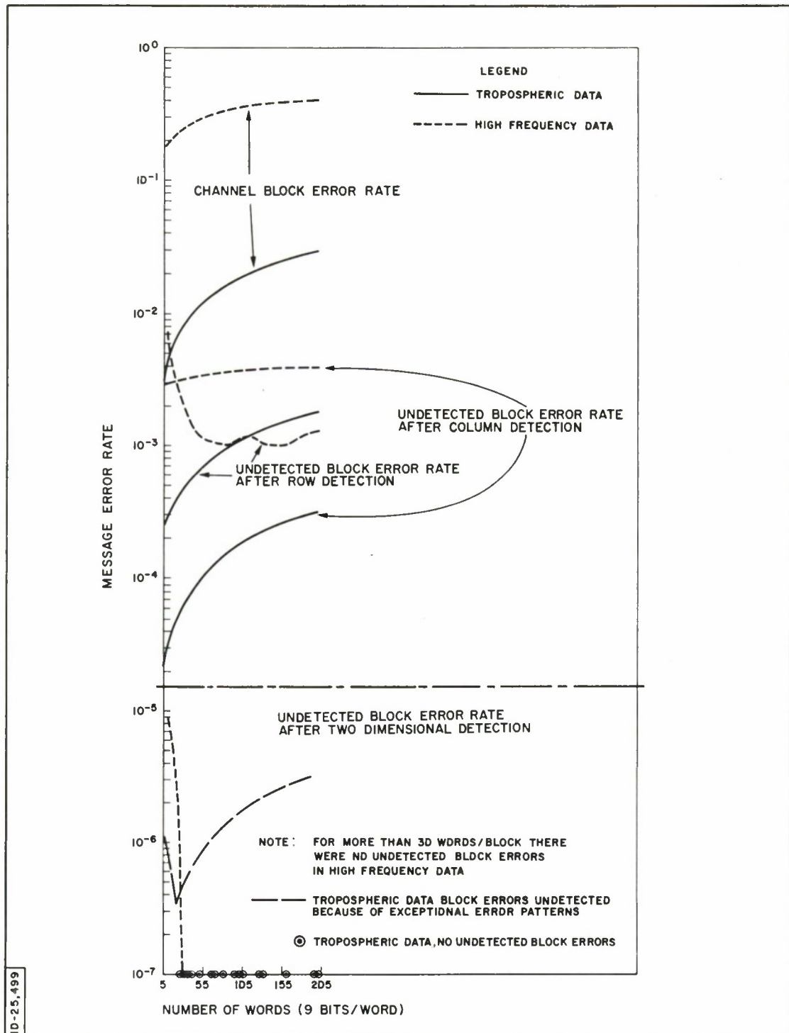
Figure 1. Performance of Two-Dimensional Parity Check Error Detection (Computer Bytes)
