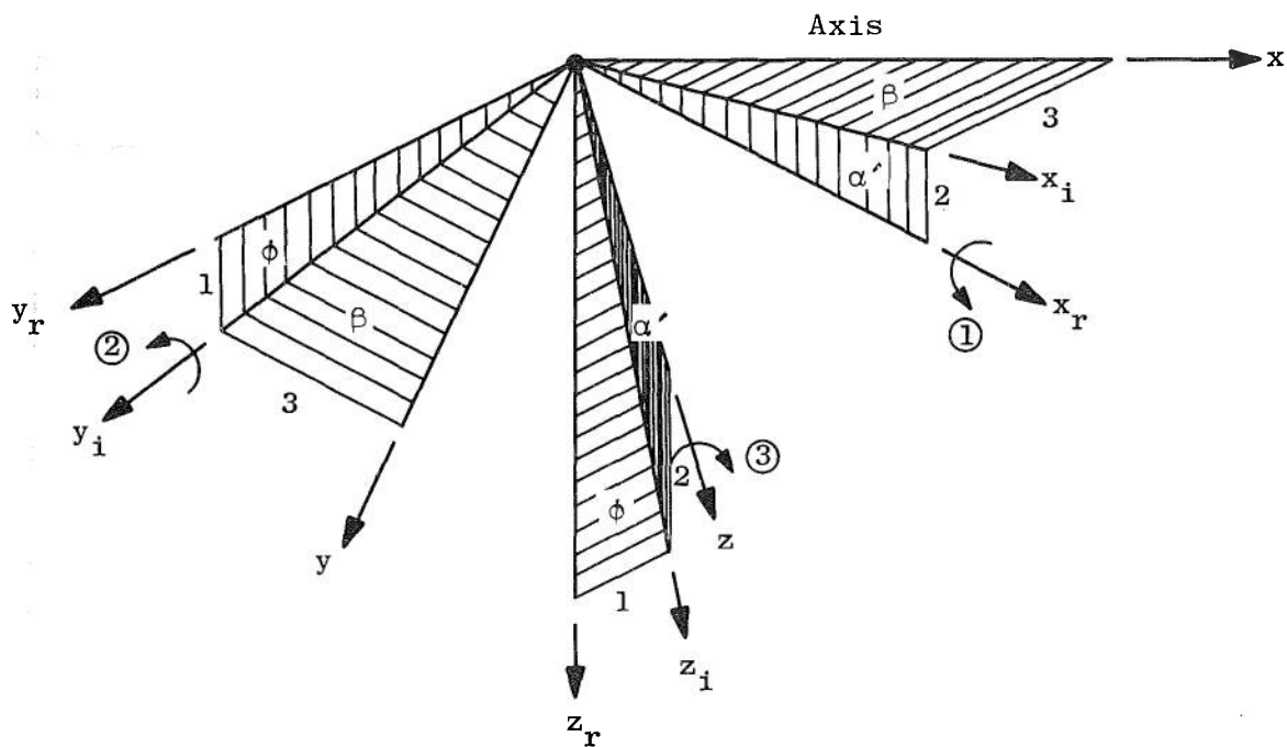
Fig. IV-6 Axis System
