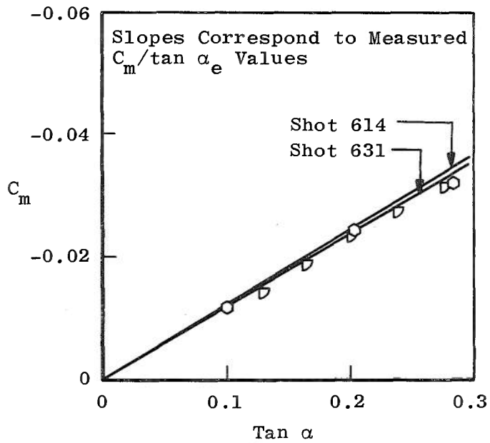
a. Pitching-Moment Coefficient
