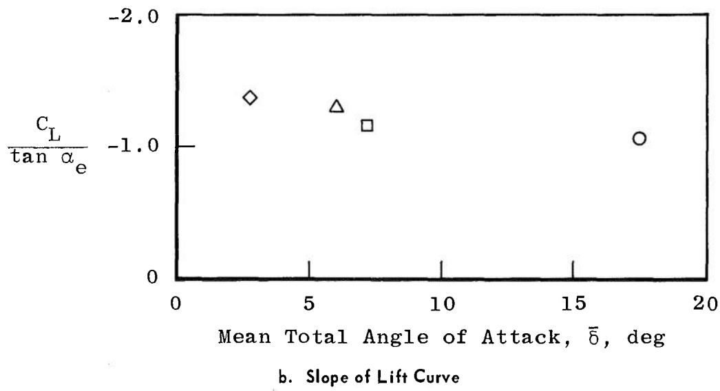
Fig. 7 Effective Static Stability Derivative and Slope of Lift Curve
