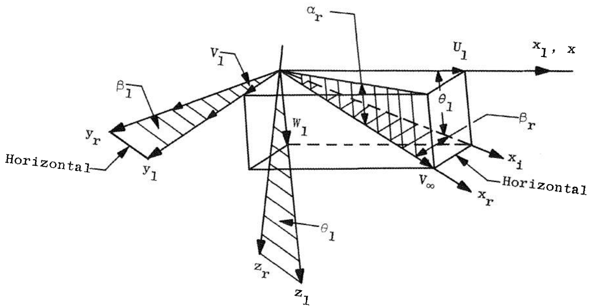
Fig. IV-7 Definition of Angles \alpha_r and \beta_r
