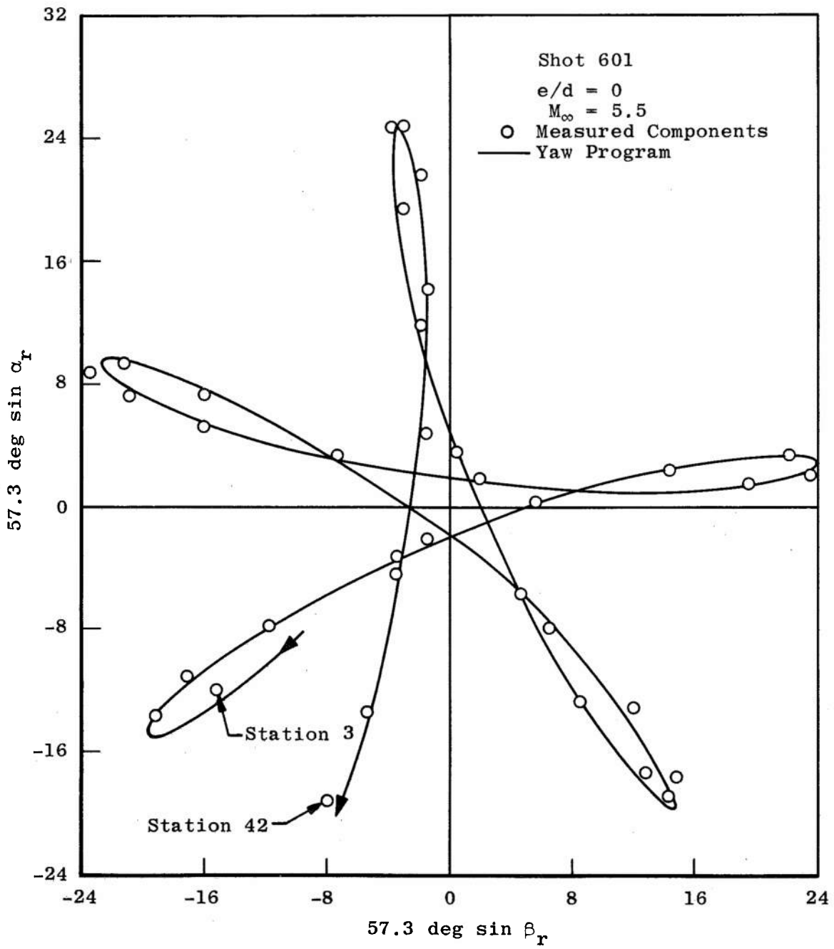
a. Symmetrical Model
