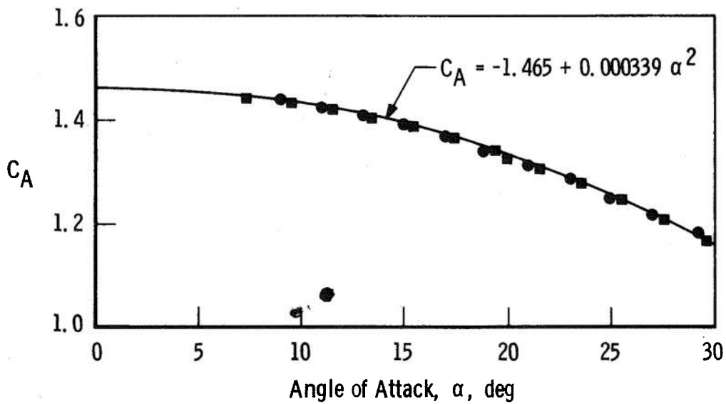
Fig. IV-3 Wind Tunnel Data for Moment and Axial Force
