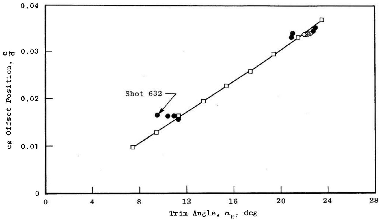
b. Second-Order Analysis Fig. 5 Concluded
