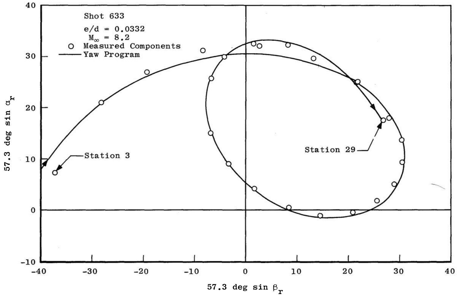
c. Full-Offset Model Fig. 4 Concluded
