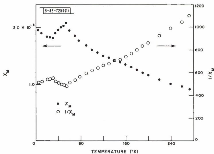
Fig. III-14. Magnetic susceptibility and reciprocal susceptibility vs temperature for high-pressure monoclinic phase of \text{CdCr}_2\text{Se}_4 .
