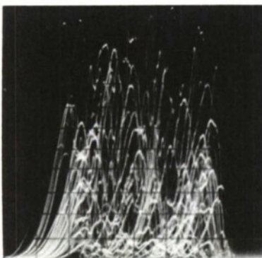
Fig. II-3. Spectrum analyzer display of beat frequency of reference laser and output of amplifier in flowing-gas operation:
