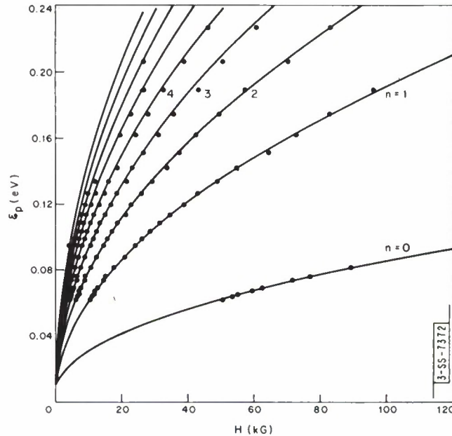
Fig. IV-1. Summary of Bi-Sb magnetoreflexion results for an 8-percent antimony alloy.
