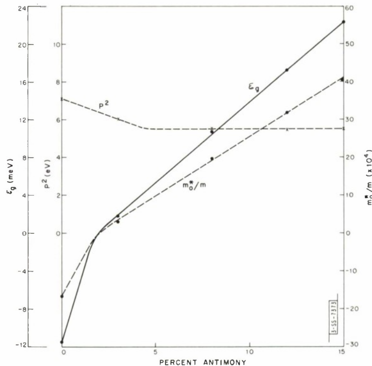
Fig. IV-2. Variation in Bi-Sb alloys of energy gap \epsilon_g (= \epsilon_{L_s} - \epsilon_{L_o}) , reduced effective mass at bottom of band m_o^* , and momentum matrix element P . T \sim 4^\circ\text{K} .
