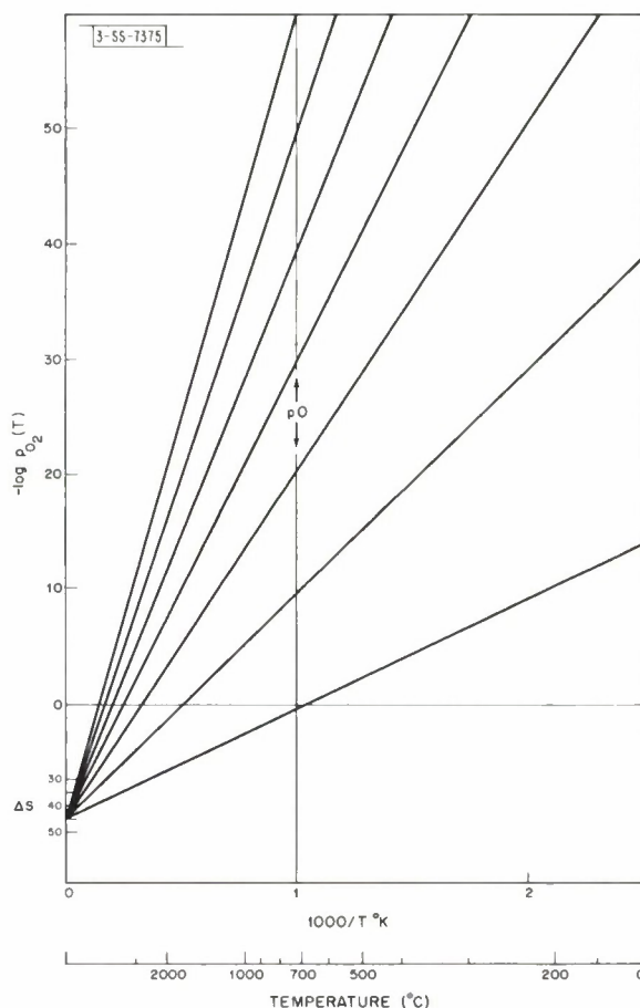
Fig. III-1. Variation of (-\log p_{O_2}) with reciprocal absolute temperature, where p_{O_2} is partial pressure of O_2 (in atmospheres) in equilibrium with a metal and its lowest oxide. For lines shown, \Delta S = 45 e.u. for reaction 2/nM + O_2 \rightarrow 2/nMO_n .
