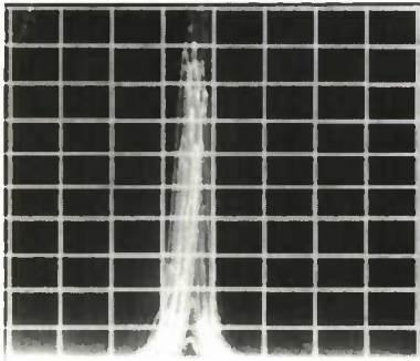
Fig. II-1. Spectrum analyzer display of beat frequency of reference laser and master oscillator with amplifier in operation:
