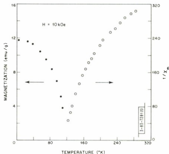
Fig. III-13. Magnetization and reciprocal magnetic susceptibility vs temperature for \text{CsNiF}_3 (6L).
