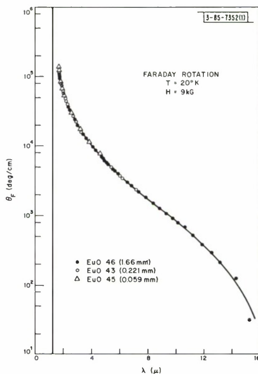
Fig. 1-6. Infrared Faraday rotation of EuO.
