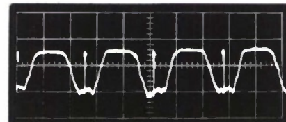
Fig. I-1. Depth of modulation produced by Ge modulator. Trace shows output of InSb detector when 2.15-mm radiation is simultaneously chopped by mechanical wheel (800 Hz) and by 2- \mu sec long 1.5-A pulses in Ge modulator.
