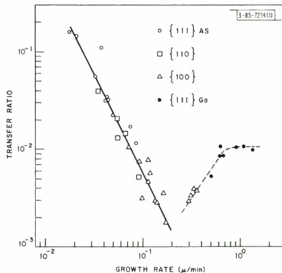
Fig. I-3. Growth rate dependence of tin transfer ratio for \{111\} As, \{110\} , \{100\} , and \{111\} Ga planes.
