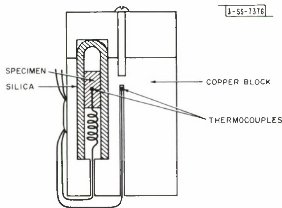
Fig. III-7. Sample holder for DTA measurements at low temperatures.
