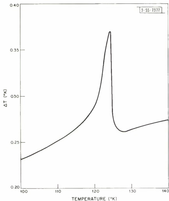
Fig. III-8. DTA curve for magnetic transition in \text{CoS}_2 (Curie temperature of 124^\circ\text{K} ).
