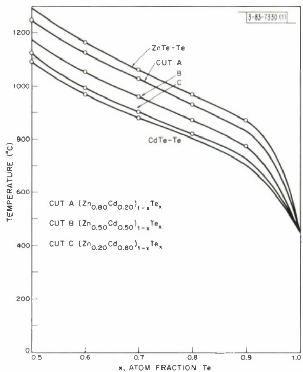
Fig. III-4. Liquidus curves for Te-rich compositions in Zn-Cd-Te system.
