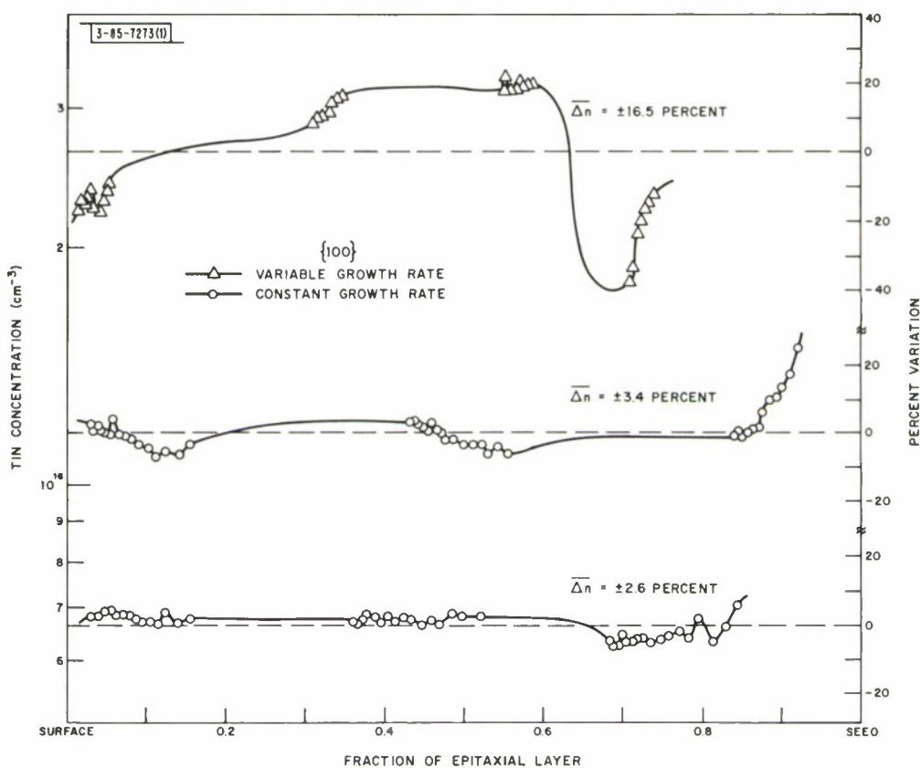
Fig. 1-4. Doping variations parallel to growth axis for {100} epitaxial layers grown on low-resistance substrates. Vertical scale has been amplified to indicate small variations in doping. Upper profile corresponds to layer grown under conditions where small variations of temperature and flow will vary growth rate and thus doping; lower two profiles were grown under conditions where growth rate is insensitive to variations in temperature and flow.
