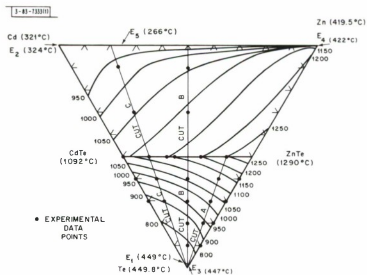
Fig. III-5. Liquidus isotherms for Zn-Cd-Te system.
