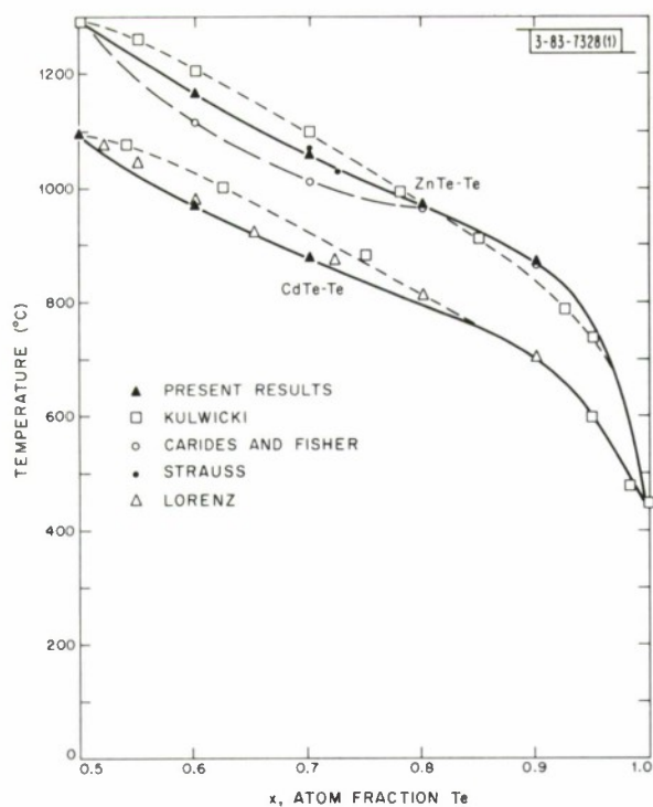
Fig. III-3. Liquidus curves for ZnTe-Te and CdTe-Te systems.
