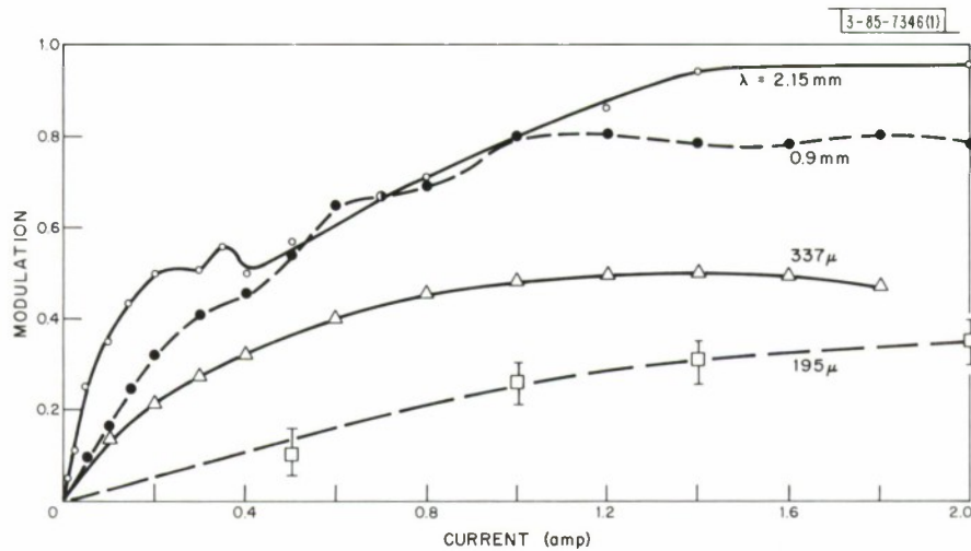
Fig. 1-2. Modulation index as a function of current in 1.3-mm thick p-type Ge ( N_A - N_D = 1.3 \times 10^{15} \text{ cm}^{-3} ).
