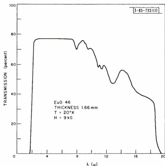
Fig. 1-5. Infrared transmission of EuO.
