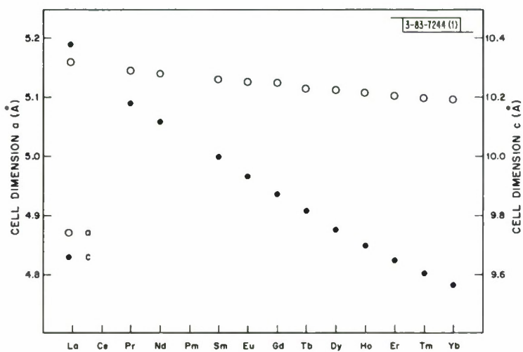
Fig. III-11. Cell dimensions a and c for \text{LnCrTeO}_6 compounds.
