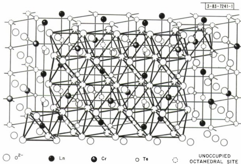
Fig. III-10. Crystal structure of \text{LnCrTeO}_6 .
