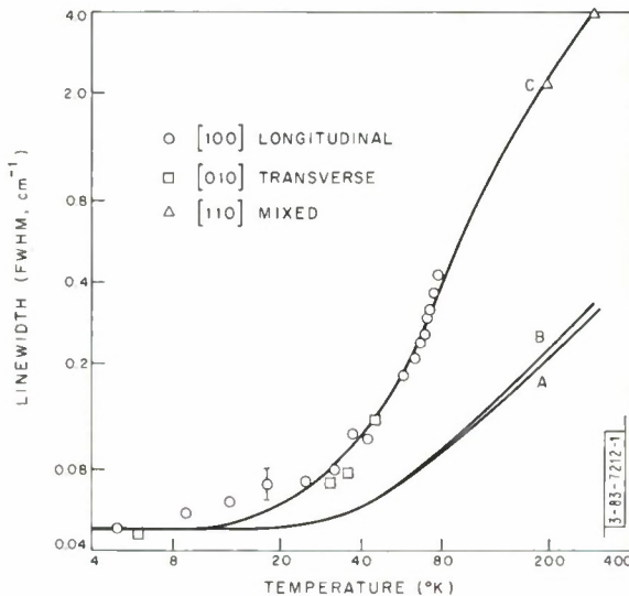
Fig. IV-3. Linewidth of 128\text{-cm}^{-1} E-mode in \alpha -quartz as function of temperature. Points are experimental, and curves are theoretical. Curve A: decay into two sharp acoustic modes only; curve B: decay into two relaxation broadened acoustic modes only; curve C: decay into acoustic modes and scattering of thermal phonons.
