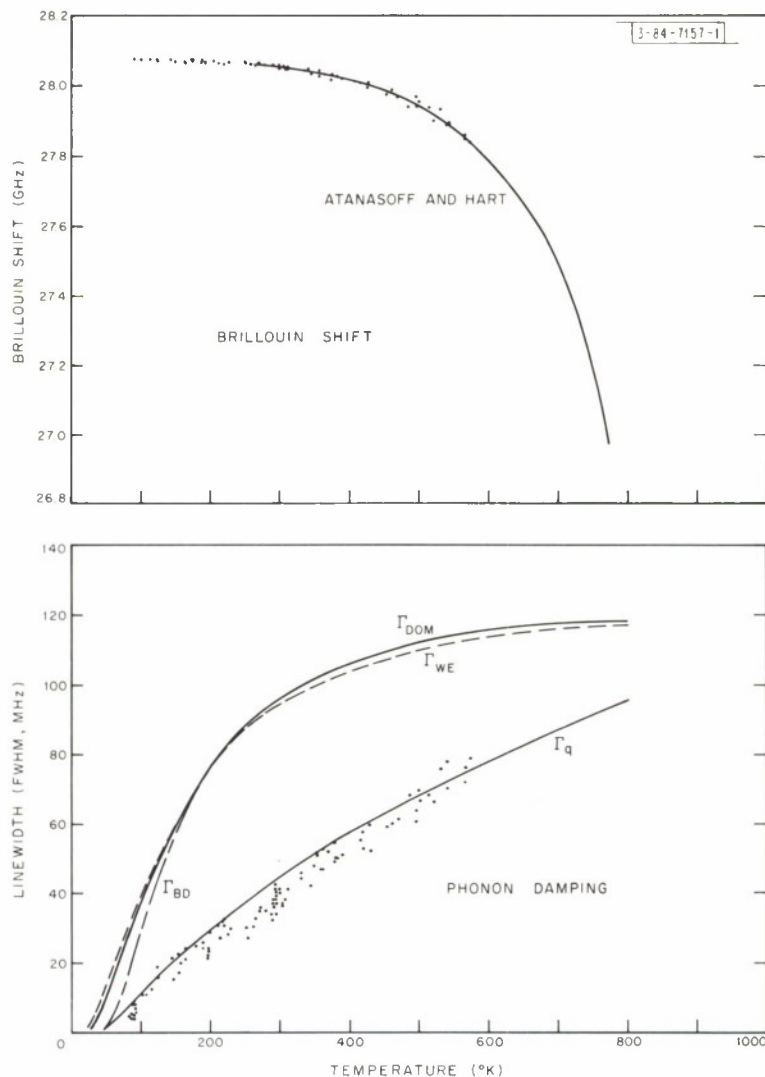
Fig. IV-4. Shift and width of 28-GHz longitudinal acoustic phonons along x-axis of \alpha -quartz. Points are experimental, and curves are theoretical. \Gamma_{DOM} , \Gamma_{WE} , and \Gamma_{BD} represent various single-relaxation time theories, and \Gamma_q represents a distributed relaxation process.
