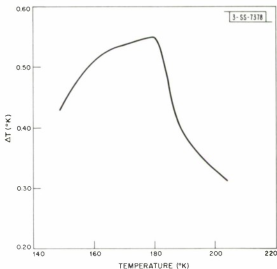
Fig. III-9. DTA curve for cubic-rhombohedral transformation in \text{Sn}_{0.8}\text{Ge}_{0.2}\text{Te} at 180^\circ\text{K} .
