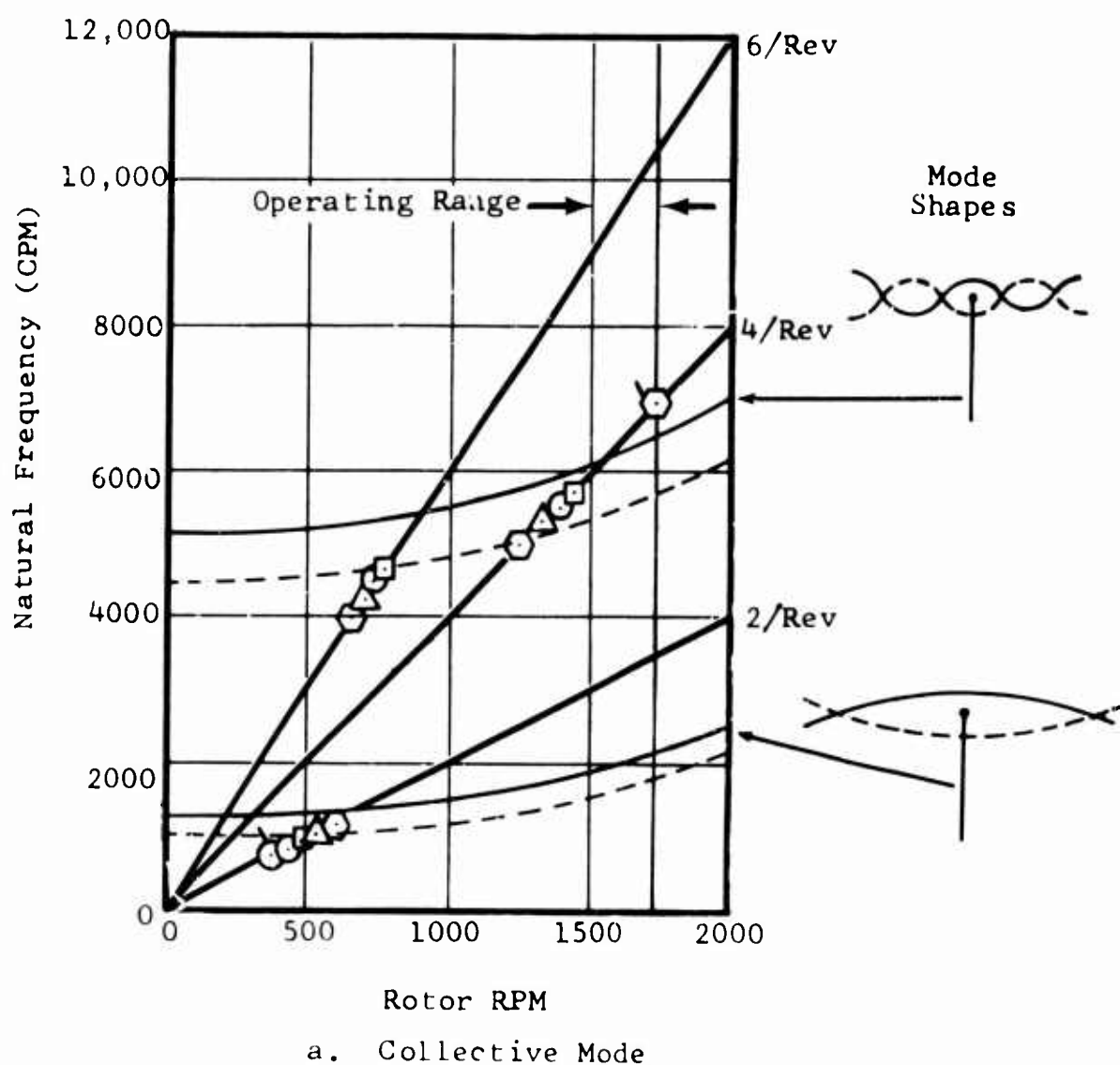
Figure 15. Coupled Rotor Natural Frequencies for the Radial Plus 45-Degree Thrust Bearing Tail Rotor Configuration.
