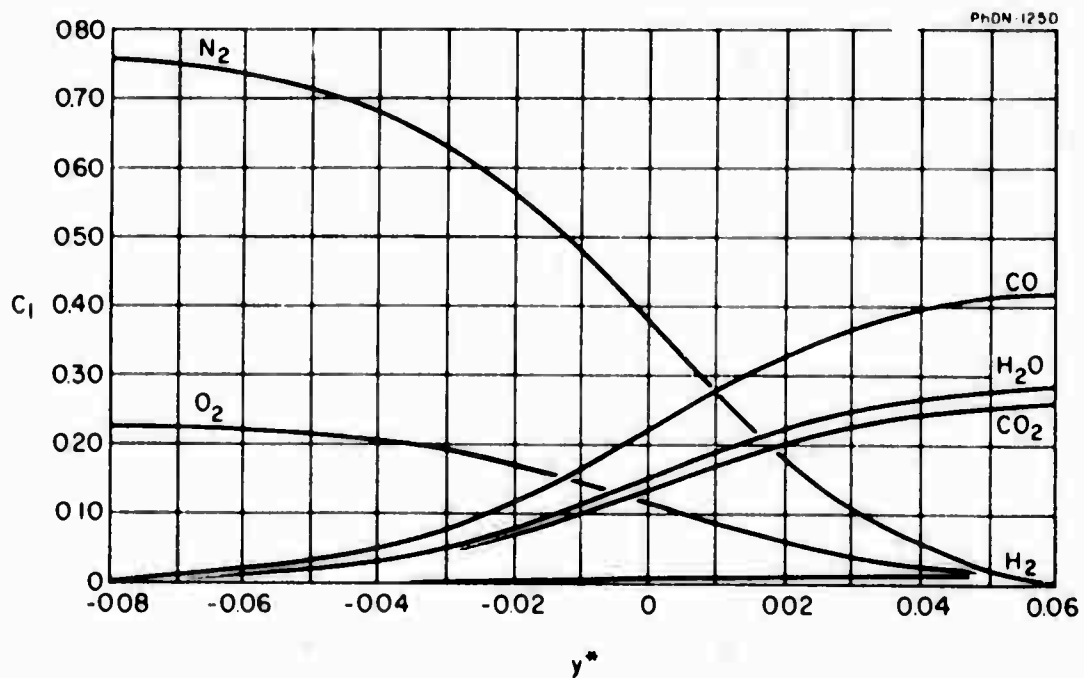
FIGURE 6d CONCENTRATION PROFILES DURING THE INITIAL STAGES OF DEVELOPMENT OF THE MIXING LAYER, x^* = 1.125
