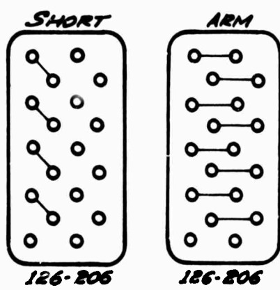
FIGURE 28 ELECTRICAL SCHEMATIC (309-28) THREE EVENT PROGRAMMER
