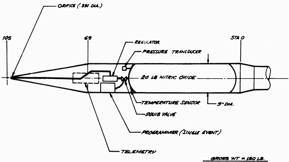
FIGURE 1 NITRIC OXIDE PAYLOAD 277-11
