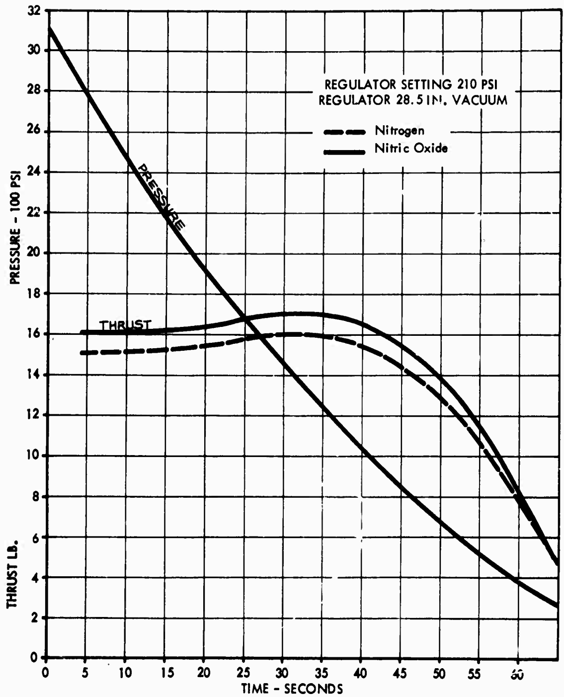
FIGURE 8 - PRESSURE & THRUST VS. TIME - FLIGHT NO. 1
