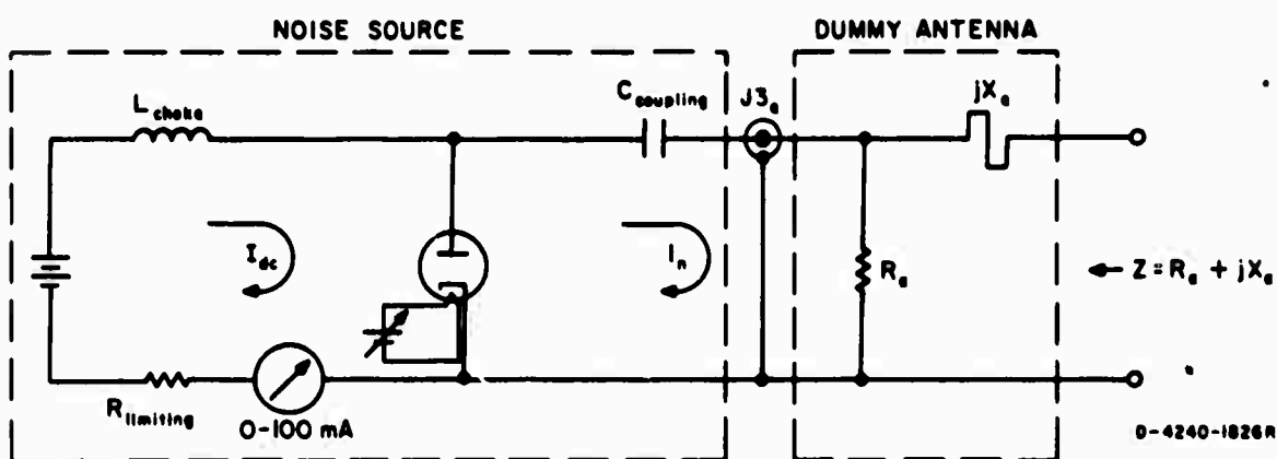
FIG. A-1 SIMPLIFIED SCHEMATIC OF DIODE NOISE SOURCE
