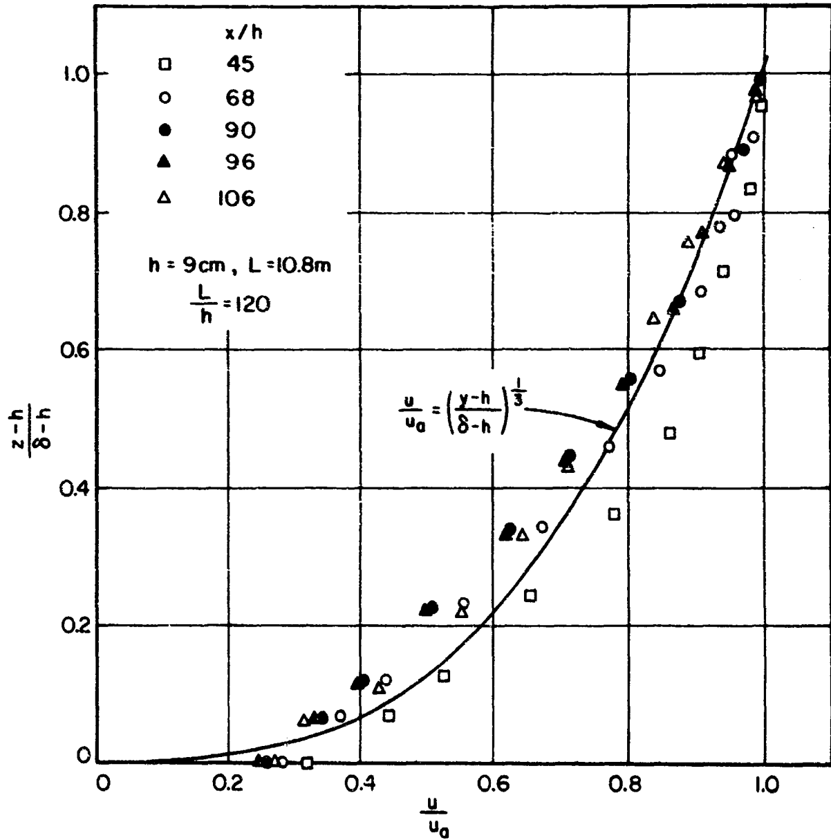
Canopy Study: Flow Above Canopy Pegs \phi 0.48, Spaced 2.54 x 2.54cm
