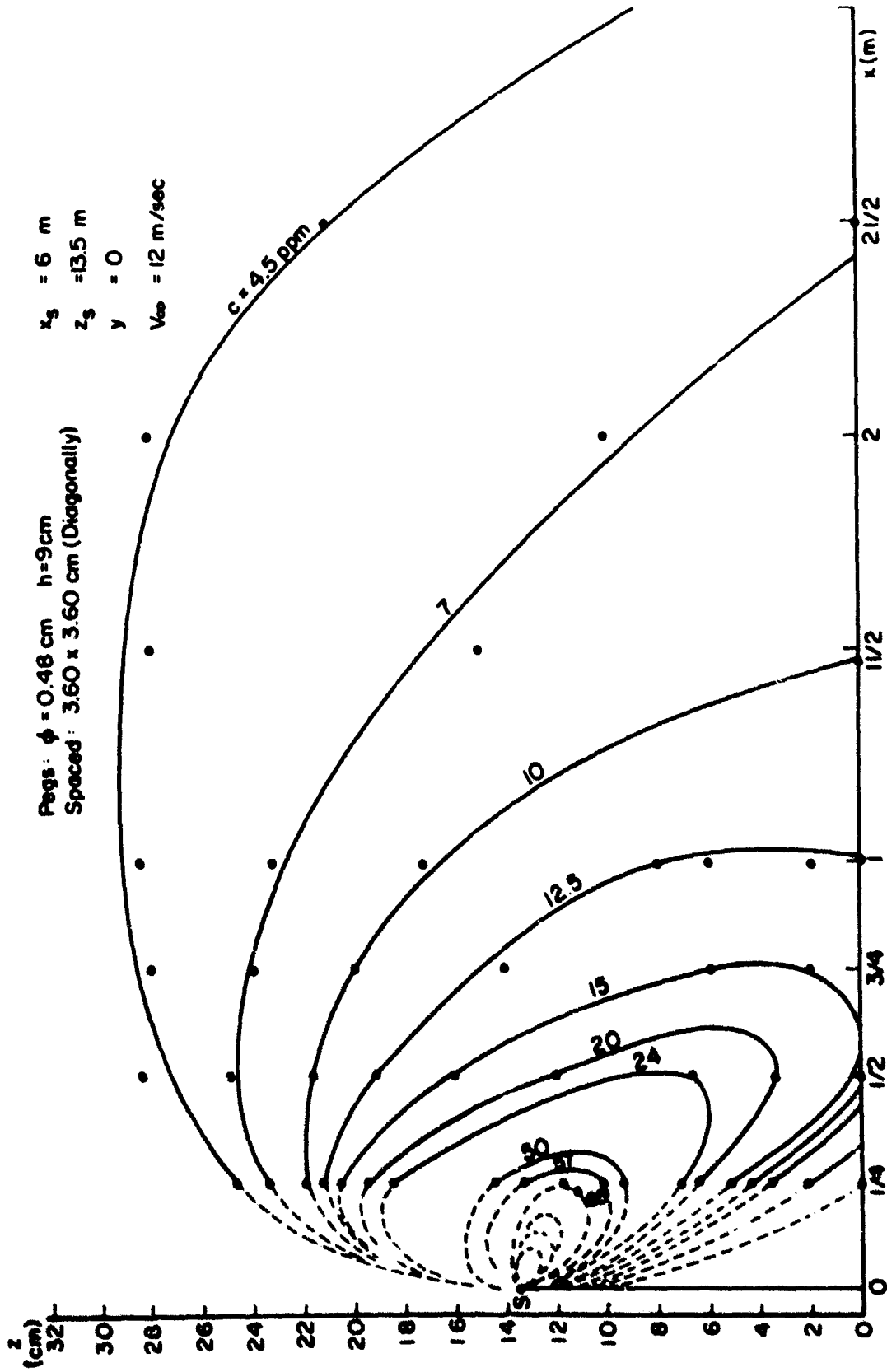
Fig. 36. Diffusion in the canopy-isoconcentration lines ( 2.54 \times 2.54 diagonal). x_s = 6 , z_s = 1.5 \text{ h}
