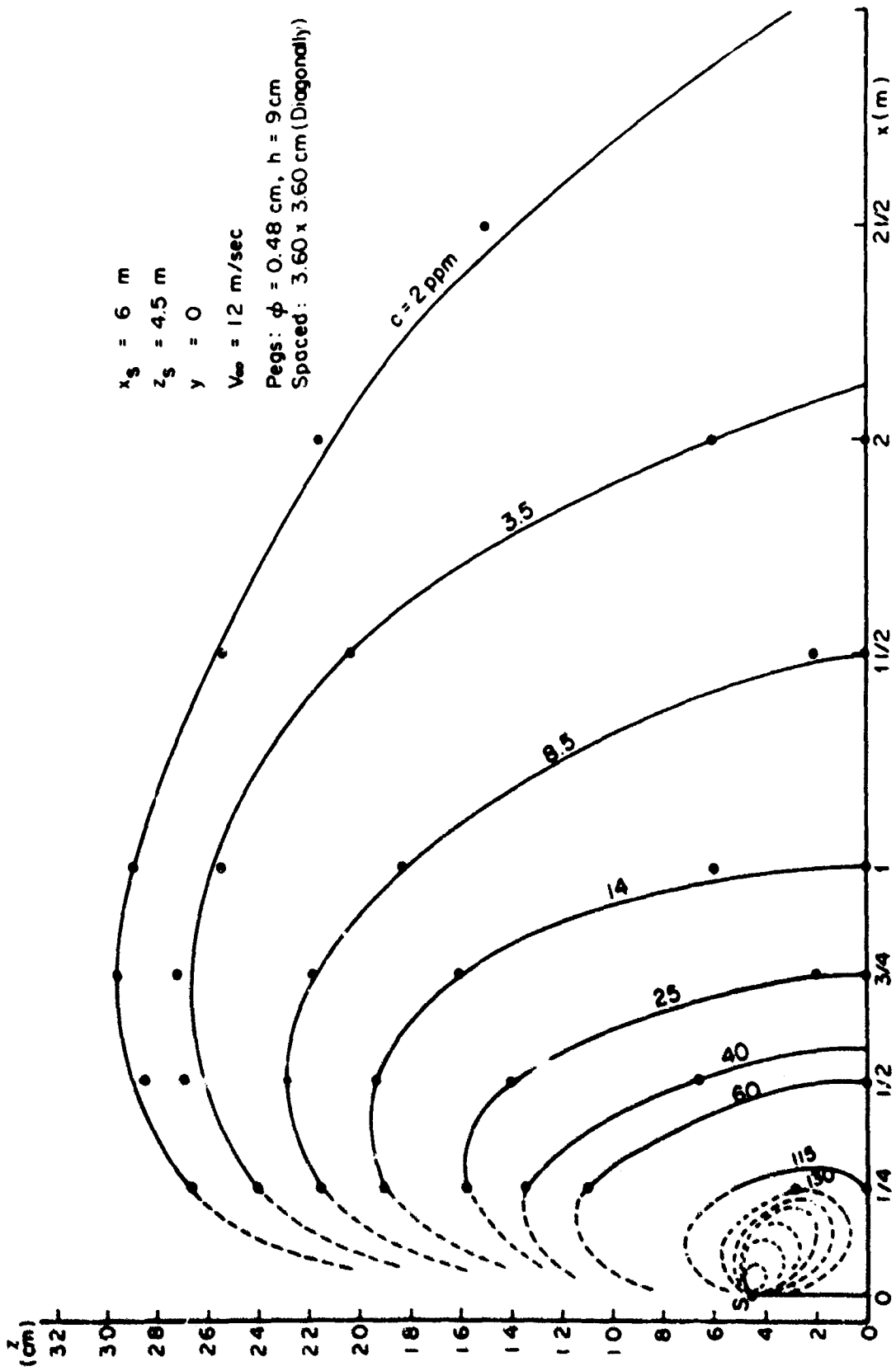
Fig. 34. Diffusion in the canopy-isoconcentration lines (2.54 x 2.54 diagonal). x_s = 6 , z_s = 0.5
