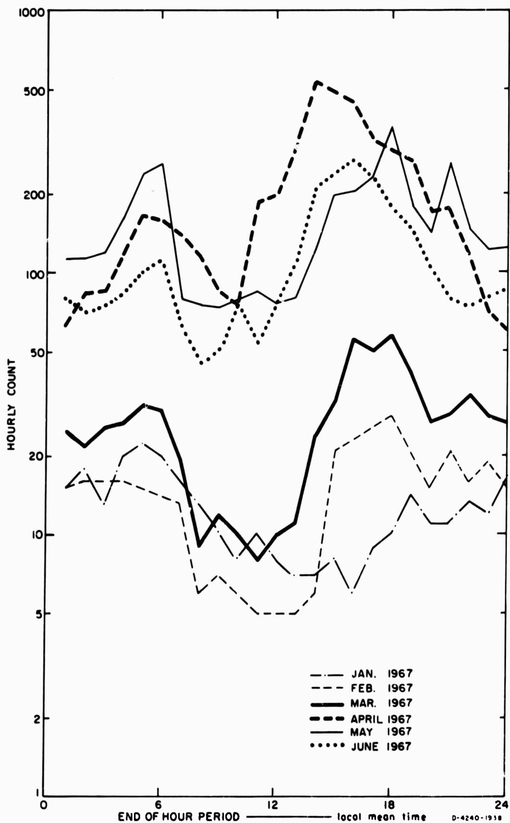
FIG. 16 DIURNAL VARIATION OF CCIR-1 DATA — JANUARY TO JUNE
