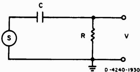
FIG. C-2 EQUIVALENT ANTENNA CIRCUIT (Generalized)
