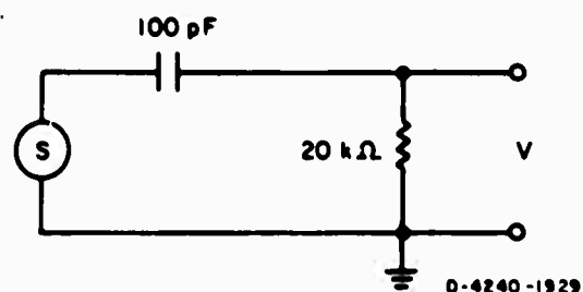
FIG. C-1 EQUIVALENT ANTENNA CIRCUIT (Actual Values)
