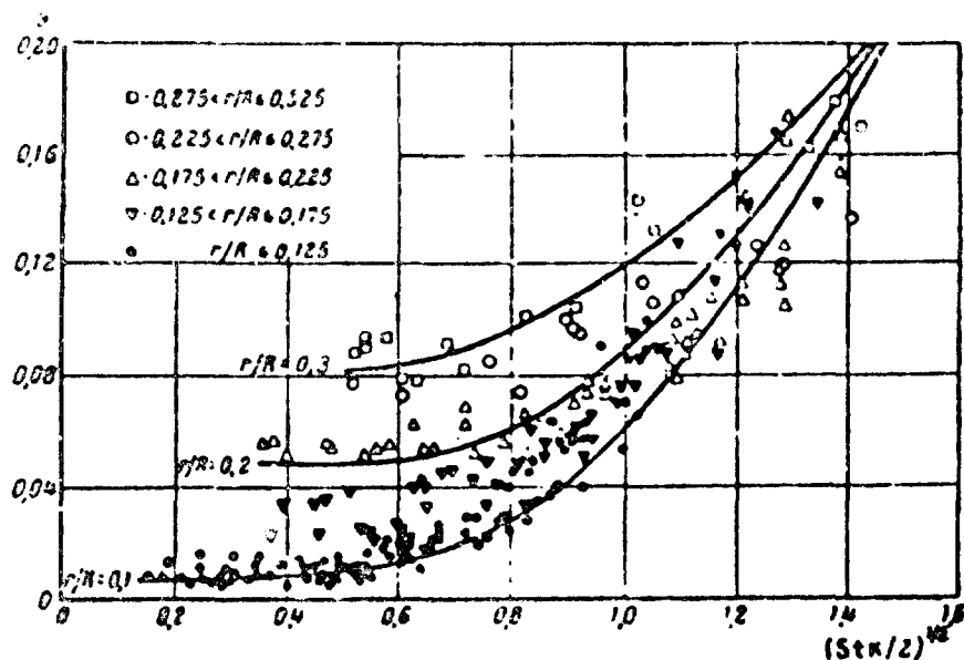
Fig. 38. Dependence of effectiveness of filters made of glass fibers on St\kappa and r/R .
