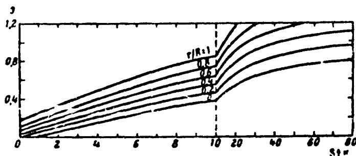
Fig. 26. Inertial precipitation on a cylinder at Re_f = 0.2 .
