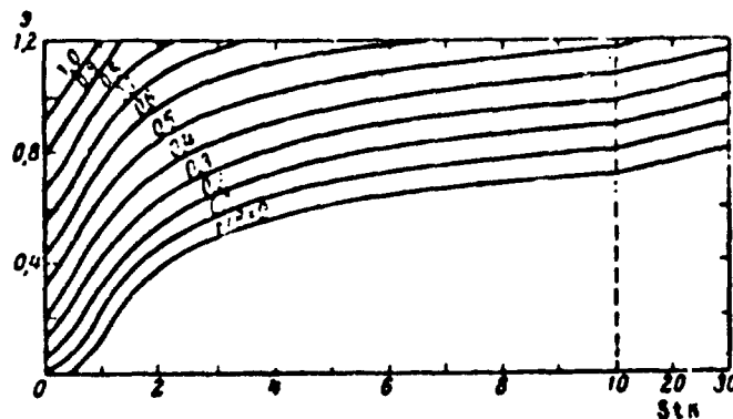
Fig. 25. Inertial precipitation on cylinder at Re_f = 10 .
