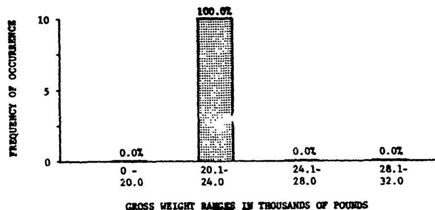
Figure 50. Gross Weight Versus Frequency of Occurrence at 50- to 60-Percent Torque Split (10 Sample Points, Table I Data).
