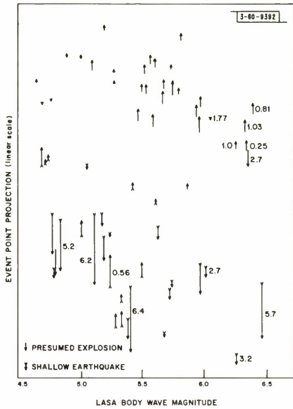
Fig. 1-10. Use of multivariate discriminant algorithm to separate presumed explosions and earthquakes. Far arrow representing each event, tail shows result of using two frequency domain variables (signal amplitude over 0.35- to 0.85-Hz and 1.45- to 1.95-Hz bands) and head shows result of adding to these two a single time-domain measurement (complexity).
