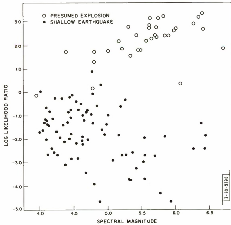
Fig. 1-8. Comparison of two short-period spectral discriminants: (a) "spectral difference" (roughly equivalent to old spectral ratio criterion), and (b) "log likelihood ratio."
