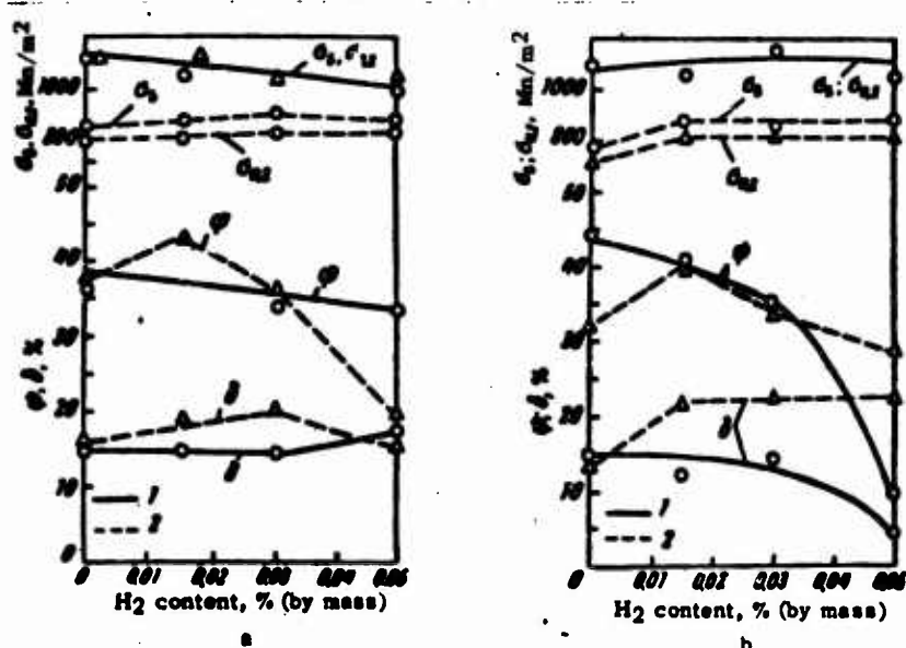
Fig. 16. Influence of hydrogen on the mechanical properties of the \alpha -titanium alloy VT5-1 after quenching (a) and after cooling with the furnace (b) in tests with various deformation rates in mm/min: 1) 20; 2) 0.4.
