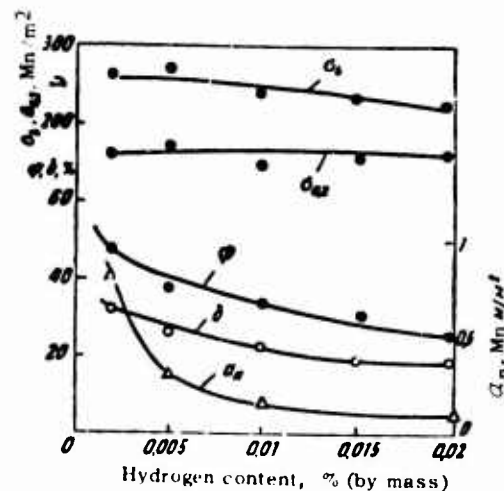
Fig. 80. Influence of hydrogen on the mechanical properties of domestic zirconium.
