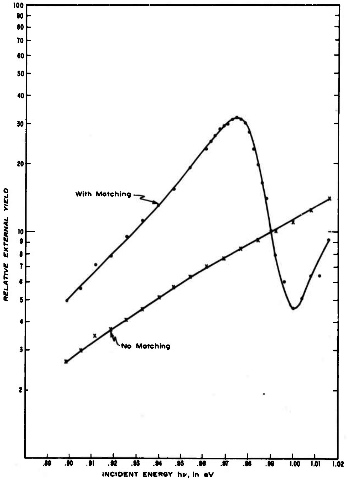
FIGURE II-33: Measured yield of a 0.051 in. diameter diode using a 0.036 in. diameter mask both with and without the \text{CaF}_2 -Au matching layers.
