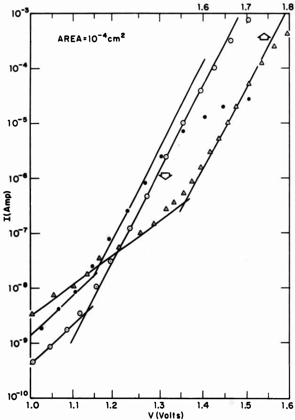
FIGURE III-9: I-V characteristic of ZnS-Ag diodes. \Delta - diode a, \odot - diode b, \bullet - diode b after heating 23.5 hrs. at 251°C. Use upper margin voltage scale for diode a, lower for diode b.
