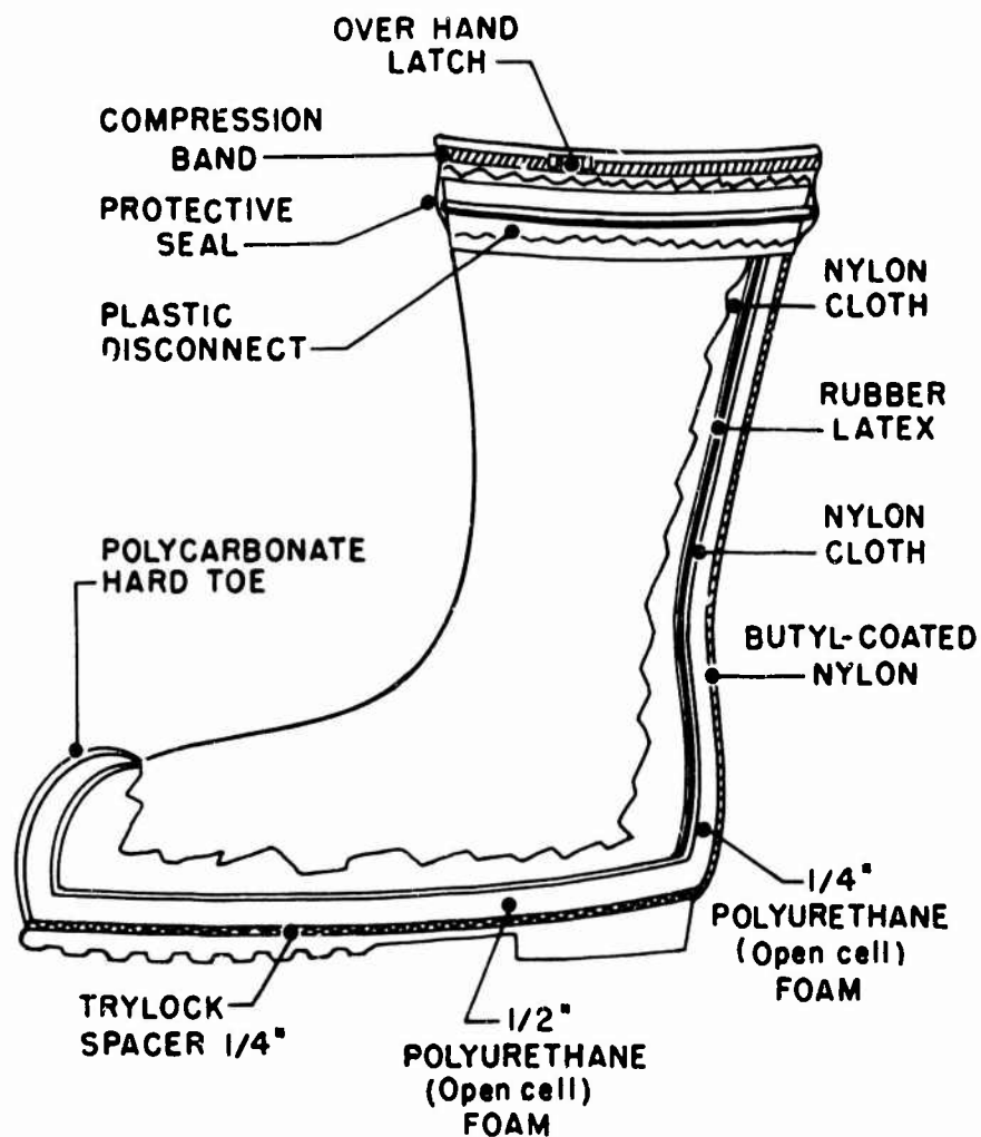
Figure 10. Boot Design Configuration
