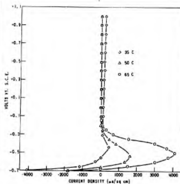
Figure 14. EFFECT OF TEMPERATURE ON POLARIZATION OF Ti-13V-11Cr-3Al IN 20% HCl
