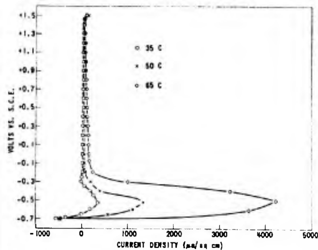
Figure 16. EFFECT OF TEMPERATURE ON POLARIZATION OF Ti-6Al-4V IN 20% HCl
