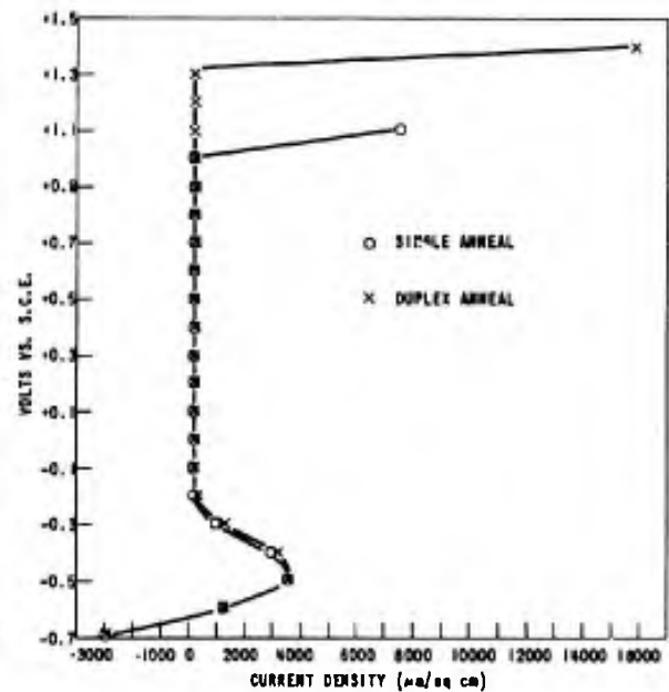
Figure 12. EFFECT OF HEAT TREATMENT ON POLARIZATION OF Ti-8Al-1Mo-1V (LONGITUDINAL) IN 20% HCl AT 65 C
