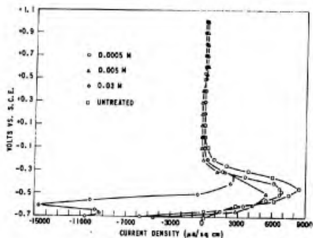
Figure 5. EFFECT OF \text{CuSO}_4 CONCENTRATION ON POLARIZATION OF Ti-6Al-6V-2Sn (180 KSI) IN 20% HCl AT 65 C
