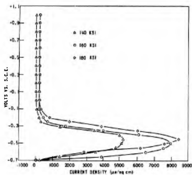
Figure 3. EFFECT OF STRENGTH LEVEL ON POLARIZATION OF Ti-6Al-6V-2Sn IN 20% HCl AT 65 C
