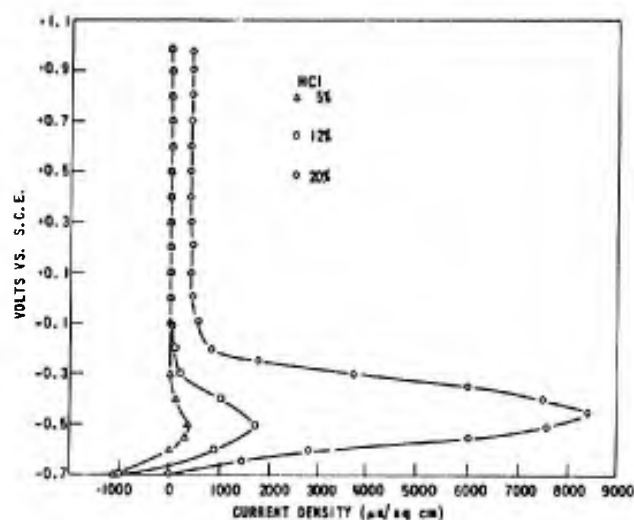
Figure 1. EFFECT OF CONCENTRATION OF HCl ON POLARIZATION OF Ti-6Al-6V-2Sn (180 KSI) AT 65 C
