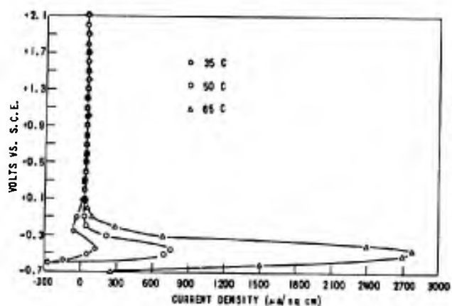
Figure 7. EFFECT OF TEMPERATURE ON POLARIZATION OF COMMERCIAL PURE Ti-75A IN 20% HCl
