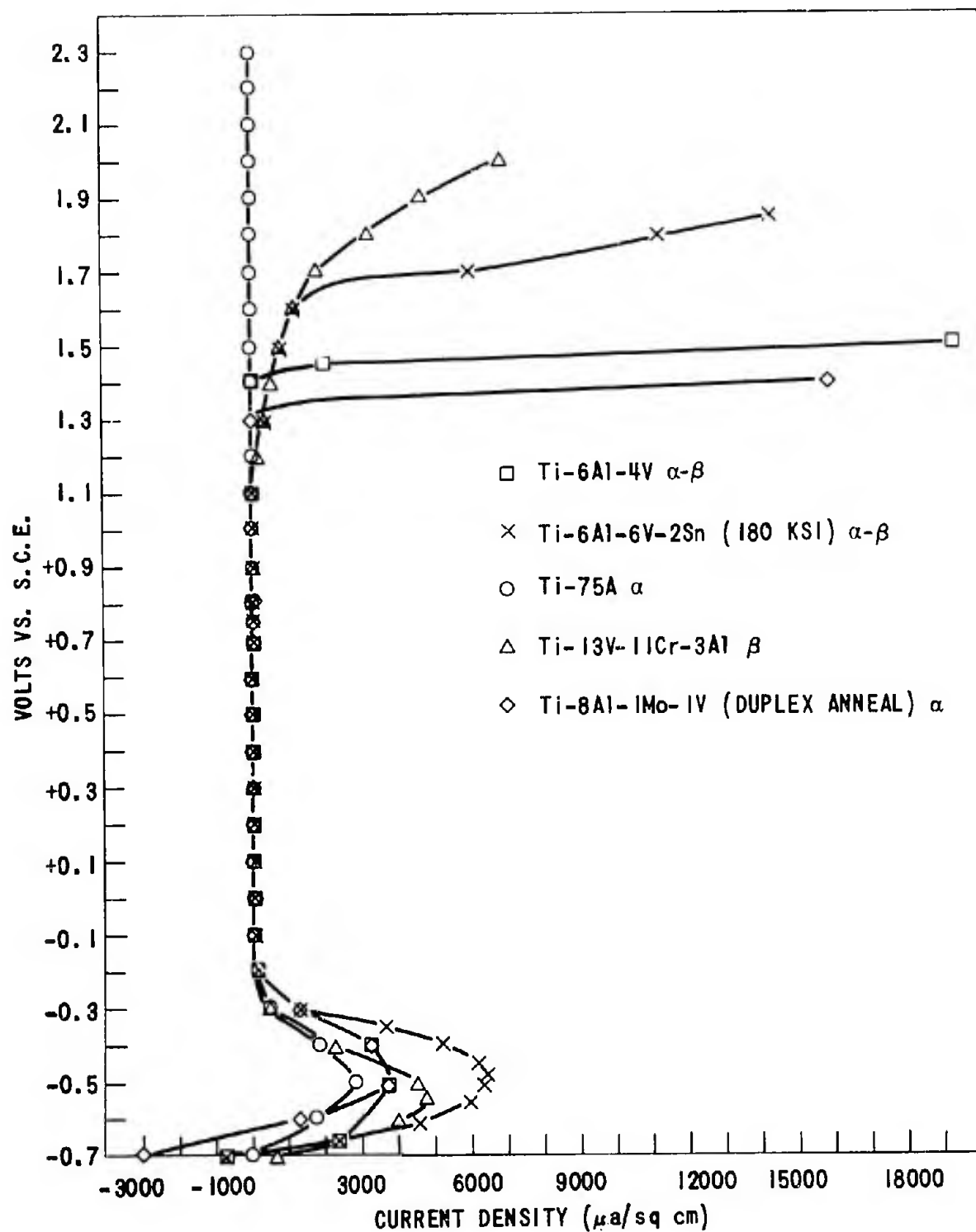
Figure 17. COMPARISON OF POLARIZATION BEHAVIOR OF TITANIUM AND ALLOYS IN 20% HCl AT 65 C
