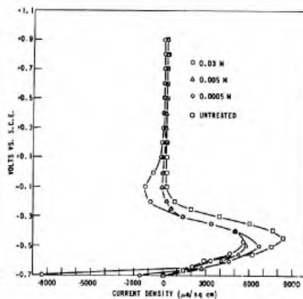
Figure 4. EFFECT OF \text{FeCl}_3 CONCENTRATION ON POLARIZATION OF Ti-6Al-6V-2Sn (180 KSI) IN 20% HCl AT 65 C
