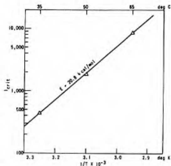
Figure 2. ARRHENIUS PLOT FOR Ti-6Al-6V-2Sn (180 KSI) IN 20% HCl
