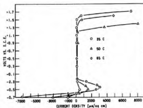
Figure 10. EFFECT OF TEMPERATURE ON POLARIZATION OF Ti-8Al-1Mo-1V (SINGLE ANNEAL, TRANSVERSE) IN 20% HCl
