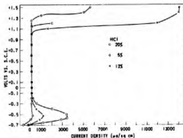
Figure 9. EFFECT OF CONCENTRATION OF HCl ON POLARIZATION OF Ti-8Al-1Mo-1V (DUPLEX ANNEALED) AT 65 C
