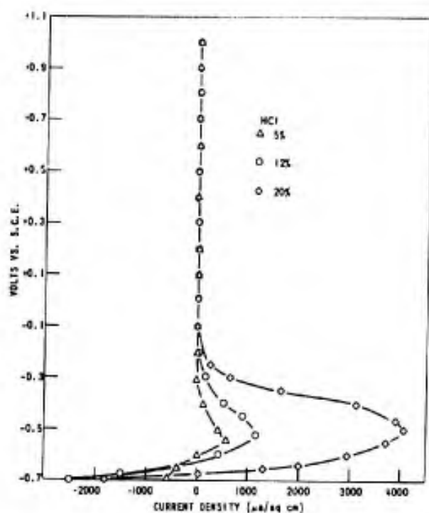
Figure 13. EFFECT OF HCl CONCENTRATION ON POLARIZATION OF Ti-13V-11Cr-3Al AT 65 C
