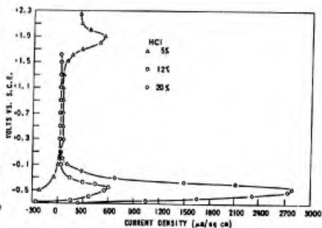
Figure 6. EFFECT OF HCl CONCENTRATION ON POLARIZATION OF COMMERCIAL PURE Ti-75A AT 65 C
