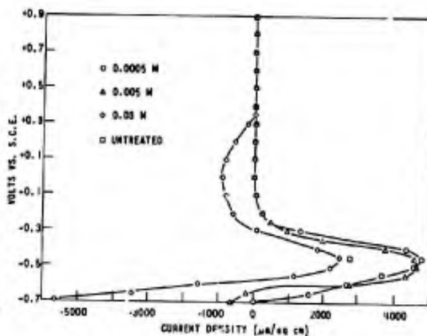
Figure 8. EFFECT OF \text{FeCl}_3 CONCENTRATION ON POLARIZATION OF COMMERCIAL PURE Ti-75A IN 20% HCl AT 65 C
