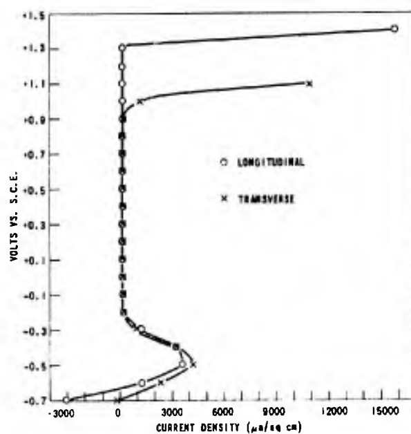
Figure 11. EFFECT OF DIRECTIONALITY ON POLARIZATION OF Ti-8Al-1Mo-1V (DUPLEX ANNEAL) IN 20% HCl AT 65 C
