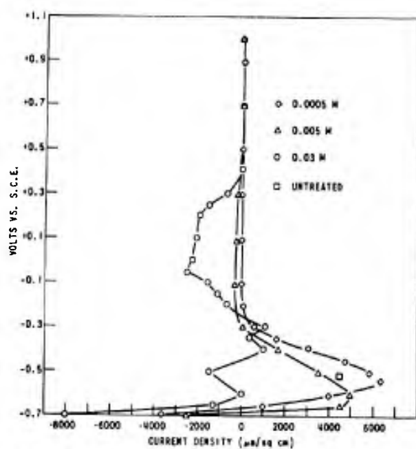
Figure 15. EFFECT OF \text{CuSO}_4 CONCENTRATION ON POLARIZATION OF Ti-13V-11Cr-3Al AT 65 C
