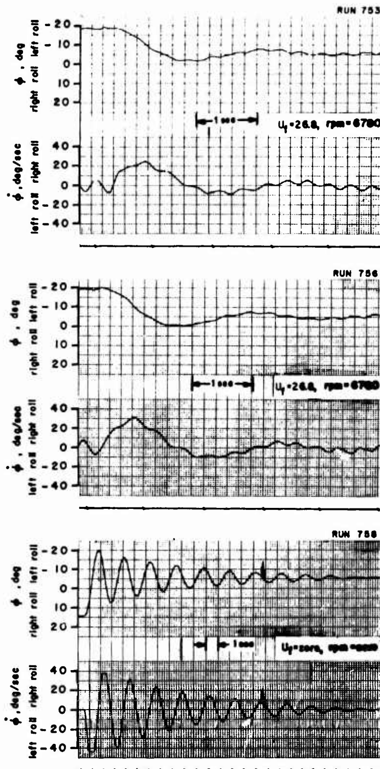
Figure 20. Lateral Transient Response. One Degree of Freedom, \phi . i_d = 60^\circ , \beta_{75R} = 26.4^\circ , \Delta\beta_0 = 2.5^\circ , Small Vertical Tail, Spring Restrained.
