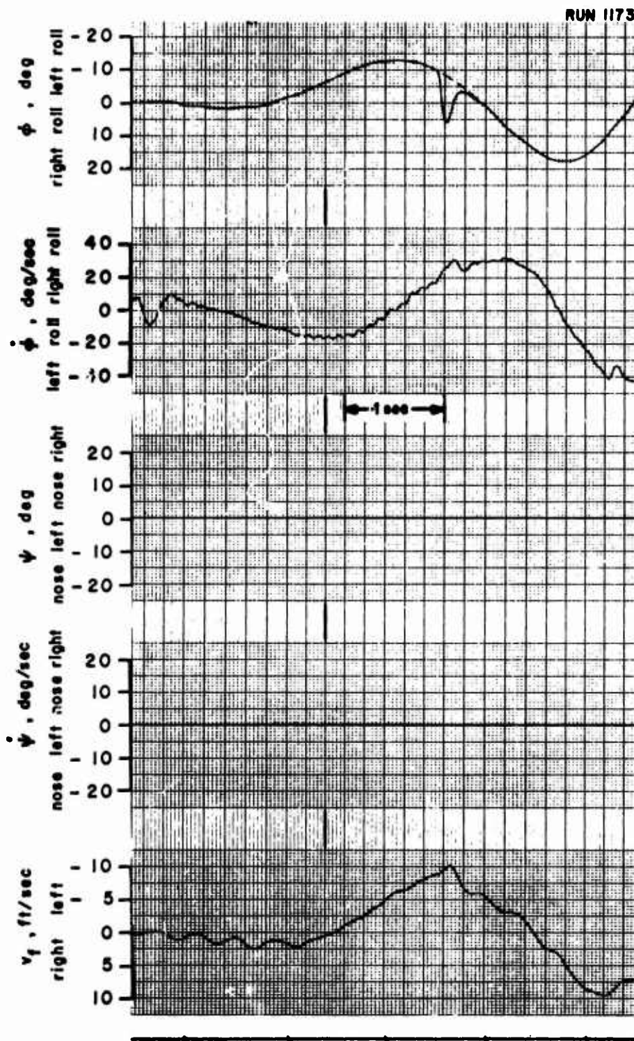
Figure 23. Lateral/Directional Transient Response. Two Degrees of Freedom, \phi - v_l . i_d = 60^\circ , U_{of} = 29 ft/sec, \beta_{.75R} = 25.5^\circ , rpm = 6780, \Delta\beta_o = 3.0^\circ , Large Vertical Tail.
