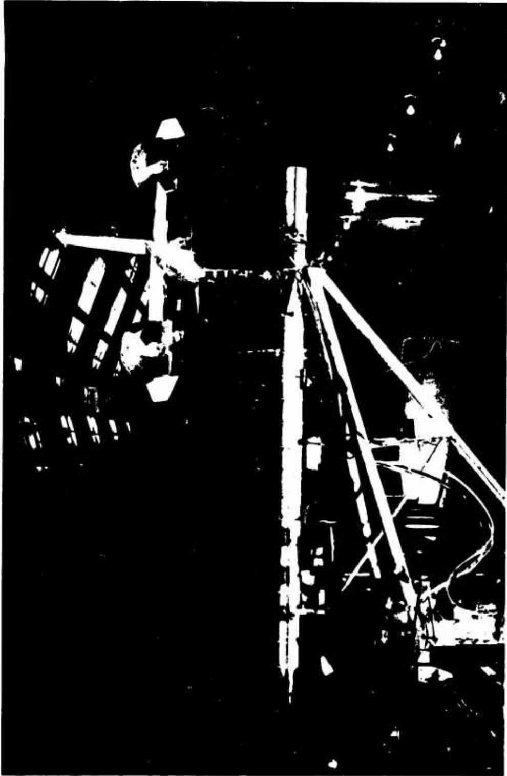
Figure 1. Princeton Dynamic Model Track, Showing Model Mounted on Lateral/Directional Dynamic Testing Apparatus.
