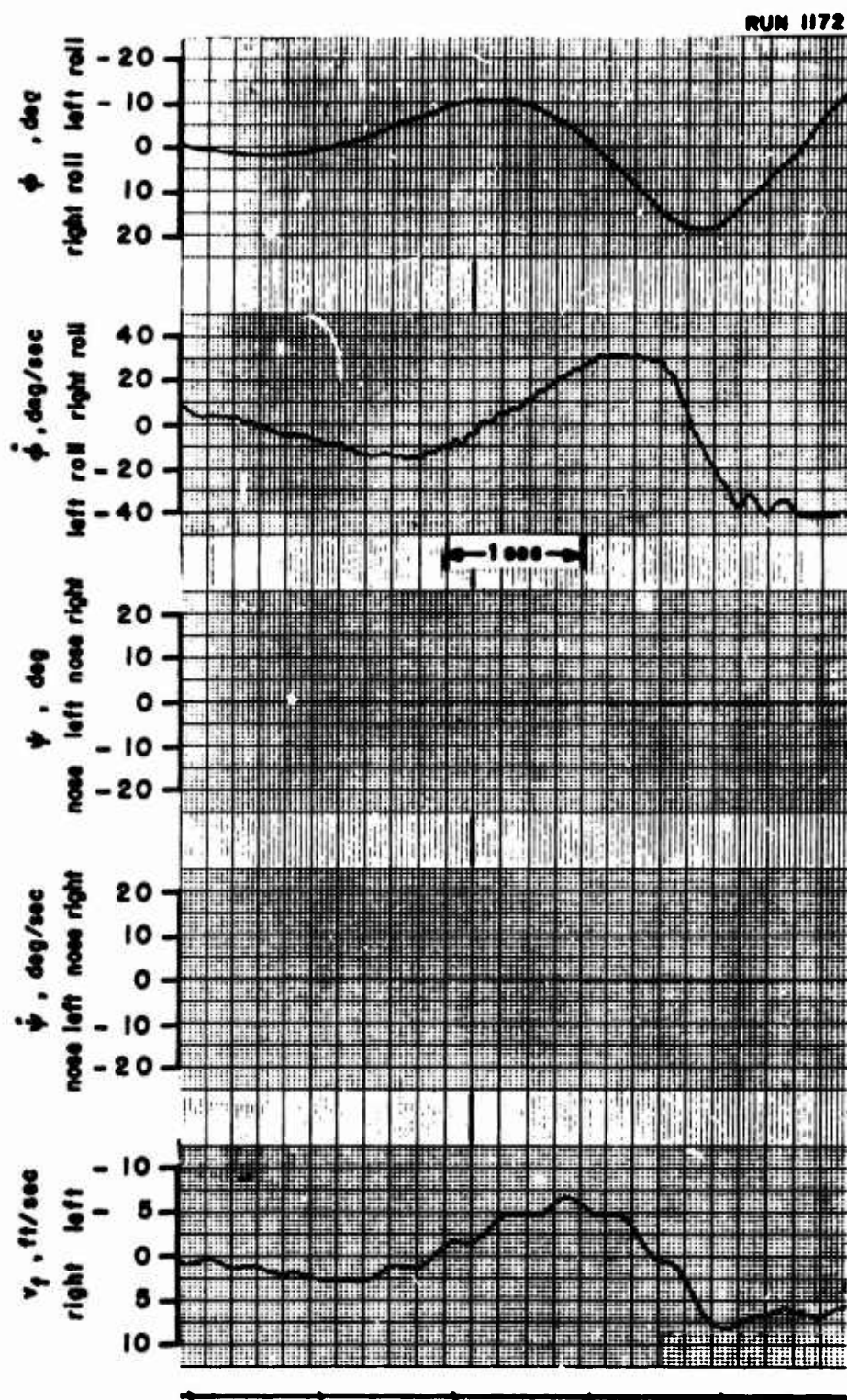
Figure 23. Lateral/Directional Transient Response. Two Degrees of Freedom, \phi - v_y . i_d = 60^\circ , U_{O_f} = 29 ft/sec, \beta_{.75R} = 25.5^\circ , rpm = 6780, \Delta\beta_0 = 3.0^\circ , Large Vertical Tail.
