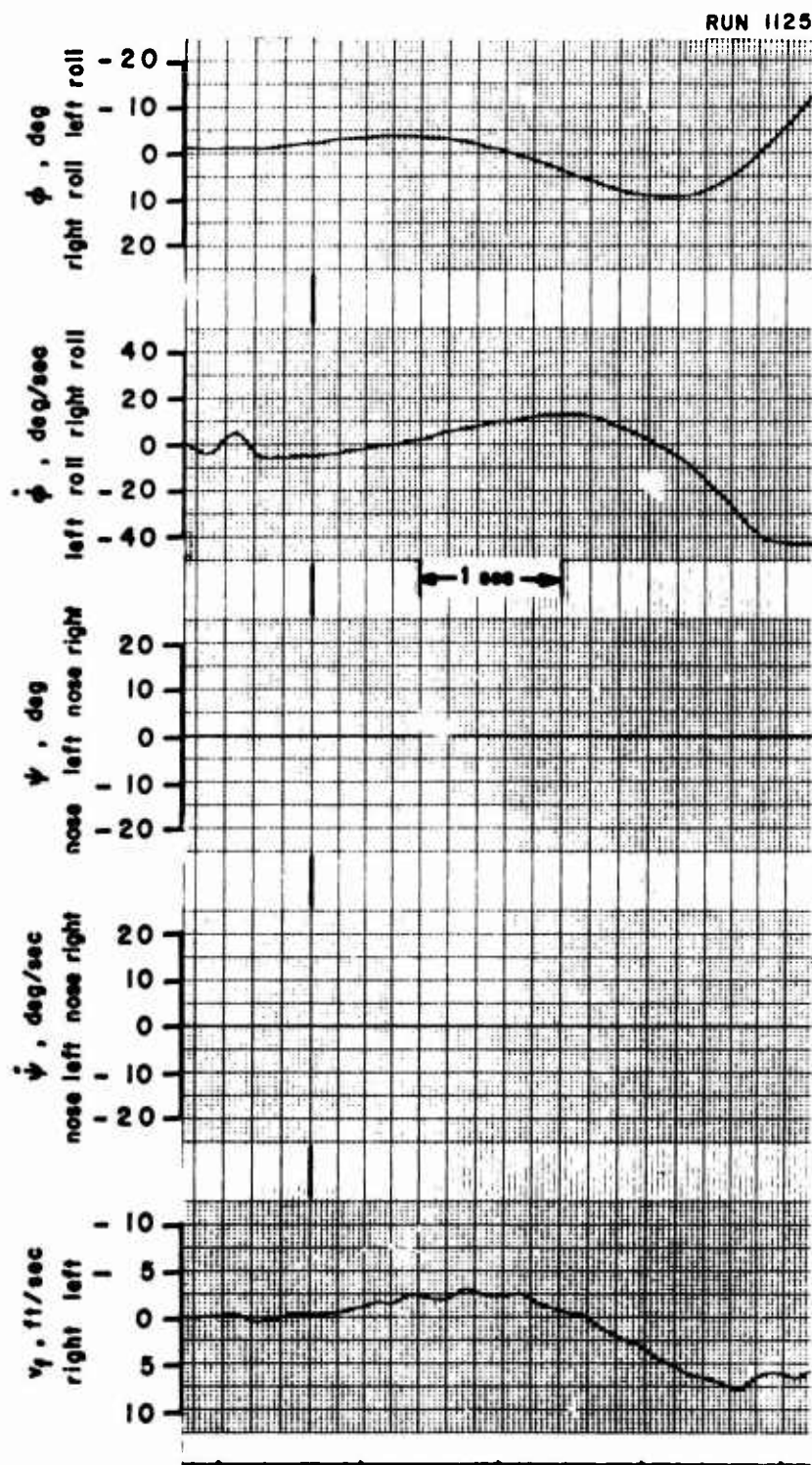
Figure 12. Lateral/Directional Transient Response. Two Degrees of Freedom, \phi - v_y . i_d = 80^\circ , U_{of} = 10 ft/sec, \delta_{75} = 25.2^\circ , rpm = 6780, \Delta\delta_o = 0.5^\circ , Large Vertical Tail.
