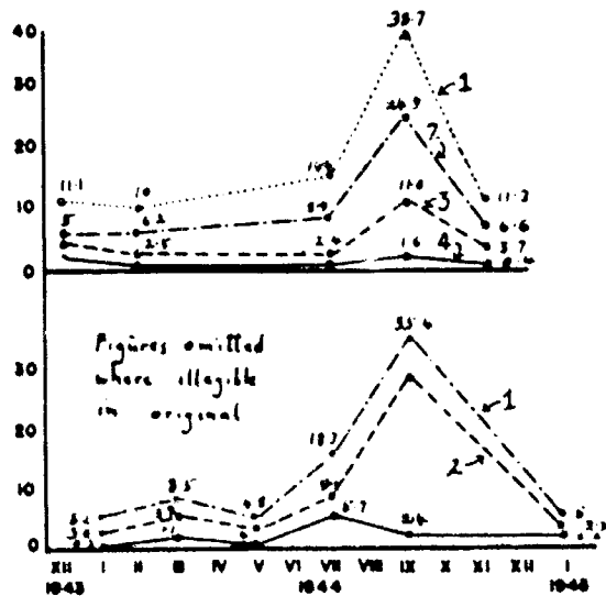
Fig. 1. Seasonal population-curves of basic species of small mammals.
