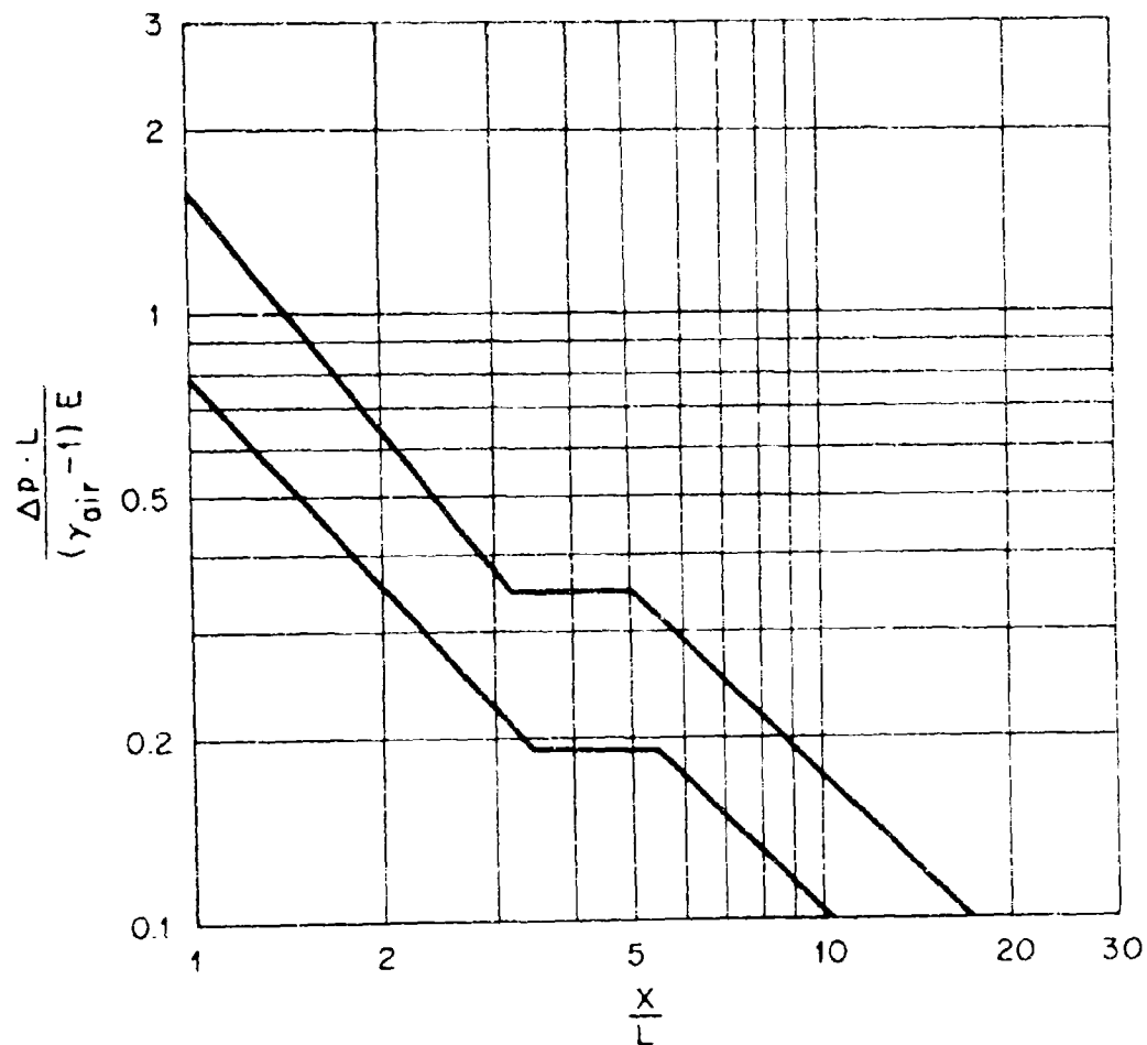
Fig. 10.3 Calculated shock overpressure as a function of distance down the shock tube for two values of the adiabatic exponent (ratio of specific heats) of the burned gas.
