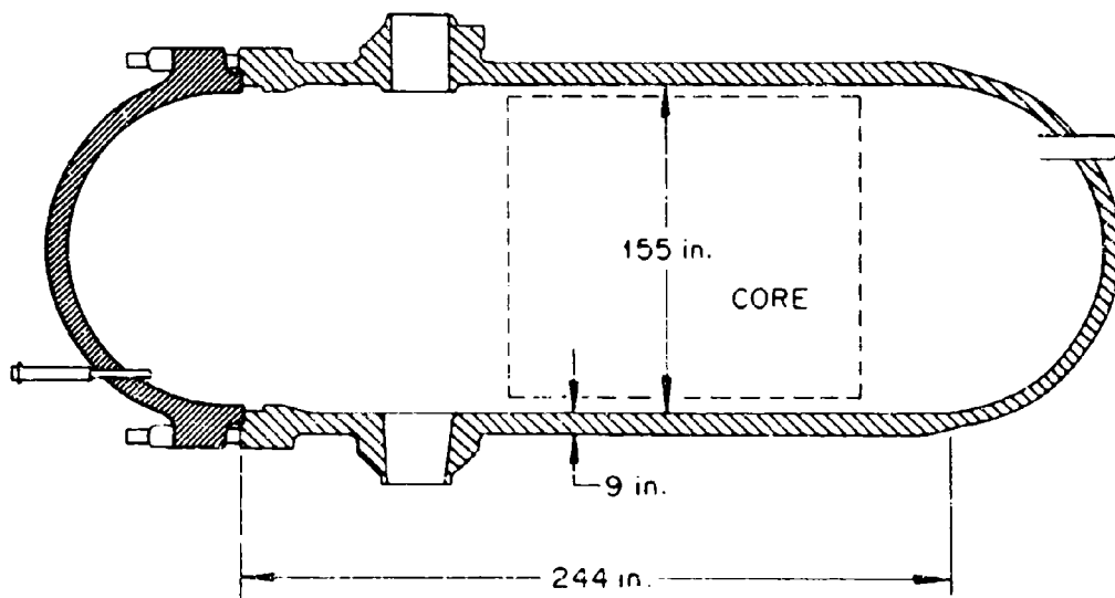
Fig. 12.4. Turkey Point, Florida, Reactor Pressure Vessel Outline.
