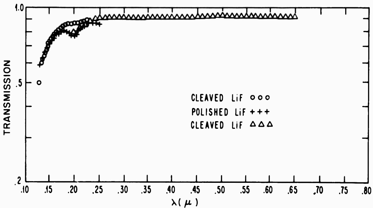
FIG 3-4 TRANSMISSION SPECTRA OF VARIOUS SUBSTRATE MATERIALS.
