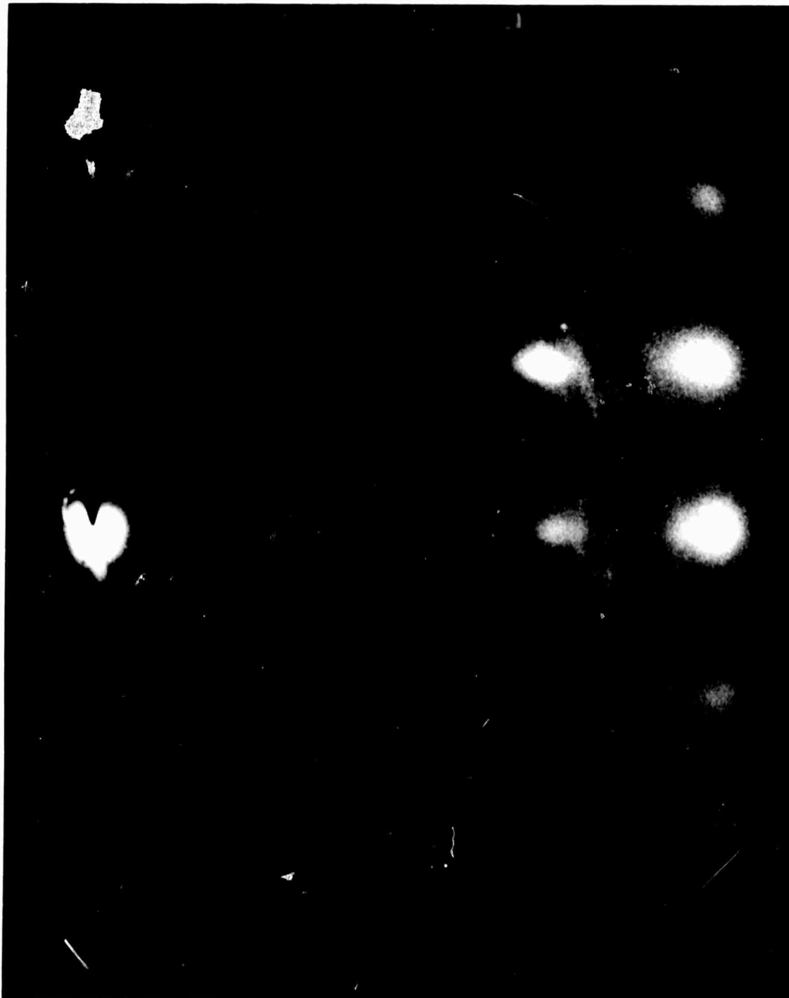
FIG. 2-9 ELECTRON DIFFRACTION PATTERN OF A FILM GROWN ON LiF BY SPUTTERING Ni IN A 20% O 2 , 80% Ar ATMOSPHERE OF .9 MICRONS. THE SPUTTERING TIME WAS TWENTY MINUTES.
