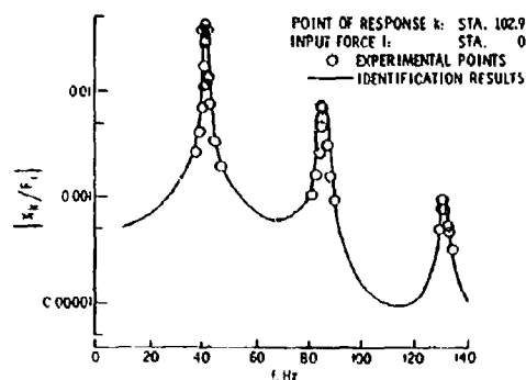
Fig. 7. Comparison of identification results with experimental frequency response for 1/40-scale model
