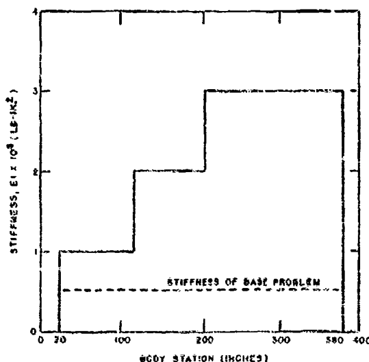
Fig. 1. Bending rigidity of a missile
