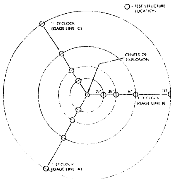
Fig. 2. Layout of test structure locations
