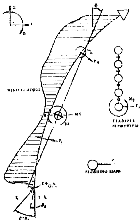
Fig. 1 Loading diagram for in-flight vehicle
