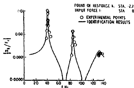
Fig. 8. Comparison of identification results with experimental frequency response for 1/40-scale model
