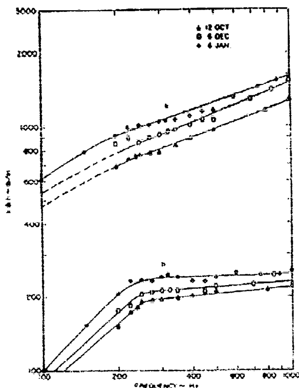
Fig. 5. k and h vs frequency
