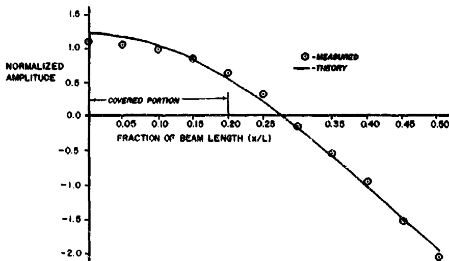
Fig. 9. Measured mode shape with 40 percent coverage
