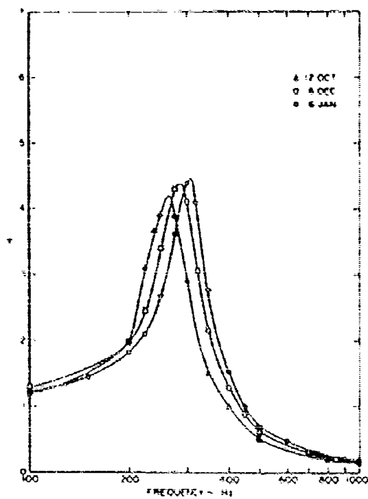
Fig. 7. Amplification factor vs frequency
