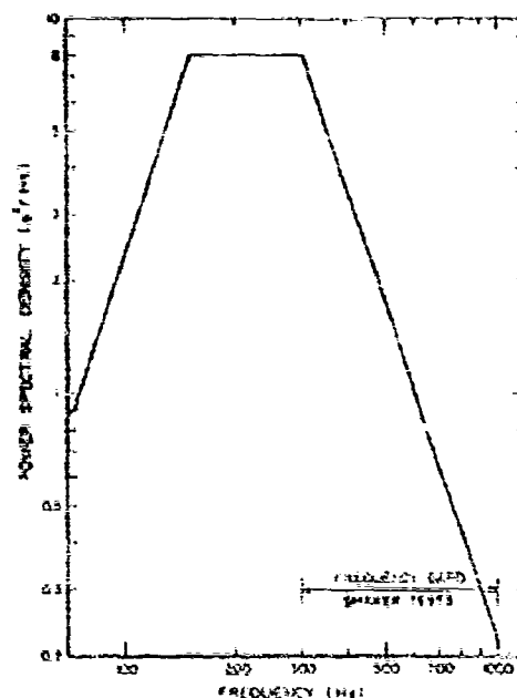
Fig. 2. Derived broadband random spectrum
