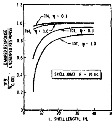
Fig. 8. Damping effectiveness for an impulsive load
