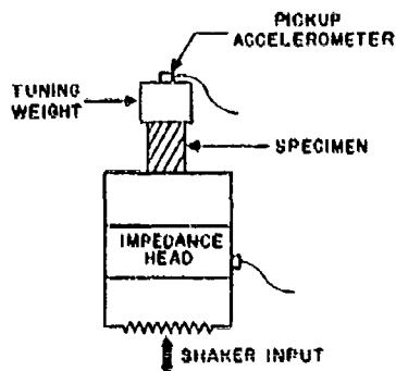
Fig. 1. Sketch of experimental setup
