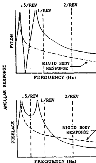
Fig. 1. Conventional helicopter isolation system with vertical restraint
