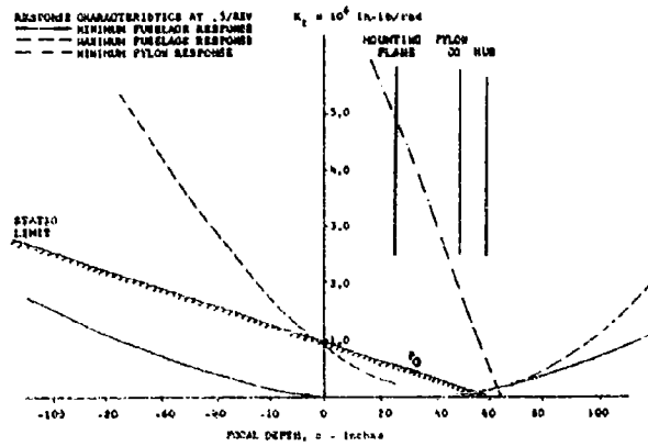
(a) At 0.5/rev
