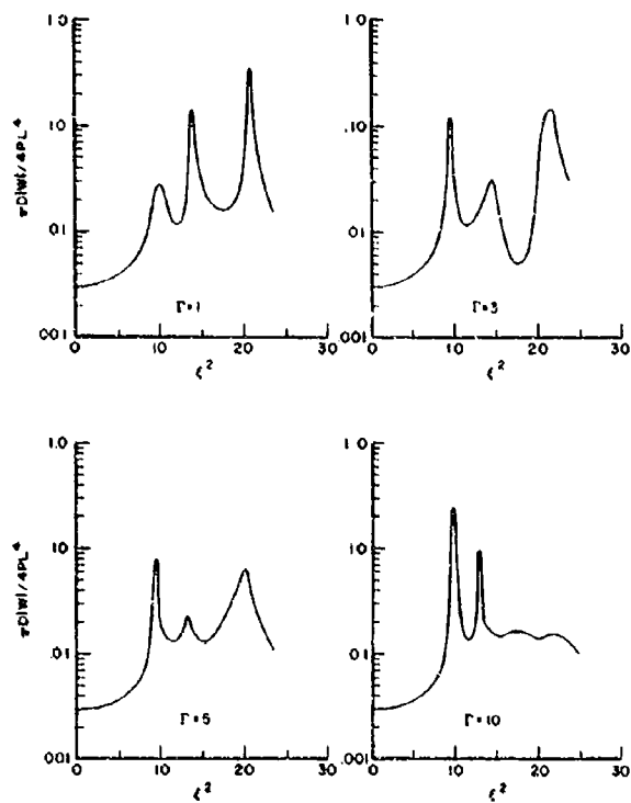
Fig. 4. Typical graphs of \pi |D|W|/4PL^4 against \zeta^2 for \lambda = 0.8
