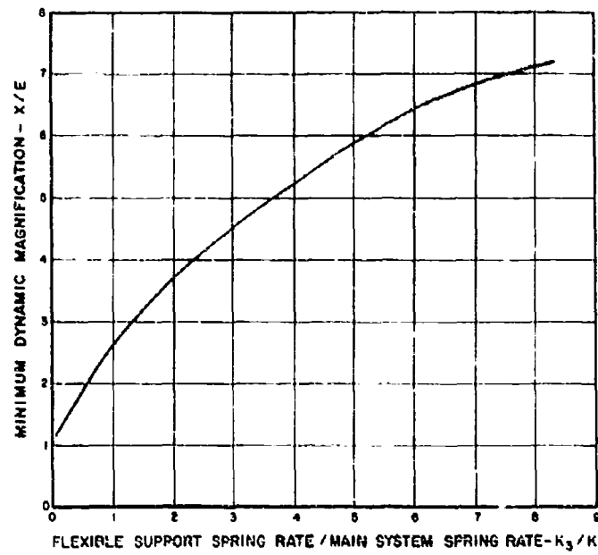
Fig. 6. Minimum-amplitude magnification as a function of flexible support spring rate
