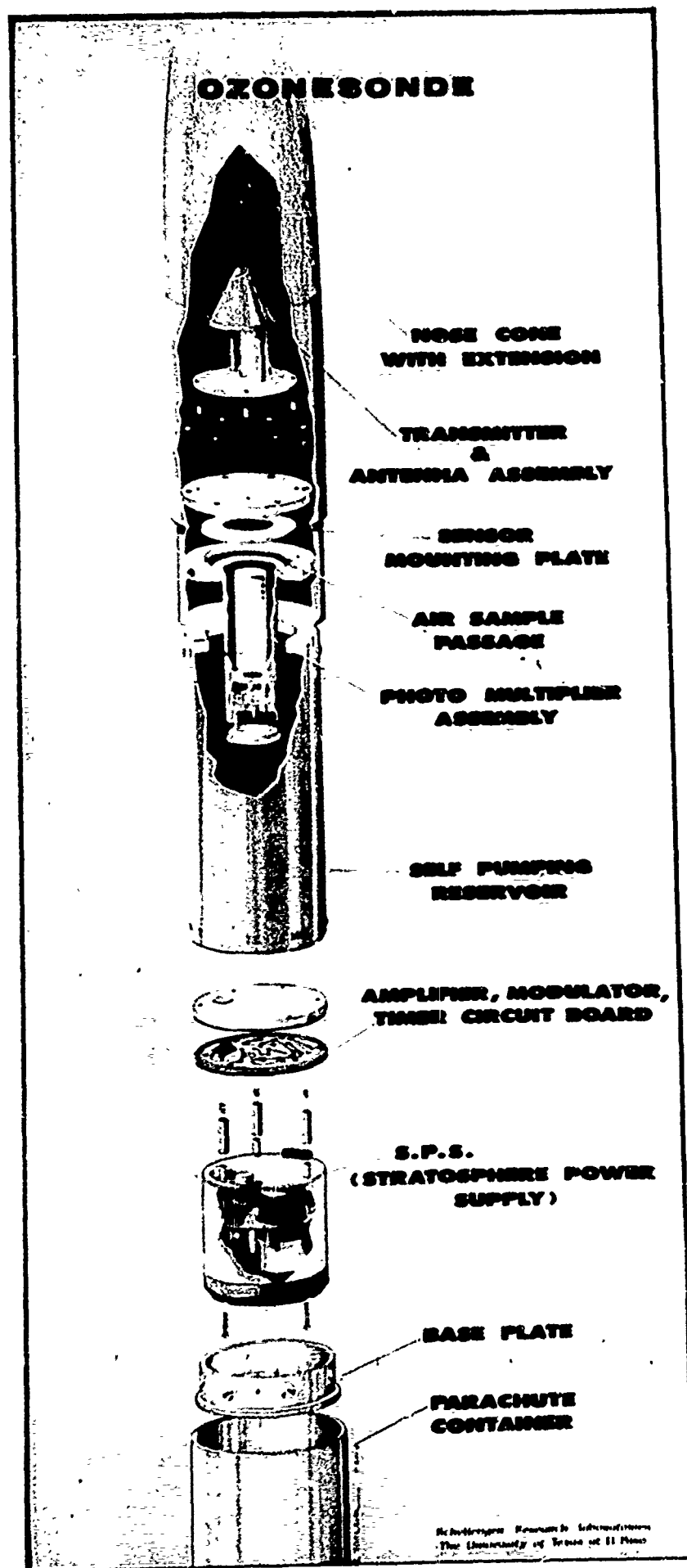
FIGURE 2. SCHEMATIC DIAGRAM OF THE ROCKET-BORNE OZONESONDE.
