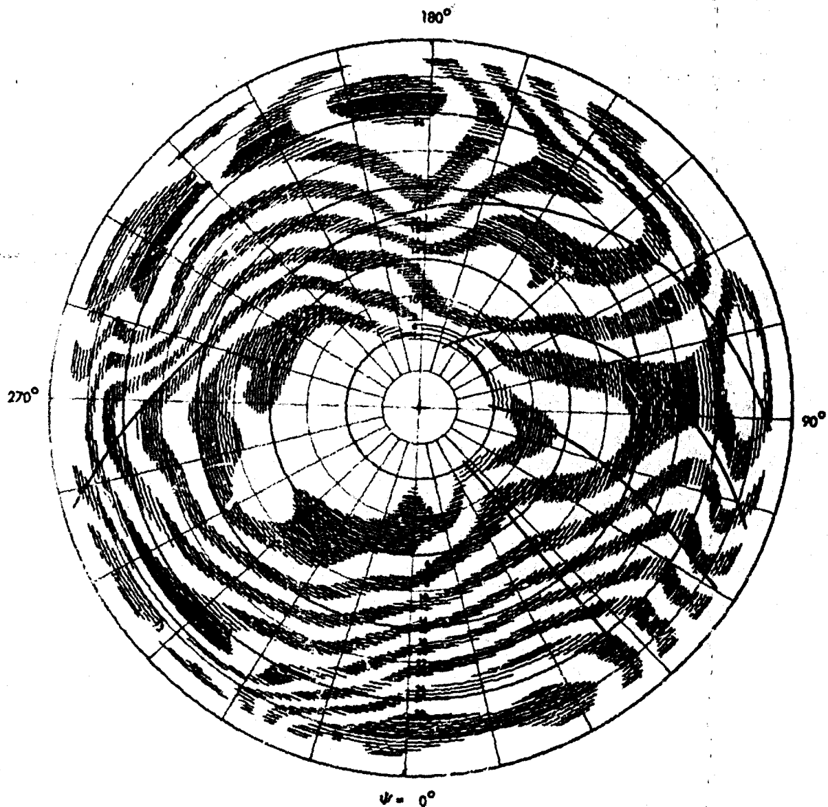
Figure 26. Computer-Drawn Contour Plot of Blade Airload Data From Scheiman.
