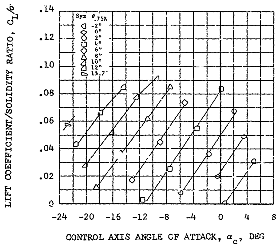
Figure 14. Nondimensional Performance Data for the 44-Foot-Diameter Rotor for Various Blade Collective Pitch Angles, \mu = 0.31 ; M(1.0, 90.) = 0.88 .
