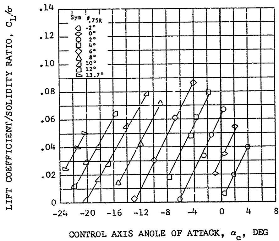
Figure 21. Nondimensional Performance Data for the 44-Foot-Diameter Rotor for Various Blade Collective Pitch Angles, \mu = 0.46 ; M_{(1.0, 90.)} = 0.86 .
