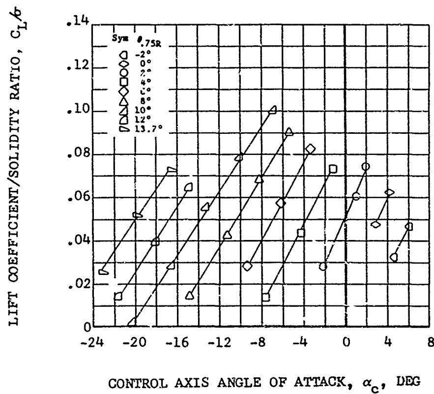
Figure 19. Nondimensional Performance Data for the 44-Foot-Diameter Rotor for Various Blade Collective Pitch Angles, \mu = 0.45 ; M_{(1.0, 90.)} = 0.77 .
