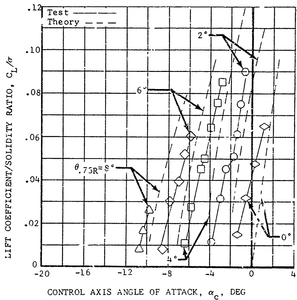
Figure 10. Test-Theory Comparison, Nondimensional Performance of the 34-Foot-Diameter Rotor for Various Collective Pitch Angles at \mu = 0.94 ; M_{(1.0, 90.)} = 0.49 .
