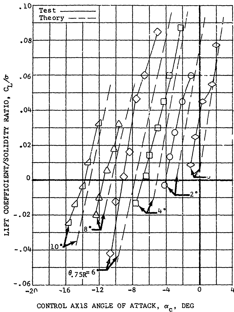
Figure 9. Test-Theoret Comparison, Nondimensional Performance of the 34-Foot-Diameter Rotor for Various Collective Pitch Angles at \mu = 0.86 ; M_{(1.0, 90.)} = 0.47 .
