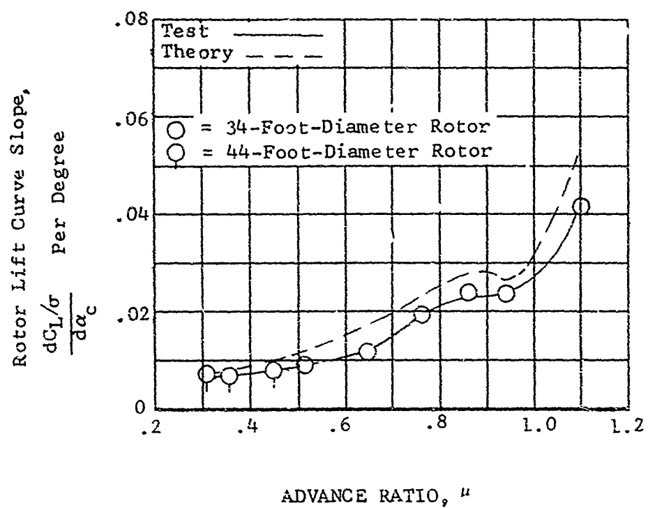
Figure 13. Test-Theory Comparison, Rotor Lift Curve Slope vs. Advance Ratio for Both Rotors.
