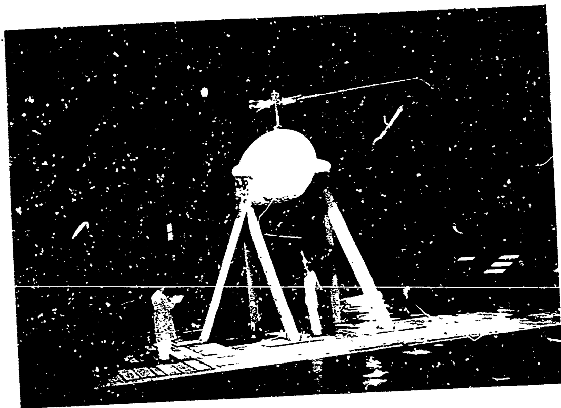
Figure 1. Full-Scale Rotor Wind Tunnel Test Module in the NASA-Ames 40- x 80-Foot Wind Tunnel.
