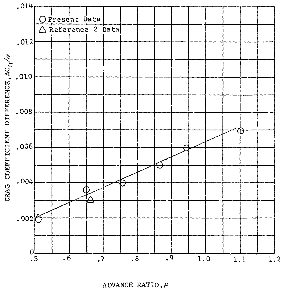
Fig. 5. 34-Foot-Diameter Rotor Test-Theory Comparison. Test-Theory Drag Coefficient Difference vs. Advance Ratio for M(1.0, 90.) Varying From 0.47 to 0.64.
