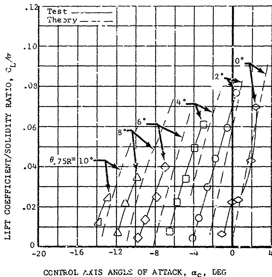
Figure 8. Test-Theory Comparison, Nondimensional Performance of the 34-Foot-Diameter Rotor for Various Collective Pitch Angles at \mu = 0.76 ; M_{(1.0, 90.)} = 0.50 .
