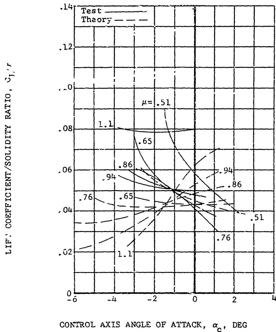
Figure 12. 34-Foot-Diameter Rotor Test-Theory Comparison of the Lift Variation with Control Axis Angle of Attack in Autorotation at Various Advance Ratios.
