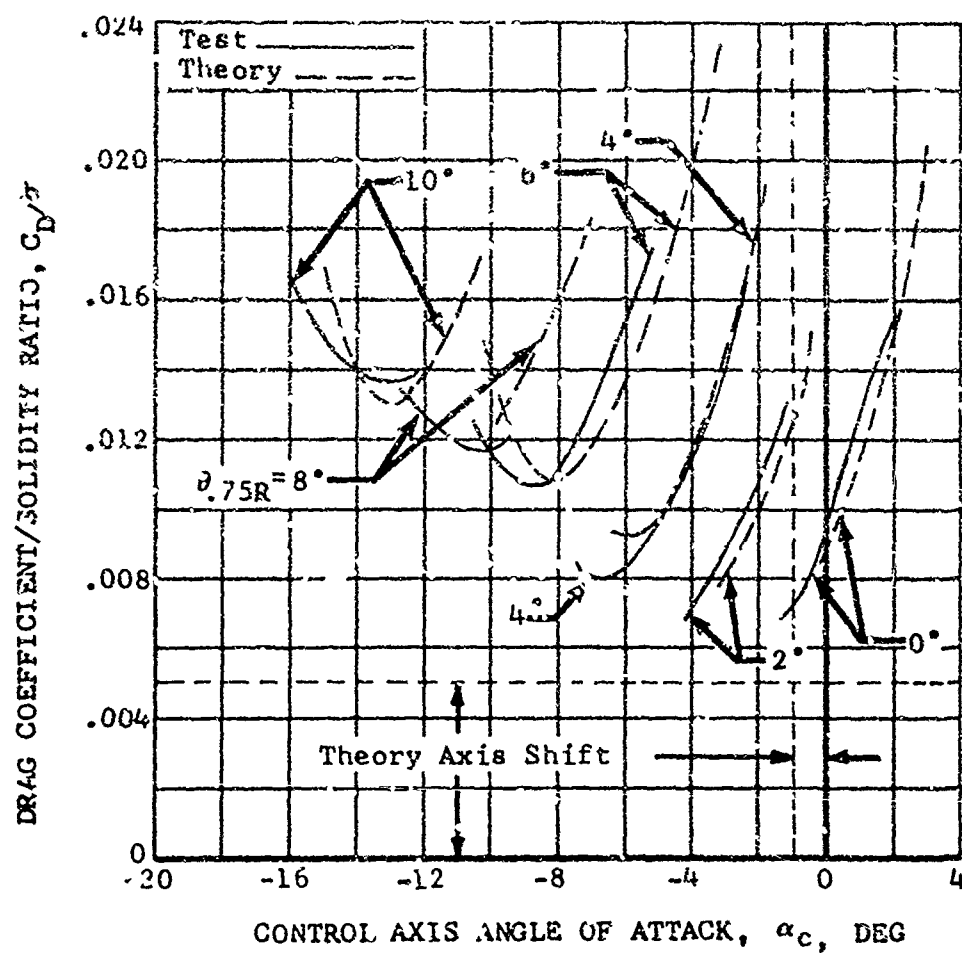
Figure 4. A Comparison of the Test-Theory Drag Coefficient/Solidity Ratio Versus Control Axis Angle of Attack for the 34-Foot-Diameter Rotor at \mu = 0.86 and M(1.0, 90^\circ) = 0.47 illustrating the Required Theory Axis Shift.
