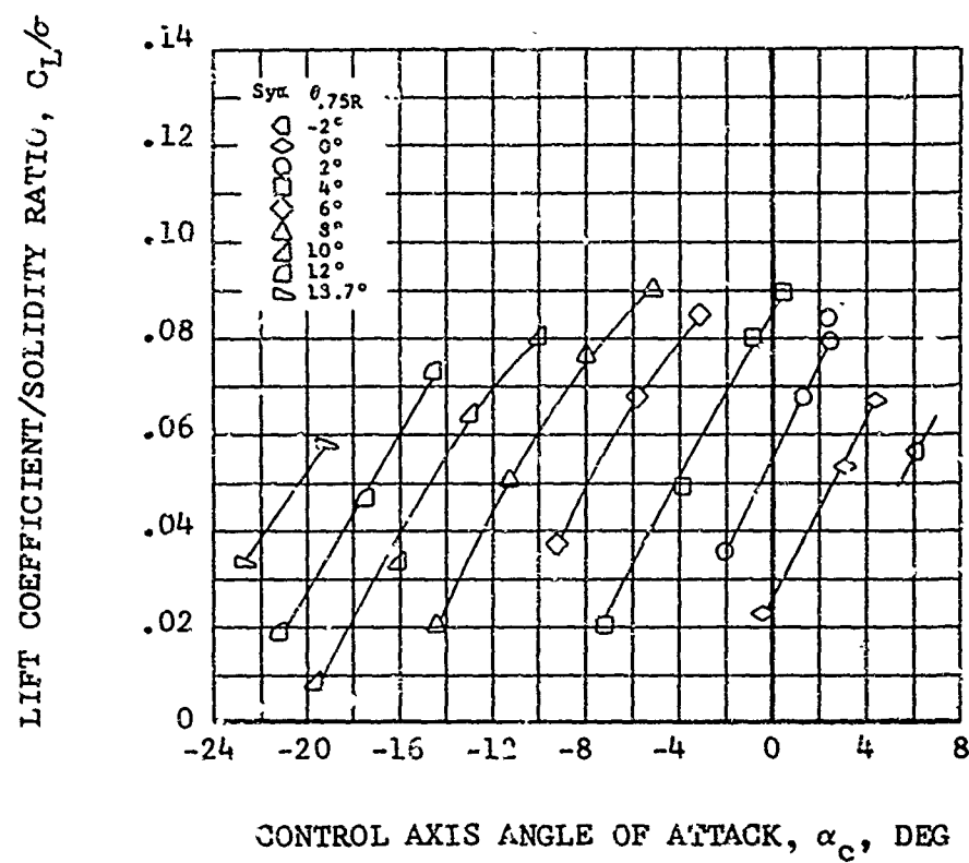
Figure 18. Nondimensional Performance Data for the 44-Foot-Diameter Rotor for Various Blade Collective Pitch Angles, \mu = 0.41 ; M(1.0, 90.) = 0.94 .
