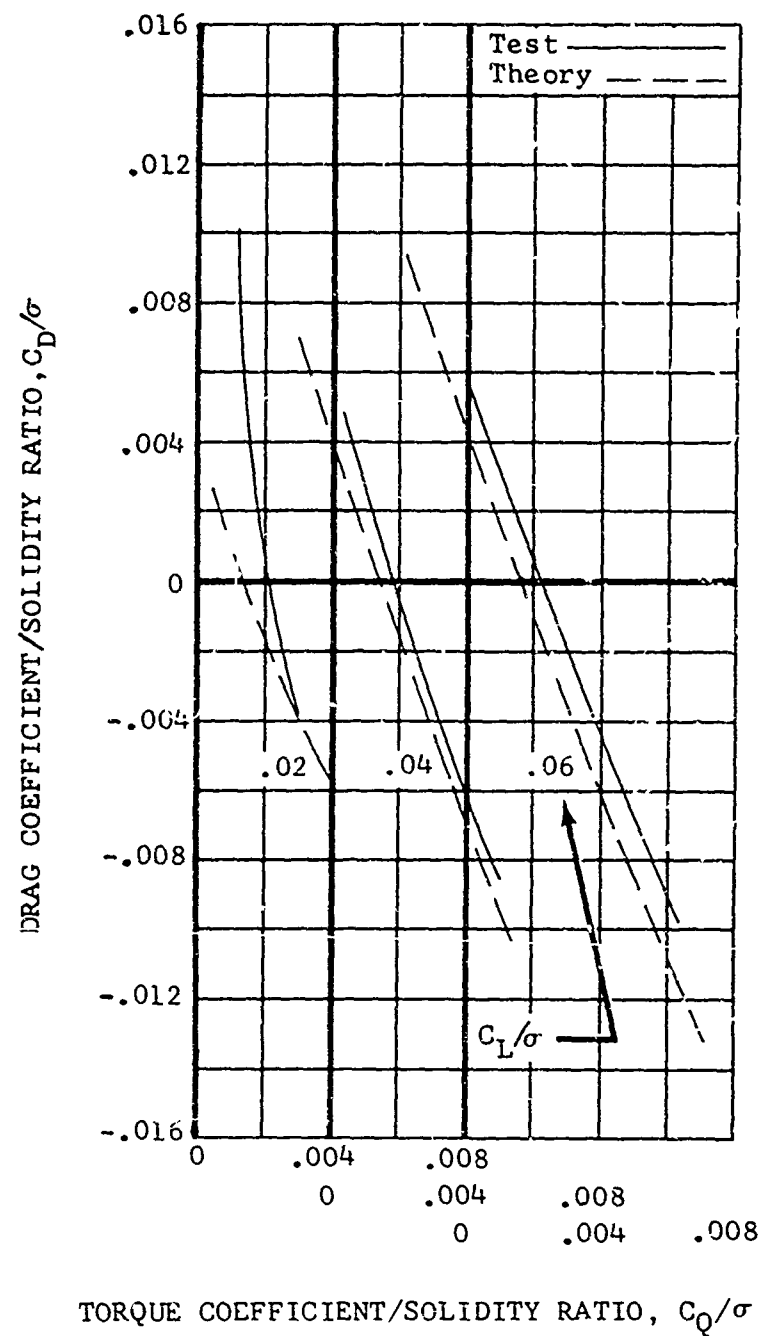
a) \mu = 0.36 ; M(1.0, 90.) = 0.80 Figure 2. Test-Theory Comparison, Nondimensional Performance of 44-Foot-Diameter Rotor at Various Combinations of Advance Ratio and Advancing Tip Mach Number.
