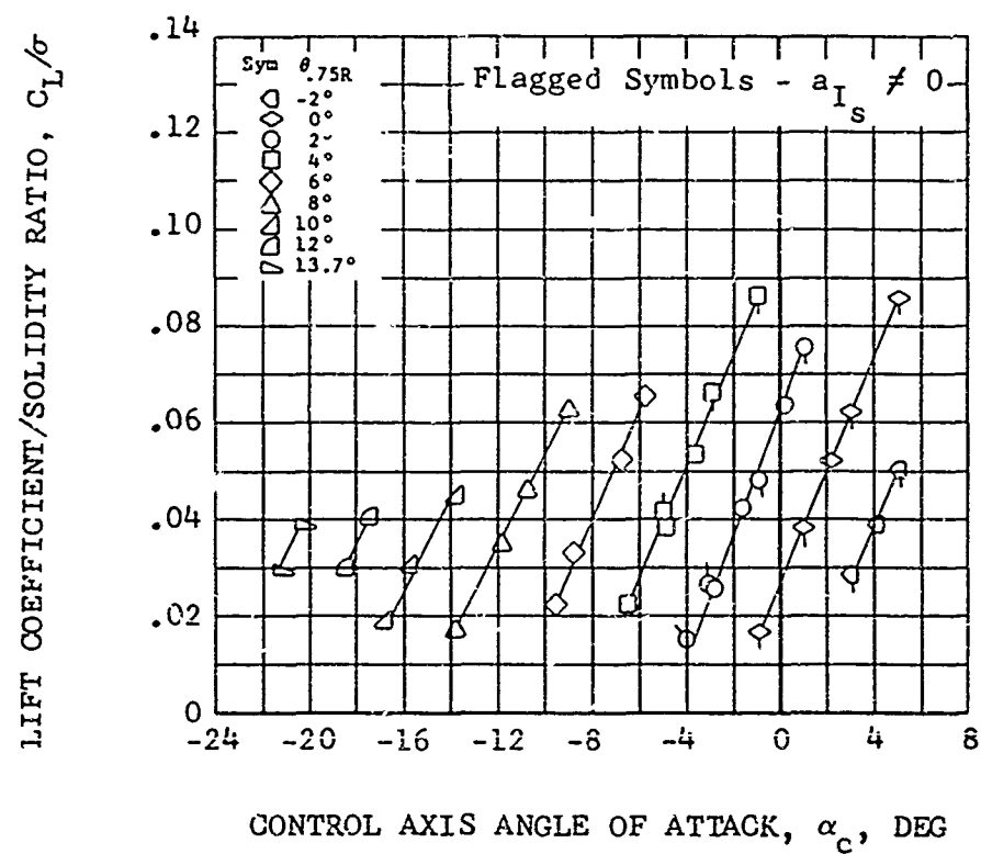
Figure 22. Nondimensional Performance Data for the 44-Foot-Diameter Rotor for Various Blade Collective Pitch Angles, \mu = 0.51 ; M_{(1.0, 90.)} = 0.80 .
