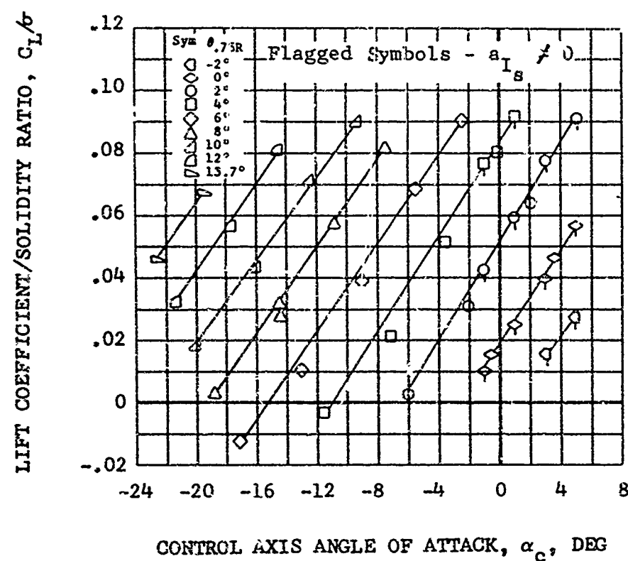
Figure 15. Nondimensional Performance Data for the 44-Foot-Diameter Rotor for Various Blade Collective Pitch Angles, \mu = 0.36 ; M_{(1.0, 90.)} = 0.80 .
