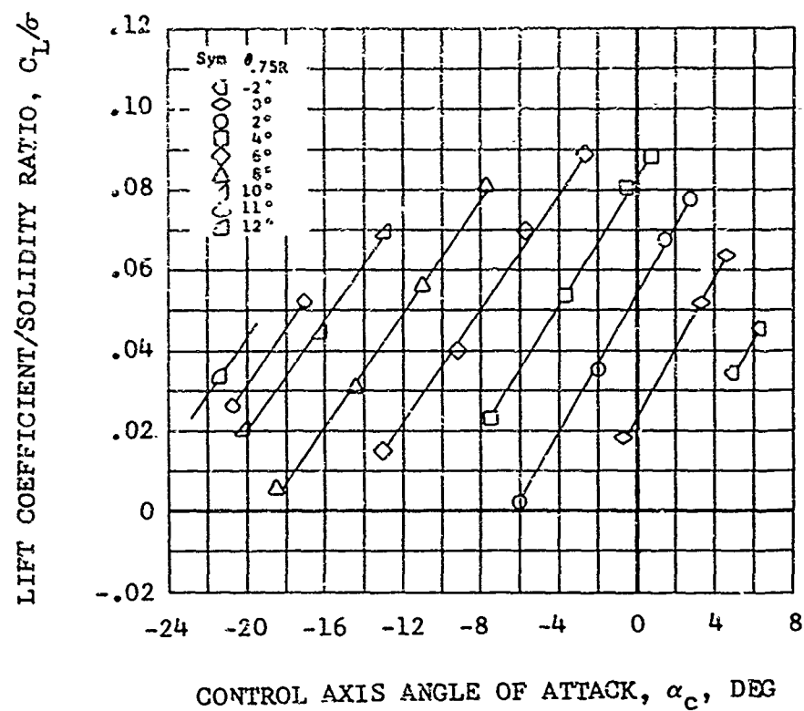
Figure 16. Nondimensional Performance Data for the 44-Foot-Diameter Rotor for Various Blade Collective Pitch Angles, \mu = 0.36 ; M(1.0, 90.) = 0.90 .
