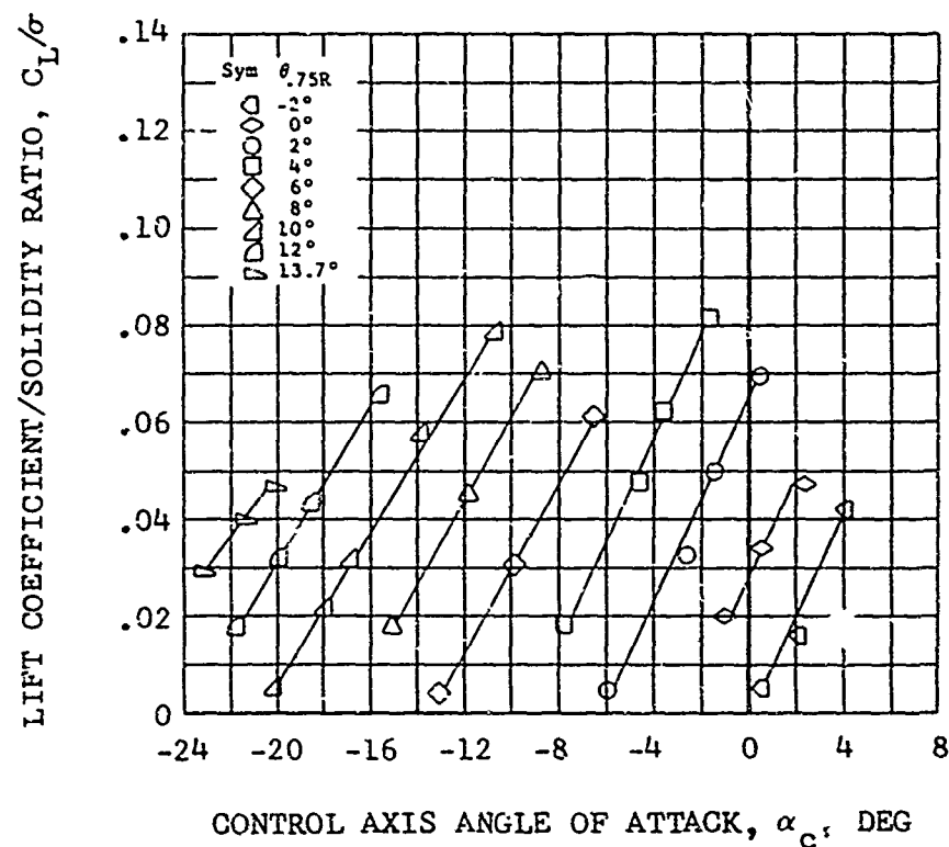
Figure 20. Nondimensional Performance Data for the 44-Foot-Diameter Rotor for Various Blade Collective Pitch Angles, \mu = 0.45 ; M(1.0, 90.) = 0.90 .
