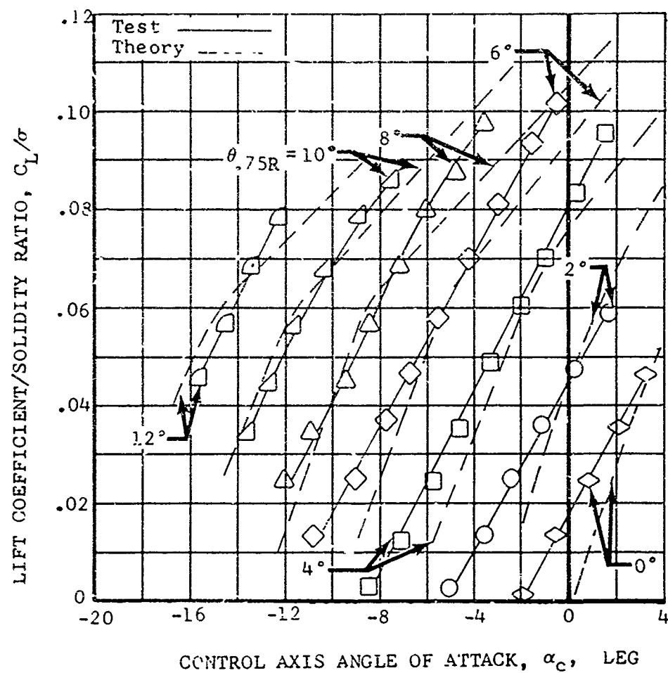
Figure 6. Test-Theory Comparison, Nondimensional Performance of the 34-Foot-Diameter Rotor for Various Collective Pitch Angles at \mu = 0.51 ; M_{(1.0, 90)} = 0.64 .
