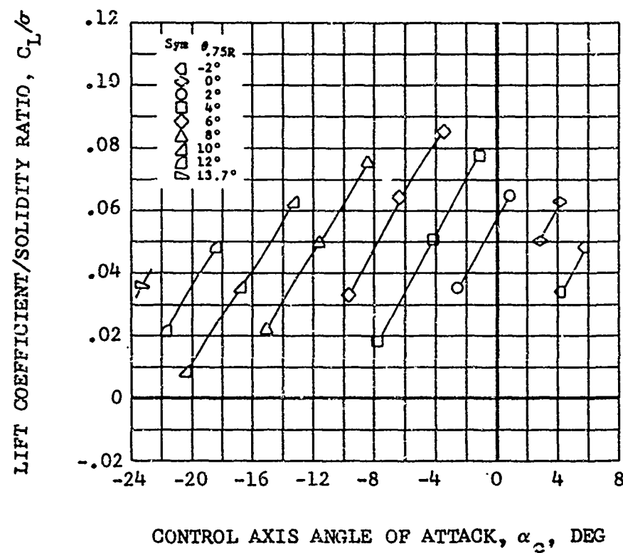
Figure 17. Nondimensional Performance Data for the 44-Foot-Diameter Rotor for Various Blade Collective Pitch Angles, \mu = 0.40 ; M(1.0, 90.) = 0.83 .
