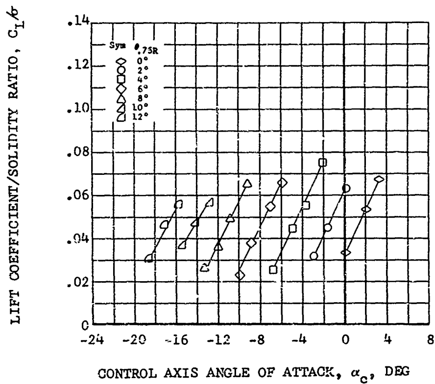
Figure 23. Nondimensional Performance Data for the 44-Foot-Diameter Rotor for Various Blade Collective Pitch Angles, \mu = 0.52 ; M_{(1.0, 90.)} = 0.81 .
