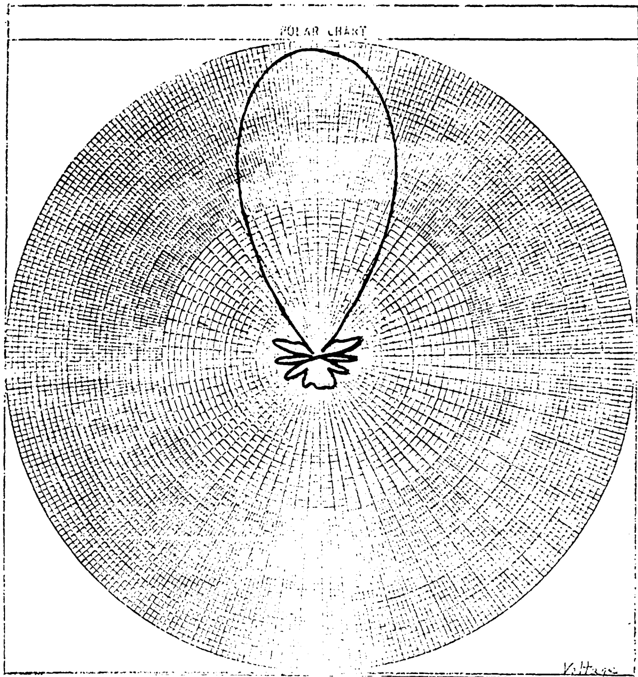
FIGURE 35. 1.5 GHz H-PLANE WITH TERMINATIONS
