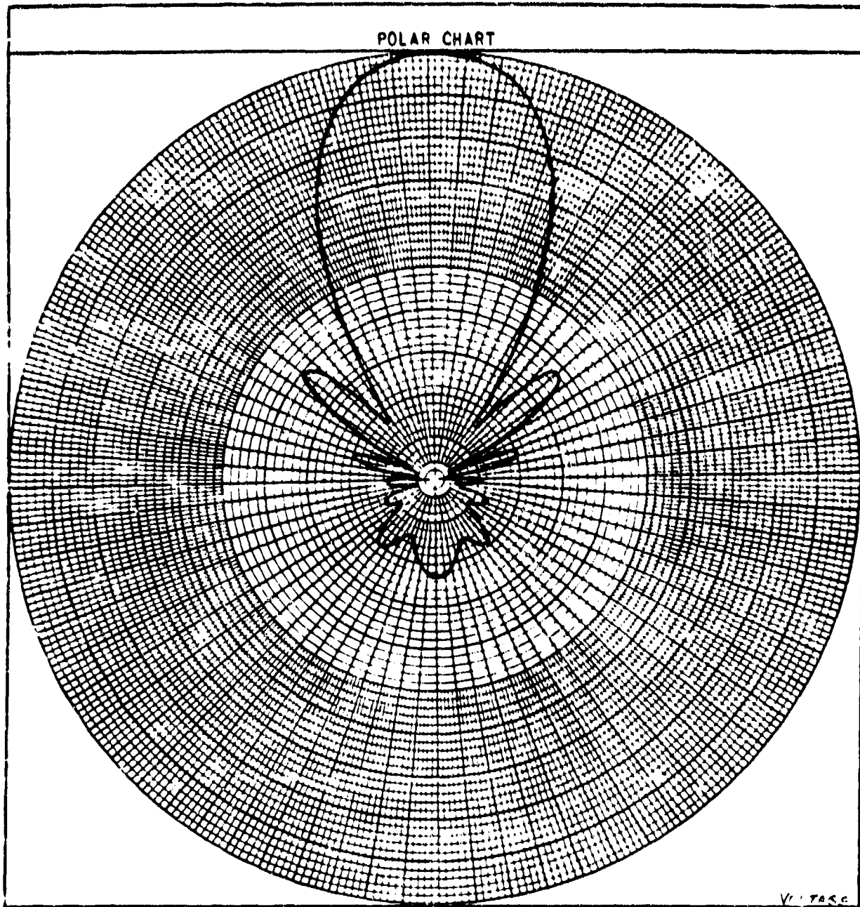
FIGURE 10. 2.0 GHz E-PLANE
