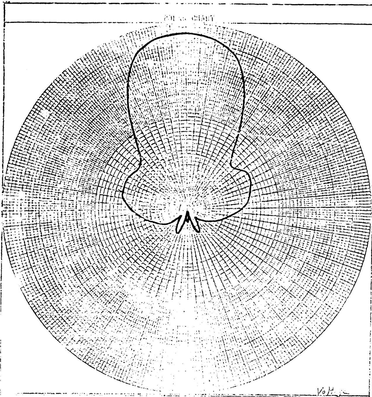
FIGURE 36. 1.5 GHz E-PLANE WITH TERMINATIONS
