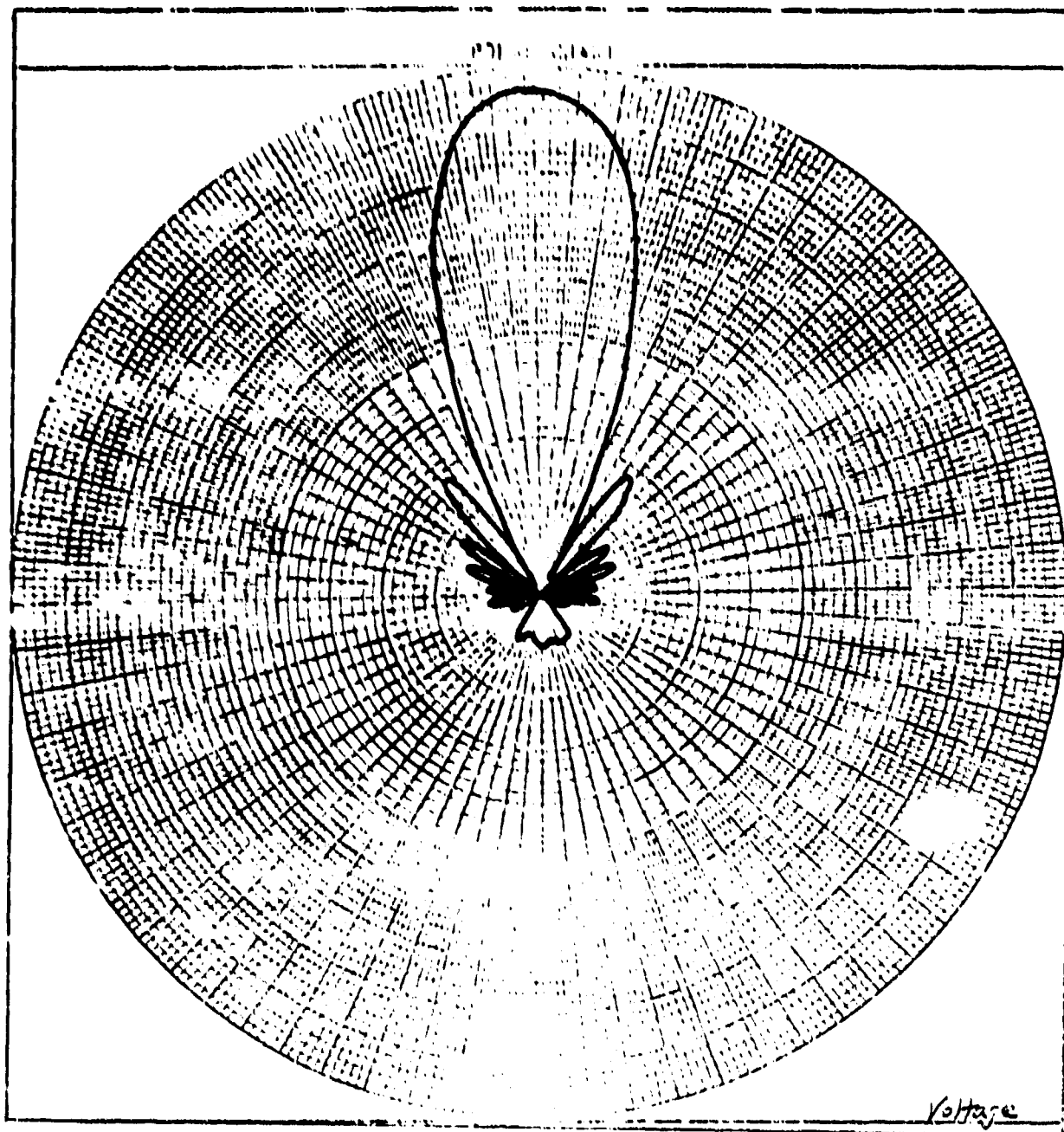
FIGURE 12. 3.0 GHz E-PLANE
