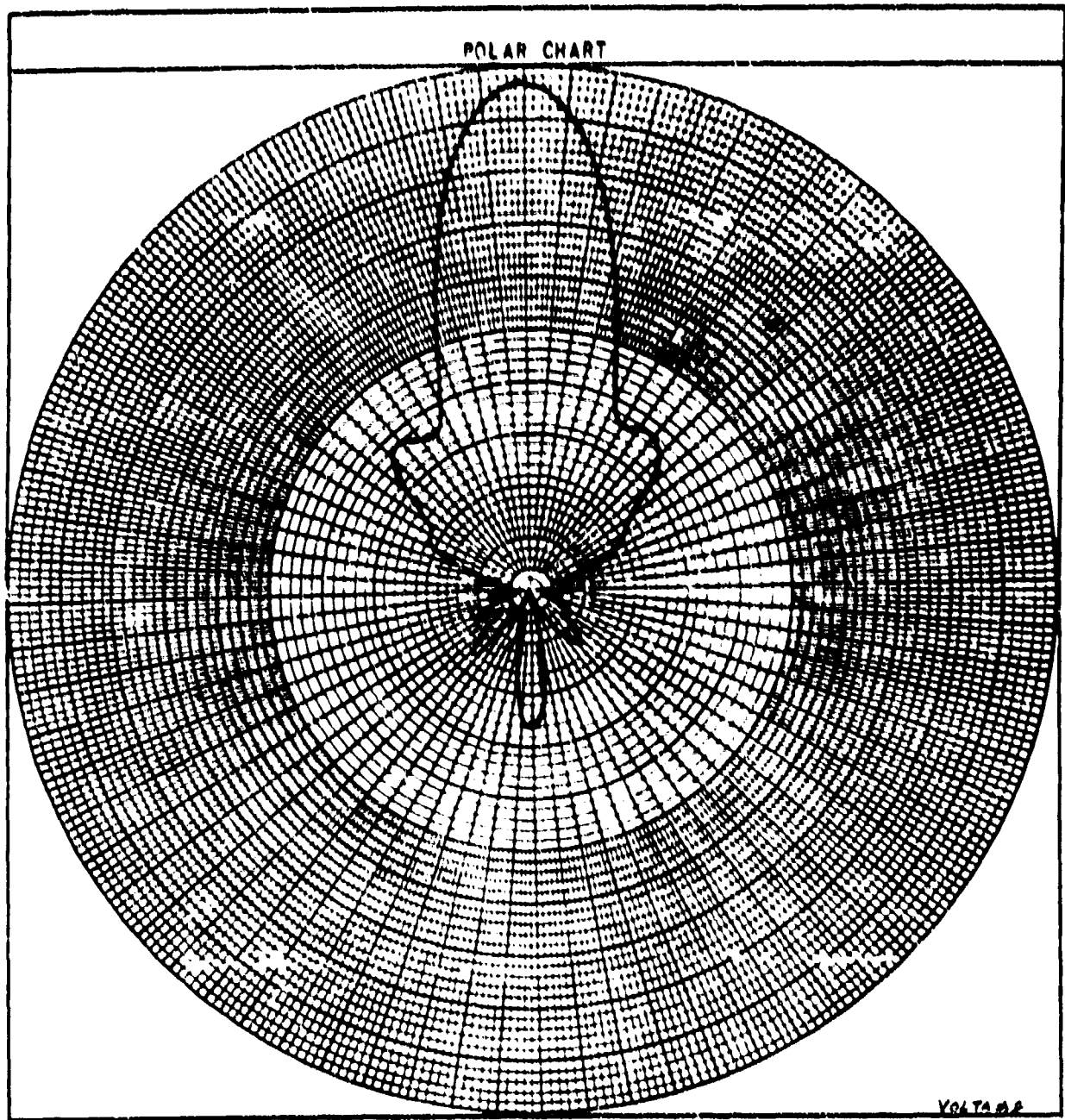
FIGURE 11. 2.0 GHz E-PLANE
