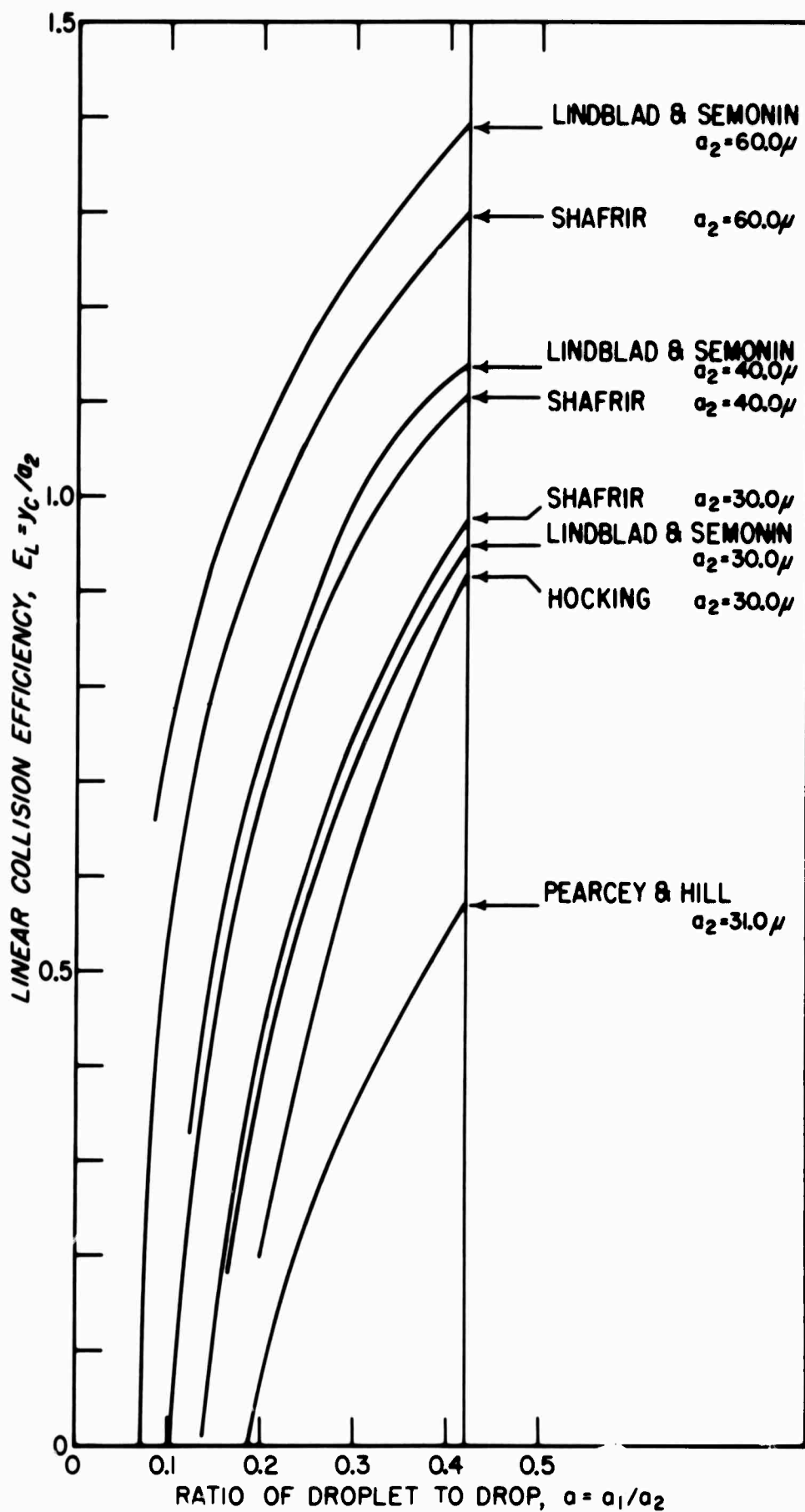
Fig. 17 Comparison of linear collision efficiency as calculated by various authors.
