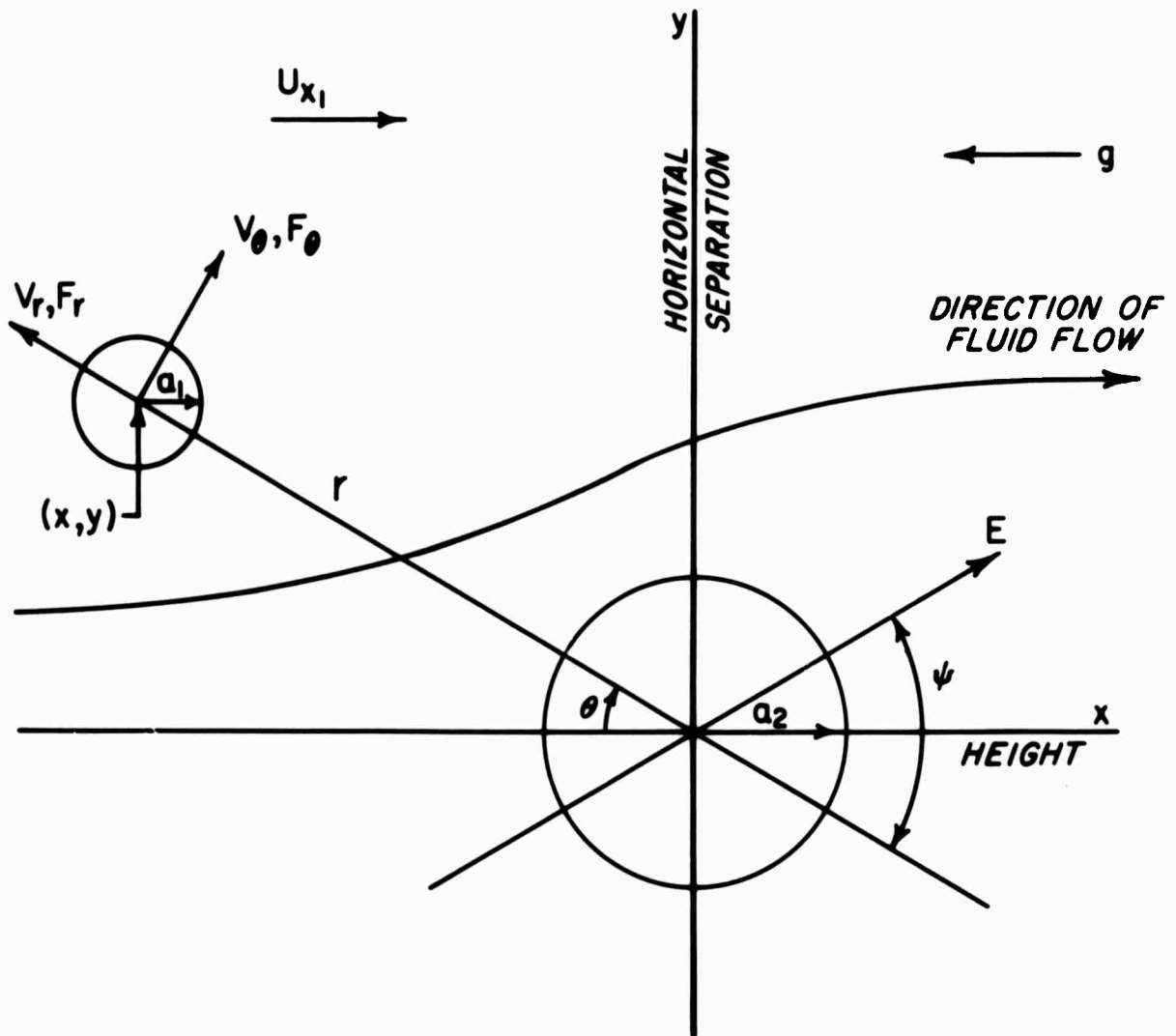
Fig. 18 Motion of a droplet in an electric field, E , relative to a fixed drop.
