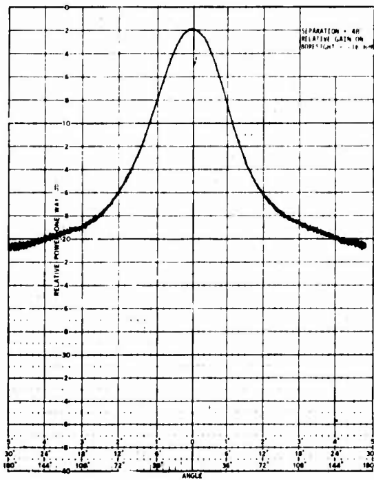
Figure 10. Near-Field Mutual Coupling Between a Dipole and Hooded Probe Antenna at Separation Distances of 28, 36, 48 and 60 Inches.
