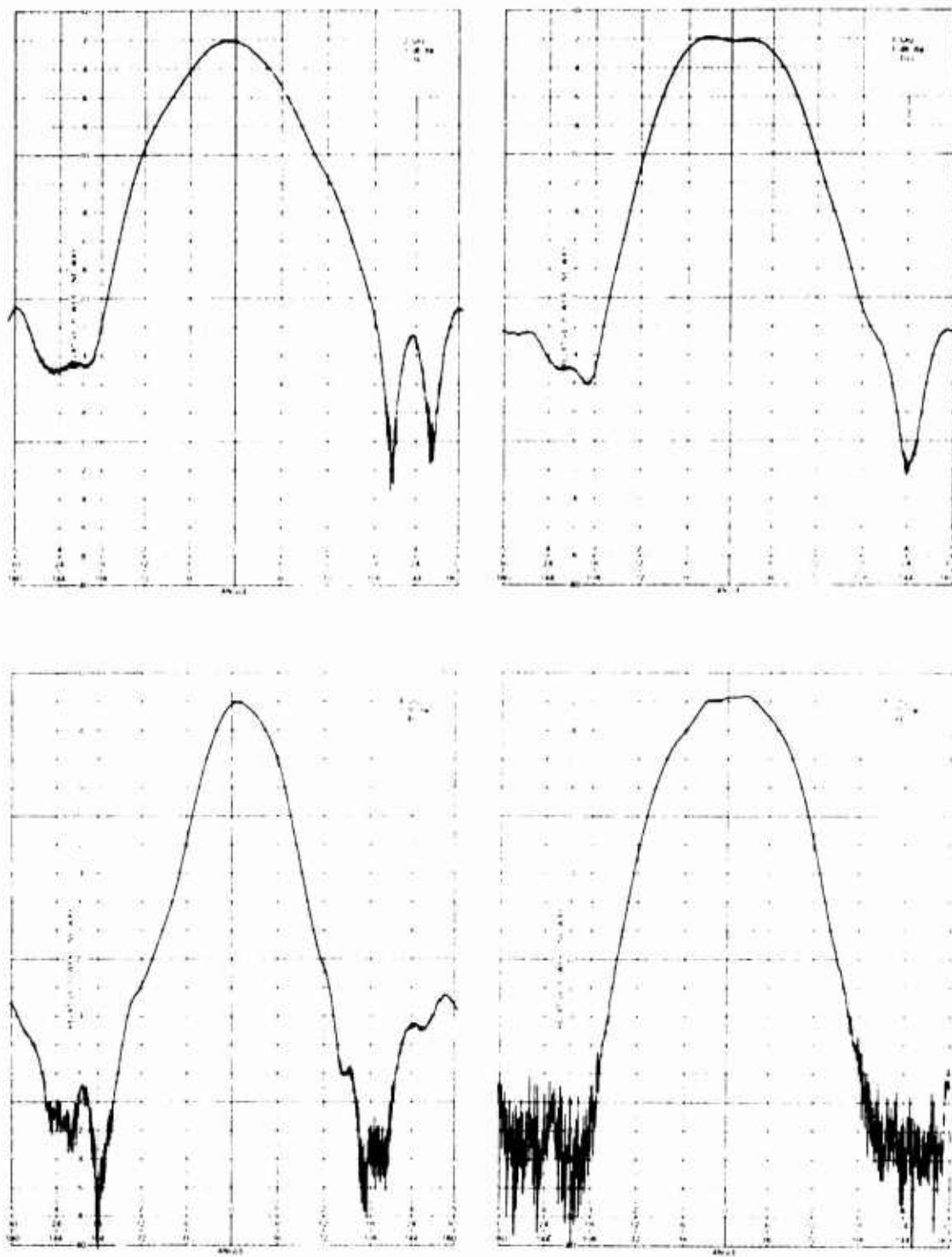
Figure 18. Antenna Patterns for 10A and 10A Antenna at 1.5, 2, 3 and 4 MHz.
