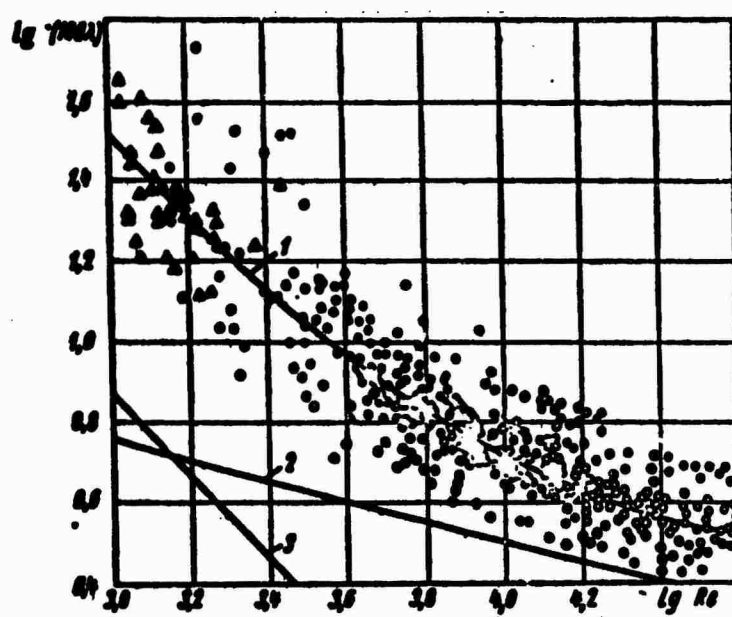
Fig. 41. Dependence of coefficient of friction on Reynolds number: 1 - average curve; 2 - according to the Blasius law; 3 - according to Poiseuille law; ○ - gasoline; ● - kerosene; Δ - turbine oil.
