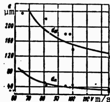
Fig. 106. Dependence of median and maximum diameter of drops of liquified paraffin on airflow velocity in the throat of a diffuser. Diameter of throat 11.5 mm, diameter of nozzle hole 1 mm. Ratio of volumetric flow rates of paraffin and air (0.96 - 0.59) \times 10^{-3} .
