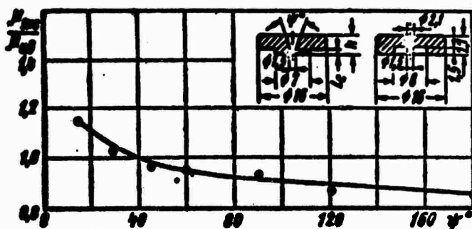
Fig. 45. Dependence of relative discharge coefficient on angle of cone on entrance into nozzle.
