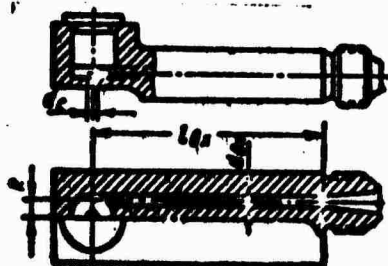
Fig. 39. Diagram of experimental injectors.
