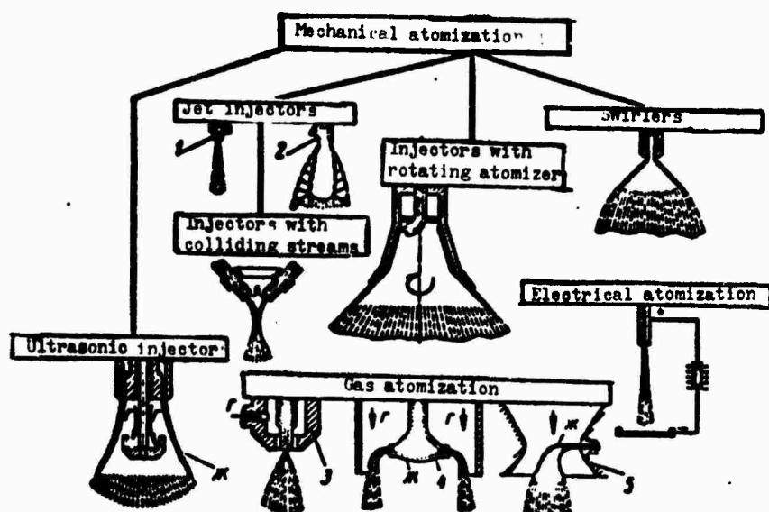
Fig. 1. Scheme of classification of methods of atomization: 1 - cylindrical nozzle; 2 - slot nozzle; 3 - atomizer with coaxial fluid and gas flows; 4 and 5 - atomizers with feed of liquid at a right angle to the airflow; Γ) gas; Ж) liquid.
