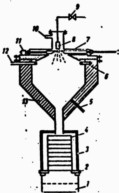
Fig. 155. Setup for sampling and freezing drops of liquid [10]: 1 - overflow of liquid nitrogen; 2 - flange of set of screens; 3 - insulated housing of set of screens; 4 - screen; 5 - thermocouple; 6 - collector for liquid nitrogen; 7 - spray cutoff; 8 - injector; 9 - solenoid valve; 10 - gas inlet; 11 - relay; 12 - liquid nitrogen inlet; 13 - silica gel thermoinsulation.
