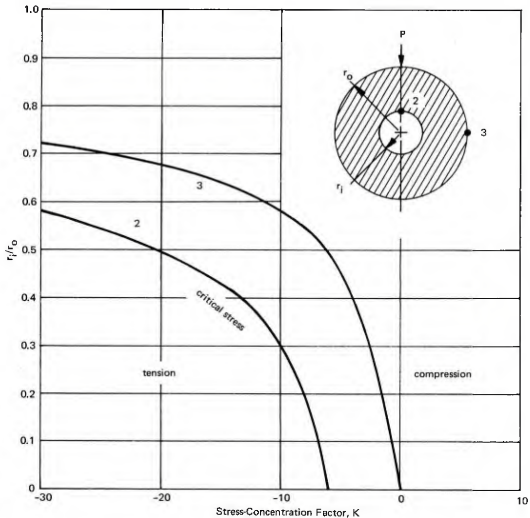
Figure 1. Stress at characteristic points in a ring under compression (from Assur, 1960).
