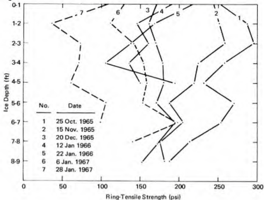
Figure 5. Chronological trend in ring-tensile strength profile.
