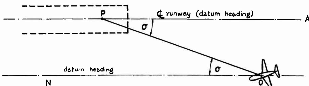
b AZIMUTH
