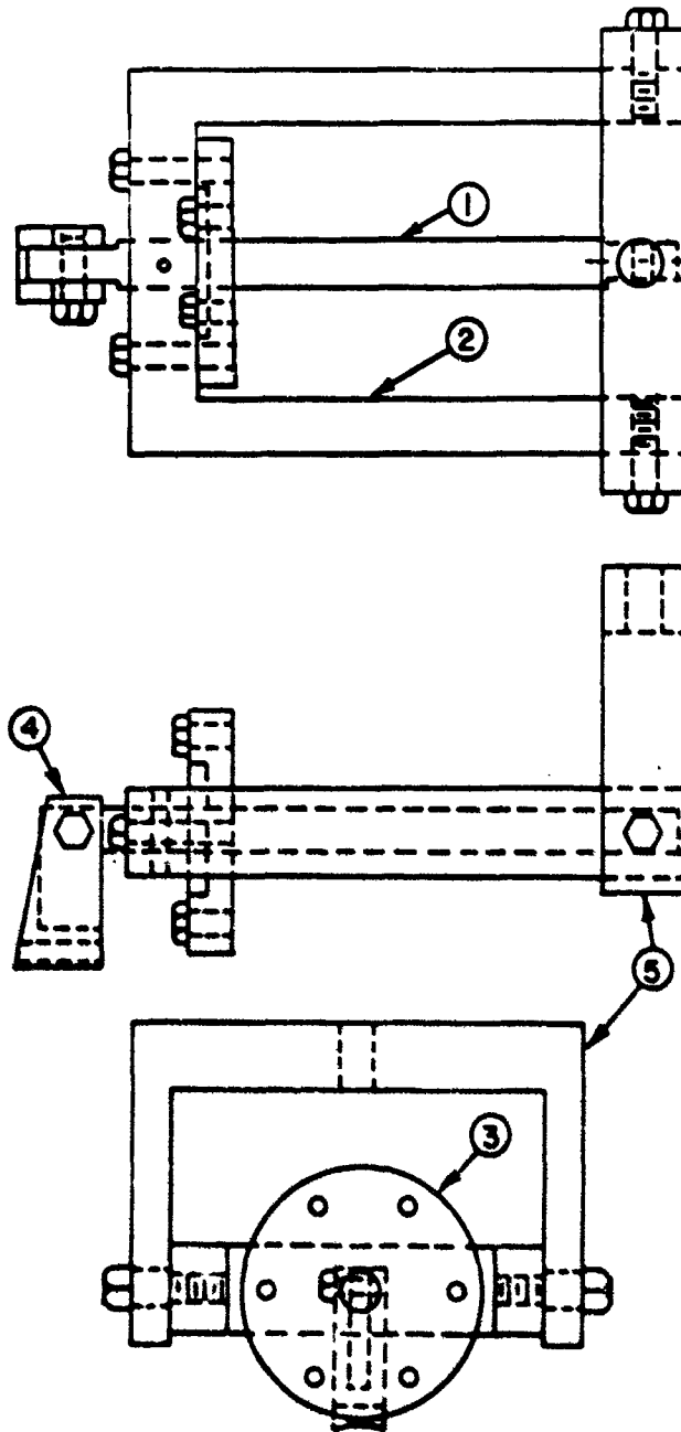
Figure 16. Feed Through Assembly
