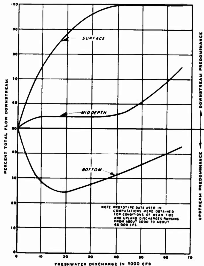
Fig. V-7. Predominance of flow in surface and bottom strata, Savannah Harbor
