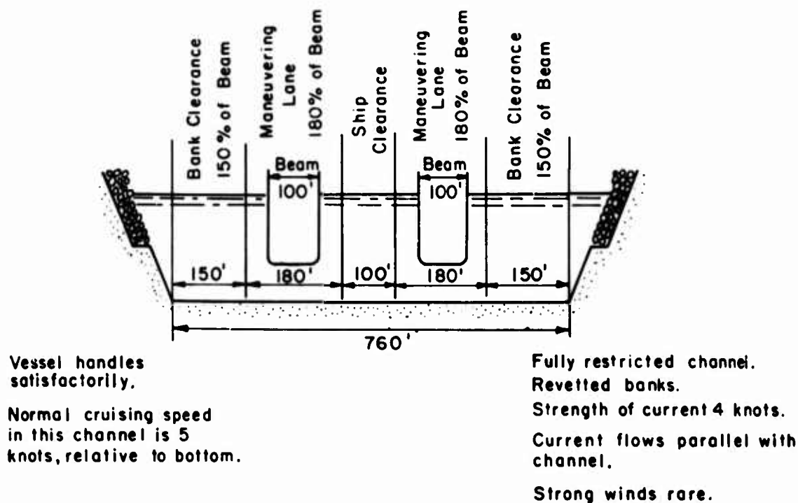
Fig. X-10. Elements of channel width
