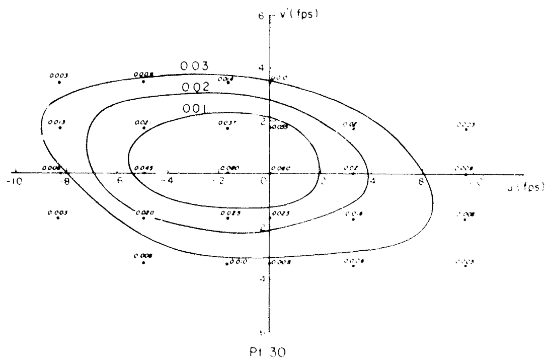
Fig. 46. Joint probability densities of u' - and v' - components at test points No. 28 and 30. (Numerical values on the contours = f(u', v') \sqrt{\overline{u'^2}} \sqrt{\overline{v'^2}} ).
