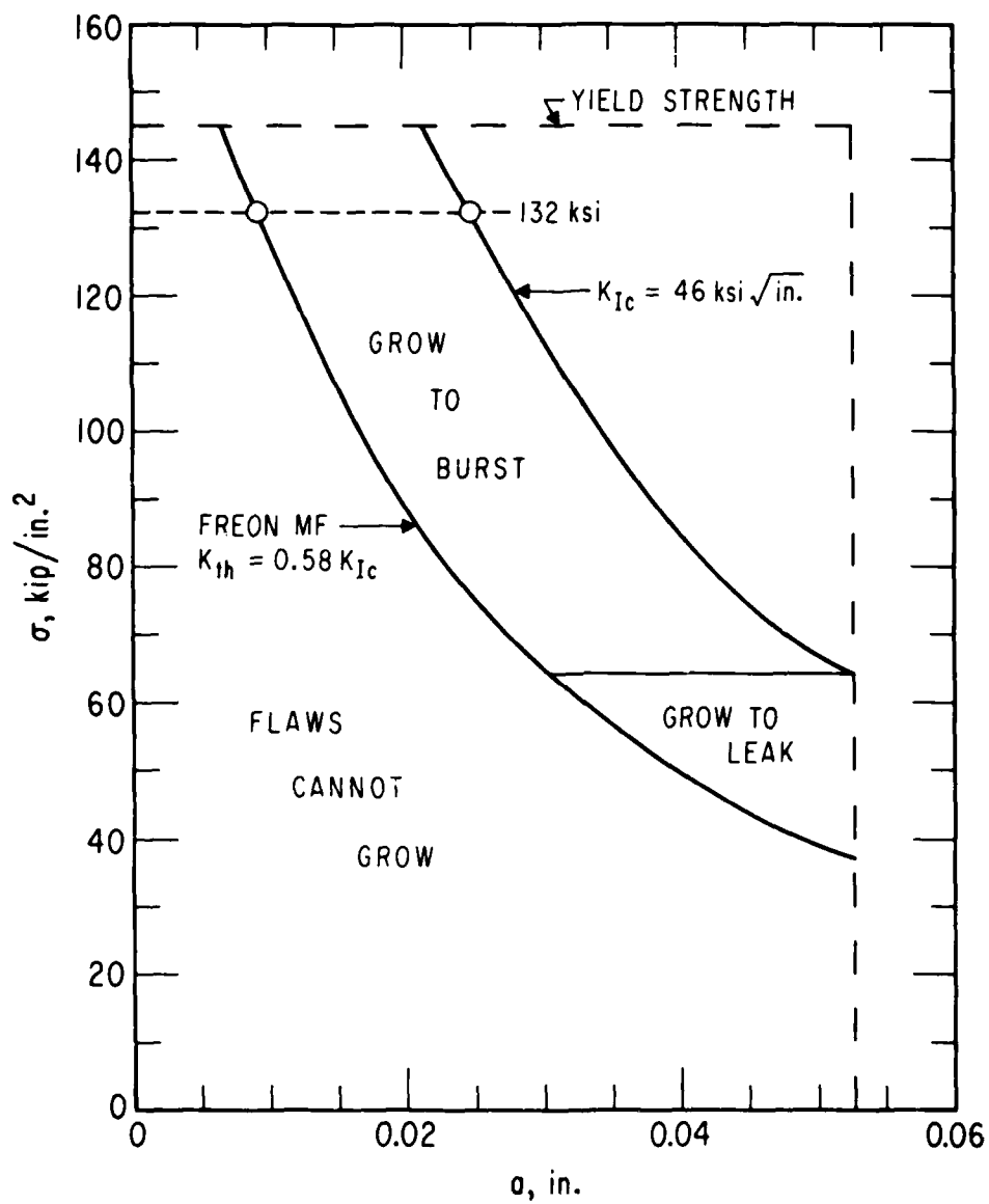
Figure 1. Effect of Environment on Flaw Detection Requirements for Ti-6Al-4V
