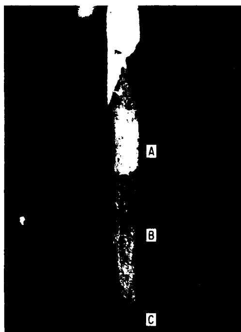
Figure 4. Fracture Surface of a Specimen Exposed to Freon MF 8X
