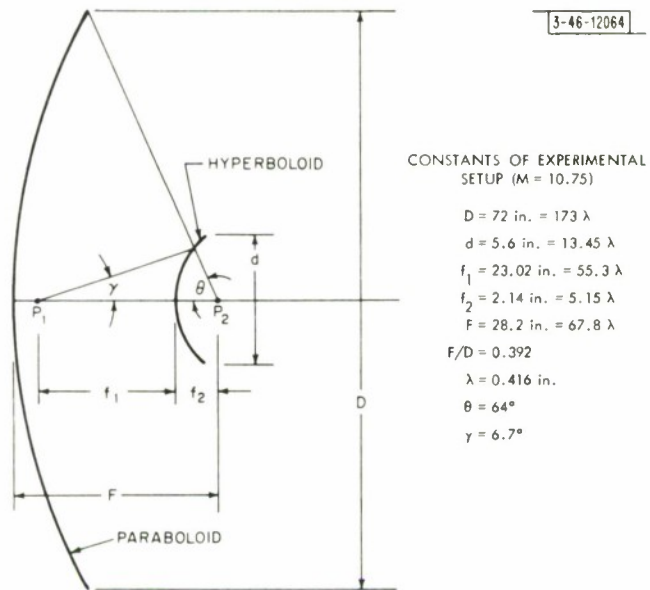
Fig. 1. Cassegrainian geometry.
