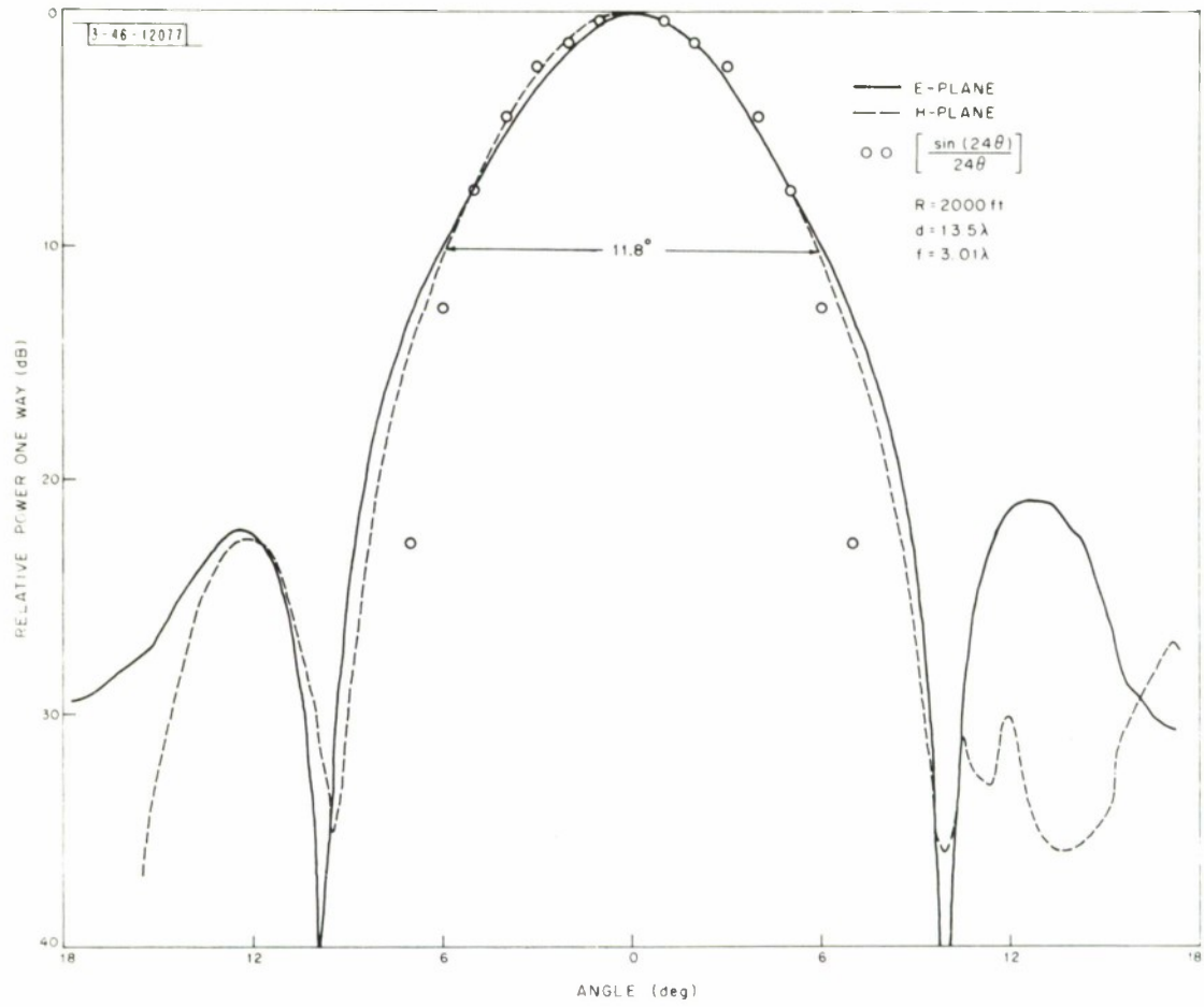
Fig. 14. Far-field radiation patterns of 13.5-λ dish with Clavin feed.
