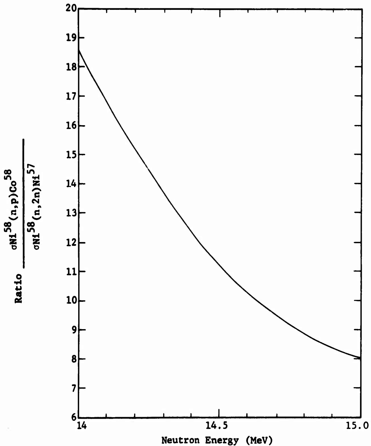
Figure 10. Energy Dependence of the Ratio of Cross Sections or Saturated Activities of \text{Ni}^{58}(n,p)\text{Co}^{58}/\text{Ni}^{58}(n,2n)\text{Ni}^{57}
