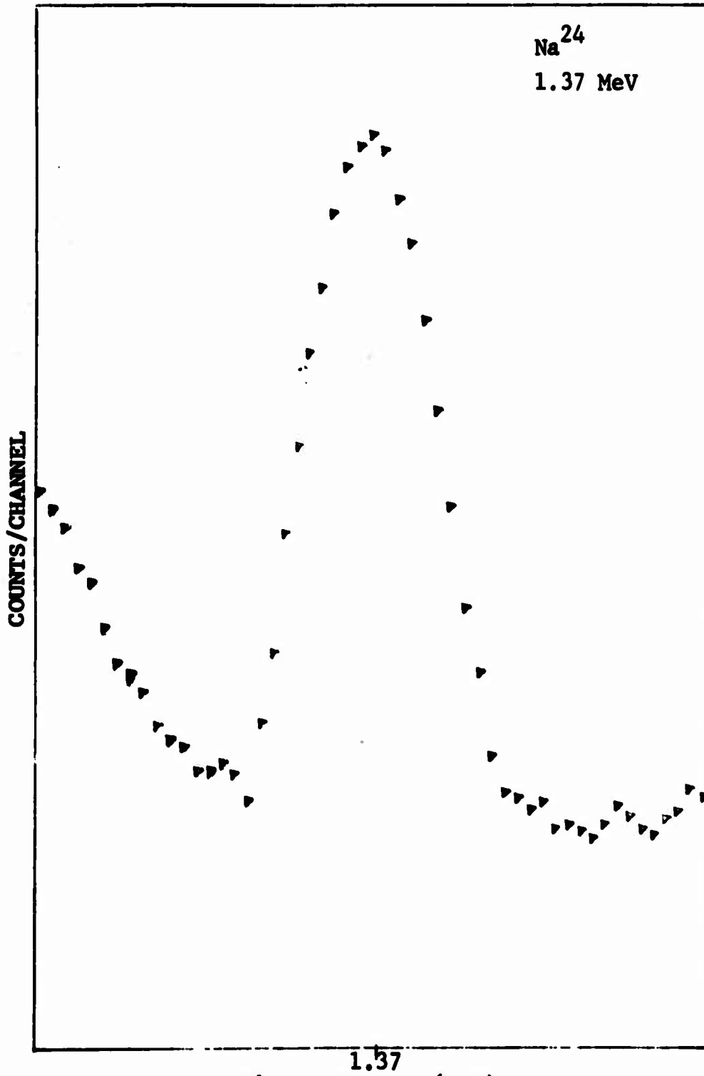
Figure 1. Typical Photopeak, 3 in. x 3 in. Foil on top of Crystal can
