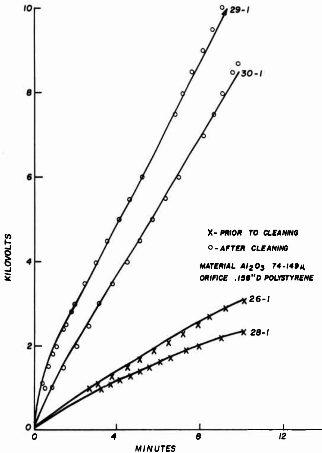
Fig 8 Curves show the effective charge buildup as a result of friction cleaning of apparatus
