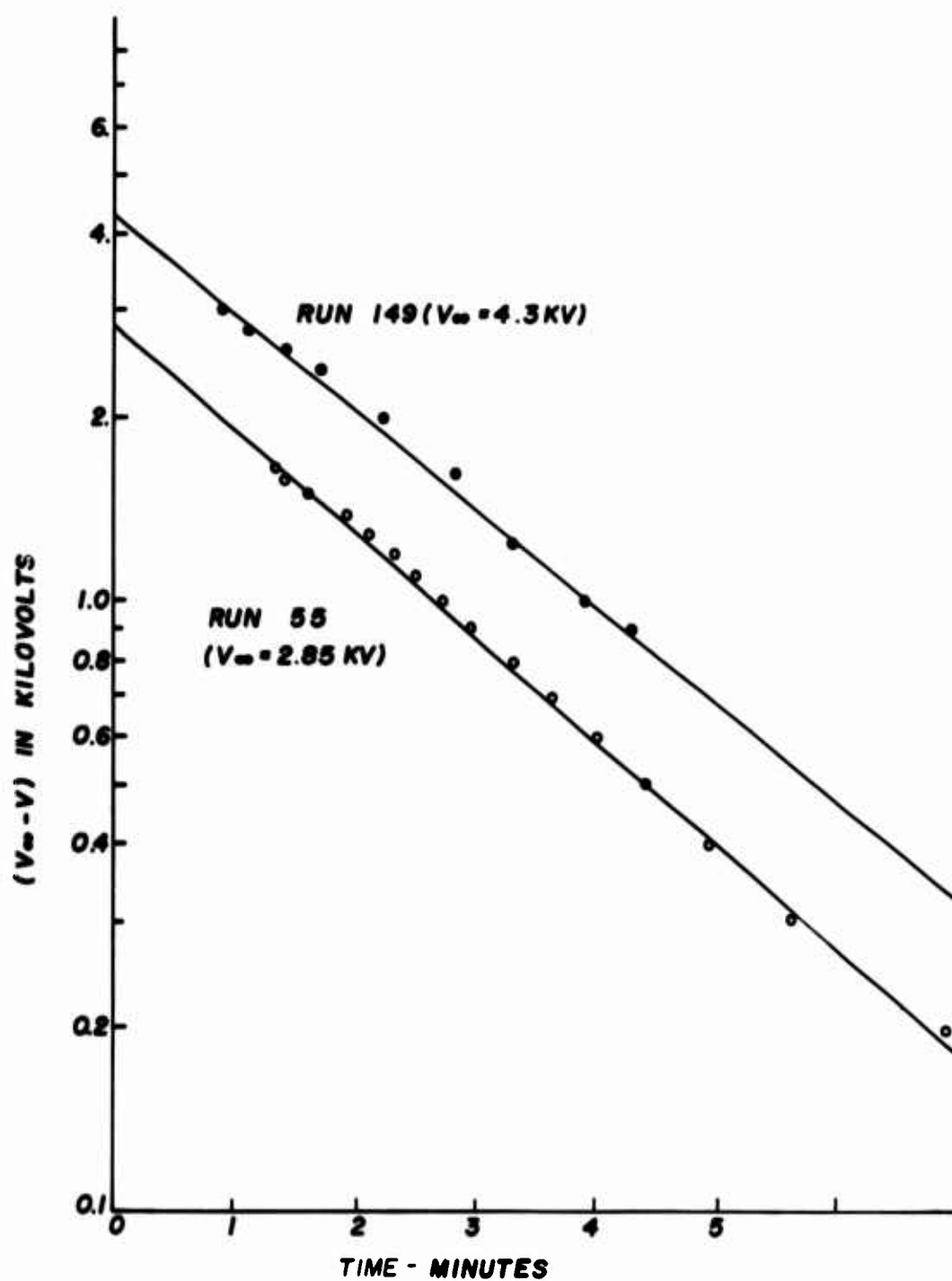
Fig 10 Charge production rate for V_{\infty} equal to 4.3 and 2.85 kv
