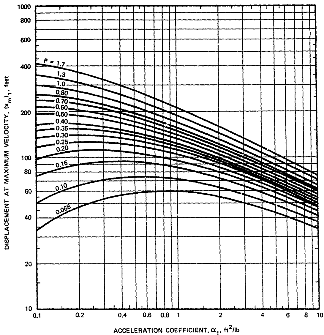
FIG. 20 PREDICTED DISPLACEMENT AT MAXIMUM VELOCITY AS A FUNCTION OF ACCELERATION COEFFICIENT AND NONDIMENSIONAL PEAK OVERPRESSURE Computed for W = 1 Mt, P_0 = 14.7 psi, and c_0 = 1117 ft/sec For other conditions, use:
