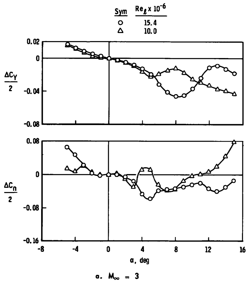
Fig. 8 Variation of \Delta C_\gamma/2 and \Delta C_n/2 with \alpha for \delta = 2 deg
