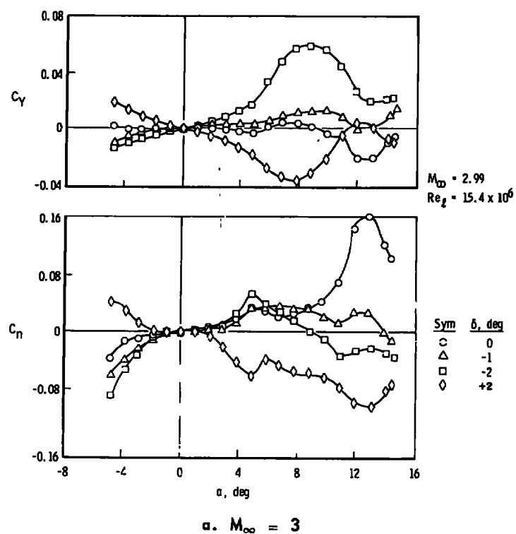
Fig. 7 Variations of C_L and C_n with \alpha for \delta = 0, -1, -2 , and 2 deg
