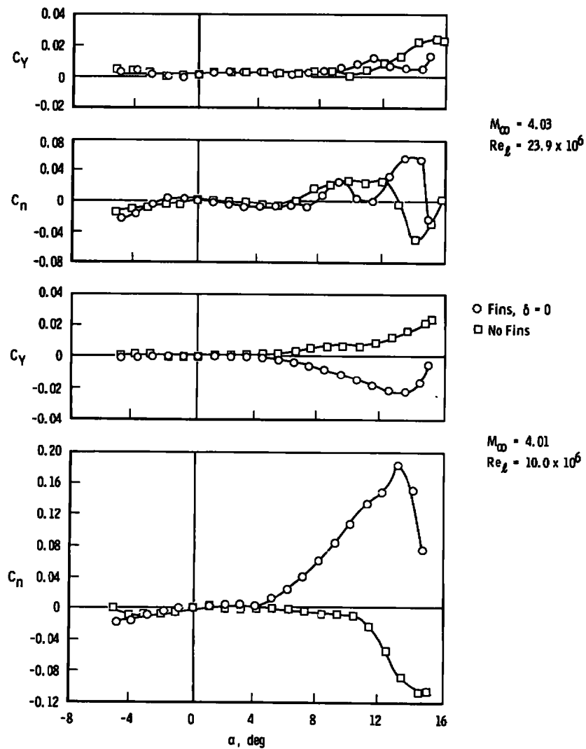
b. M_\infty = 4 Fig. 4 Continued
