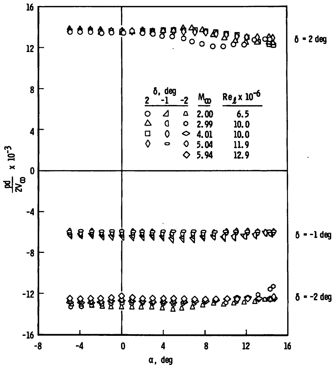
Fig. 6 Variation of Spin Parameter ( pd/2V_\infty ) with \alpha
