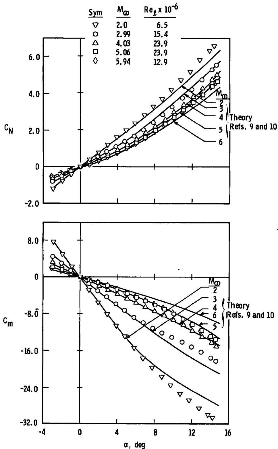
Fig. 11 C_N and C_m Variations with \alpha for Fins-On ( \delta = 0 )
