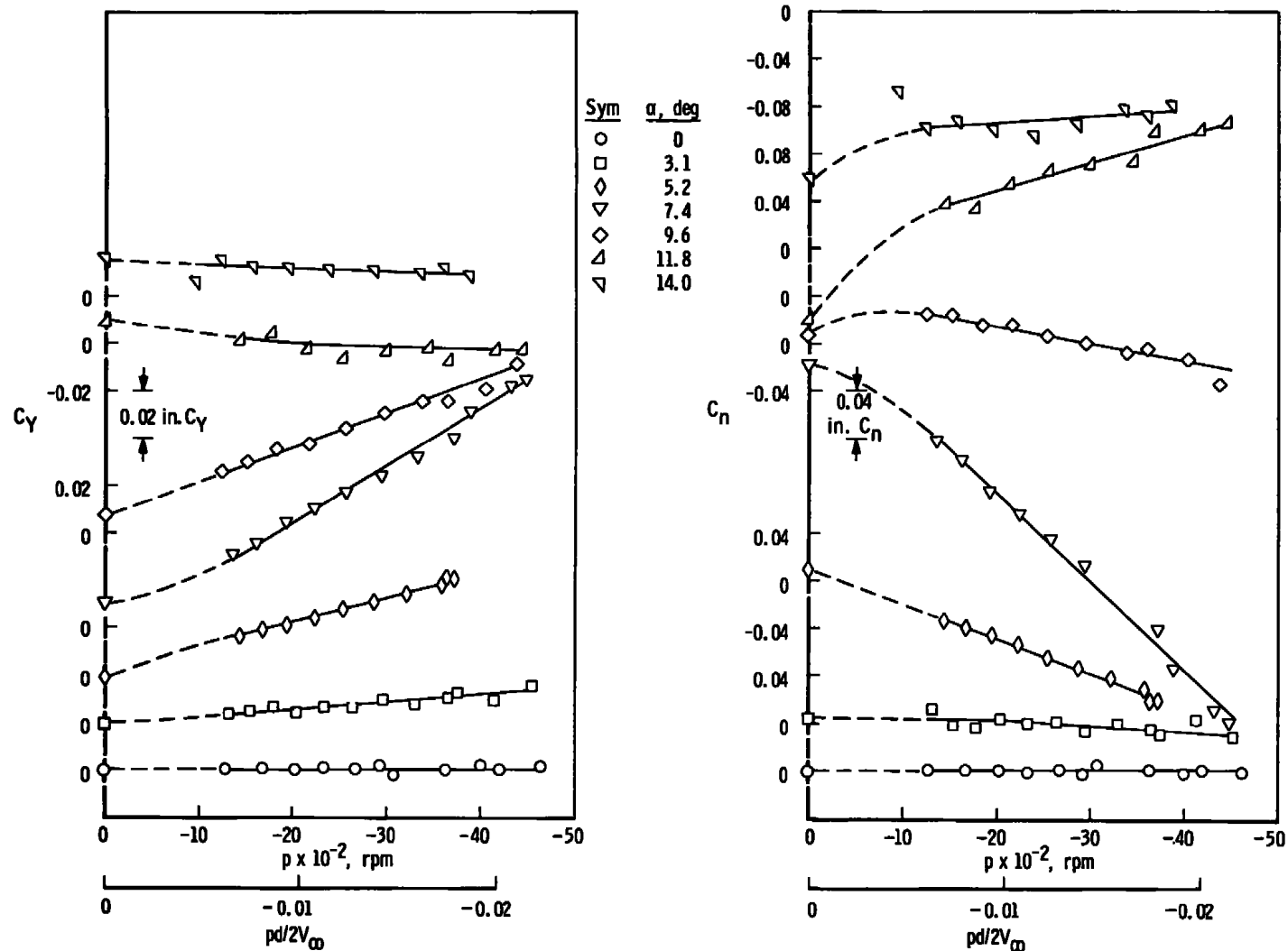
\alpha . M_\infty = 3 , Re_l = 15.4 \times 10^6 Fig. 10 Variation of C_Y and C_n with p for the Fins-Off Configuration
