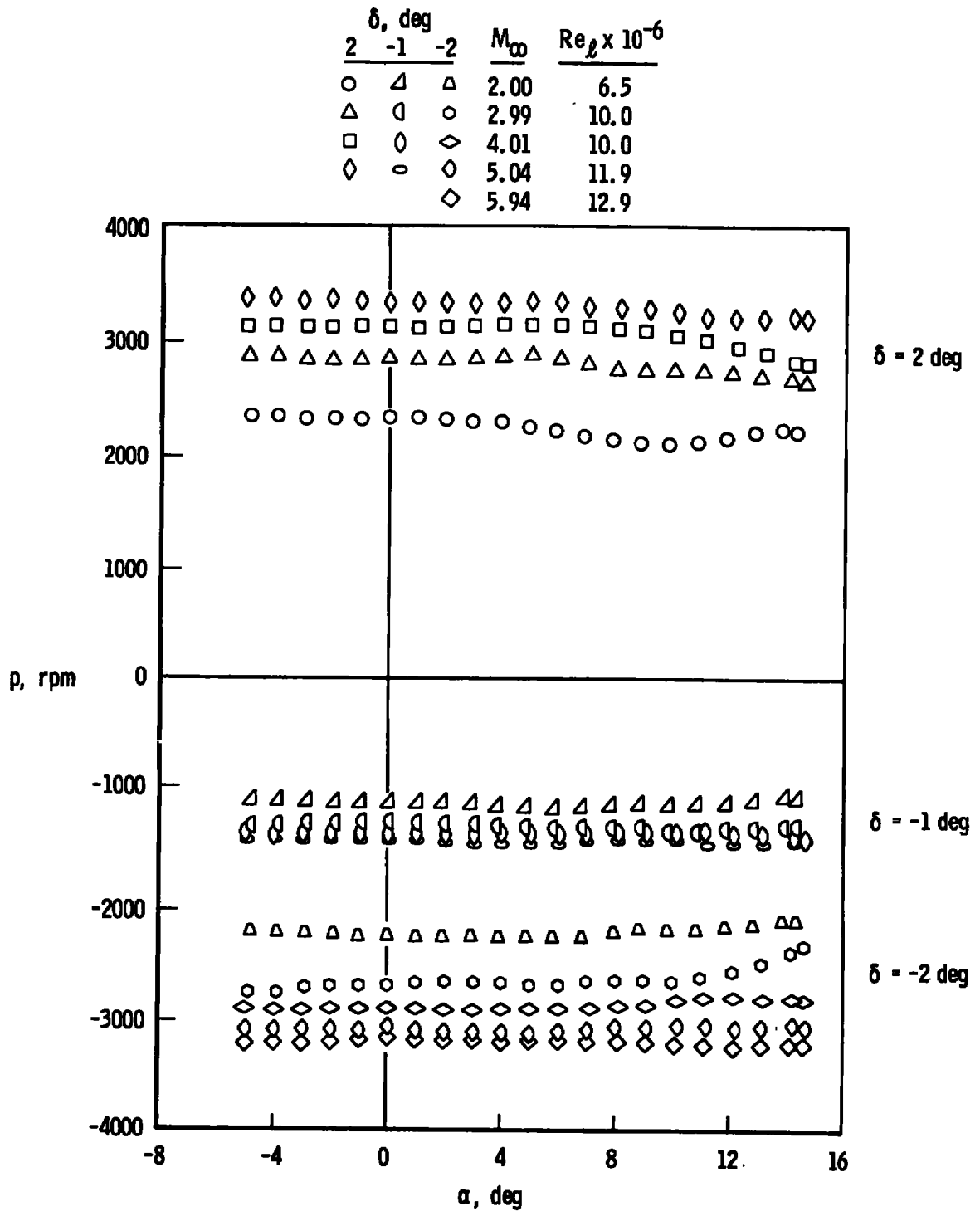
Fig. 5 Variation of Spin Rate with \alpha
