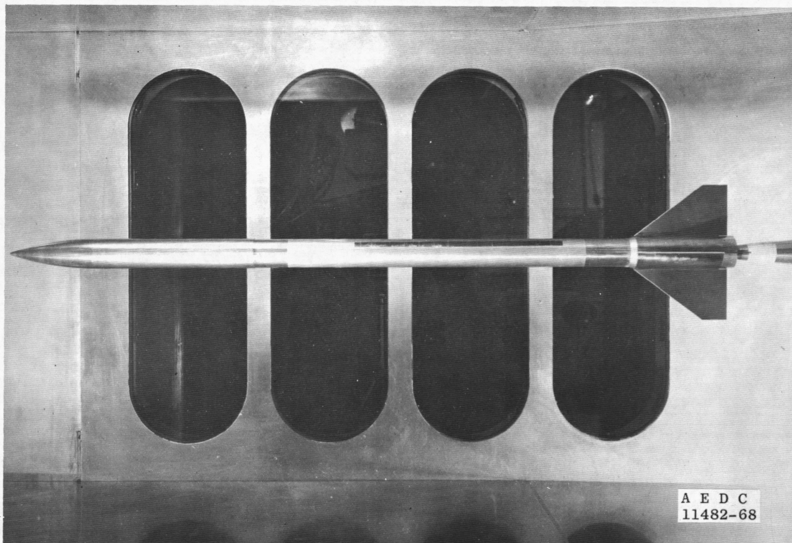
Fig. 1 Photograph of Apache Model Installed in Tunnel A
