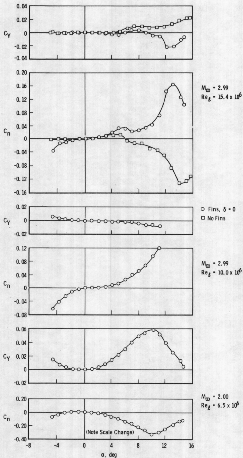
Fig. 4 Variations of C_Y and C_n with \alpha for p = 0 , Fins-On ( \delta = 0 ) and Fins-Off
