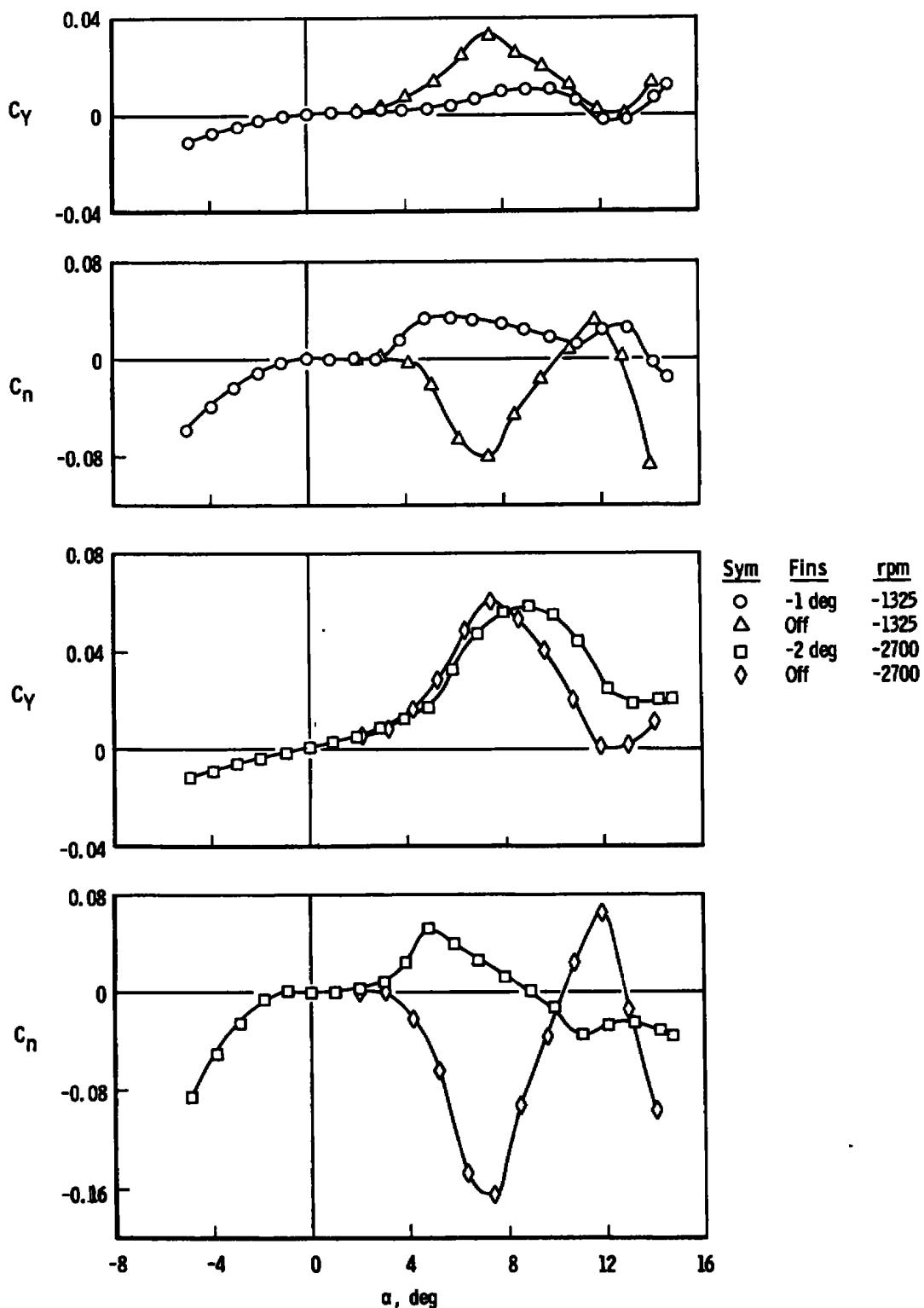
Fig. 9 Effects of Fins on the C_Y and C_n Variations with \alpha
