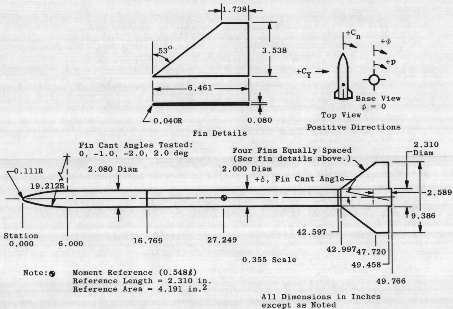
Fig. 2 Model Details
