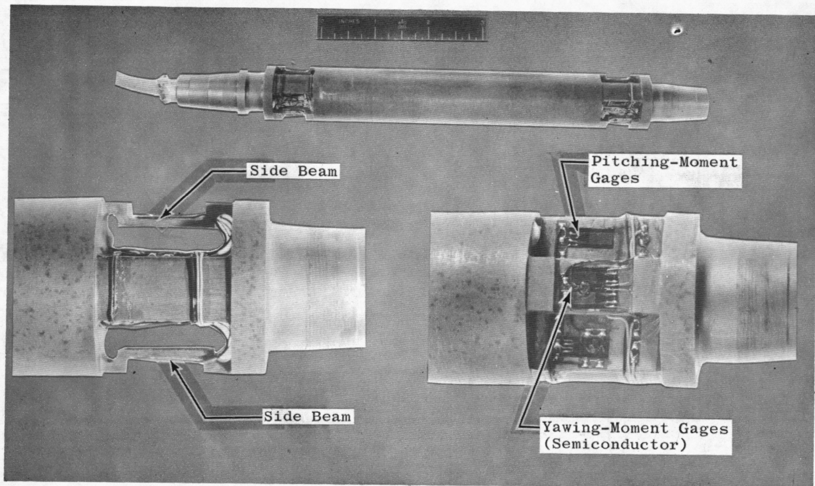
Fig. 3 Balance Details
