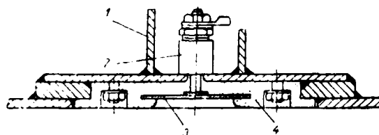
Fig. 6. Unit for Fastening the Improved Anode on the Motor Ship Svanetiya. 1 - lead-in cover; 2 - stuffing box; 3 - anode; 4 - fiberglass.
