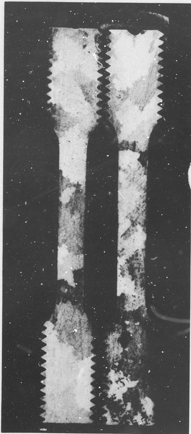
Figure 115. Vendor A Round Specimen.
