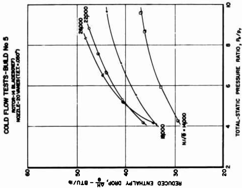
Figure 183. Build 5 - Reduced Enthalpy Drop vs Total-Static Pressure Ratio.
