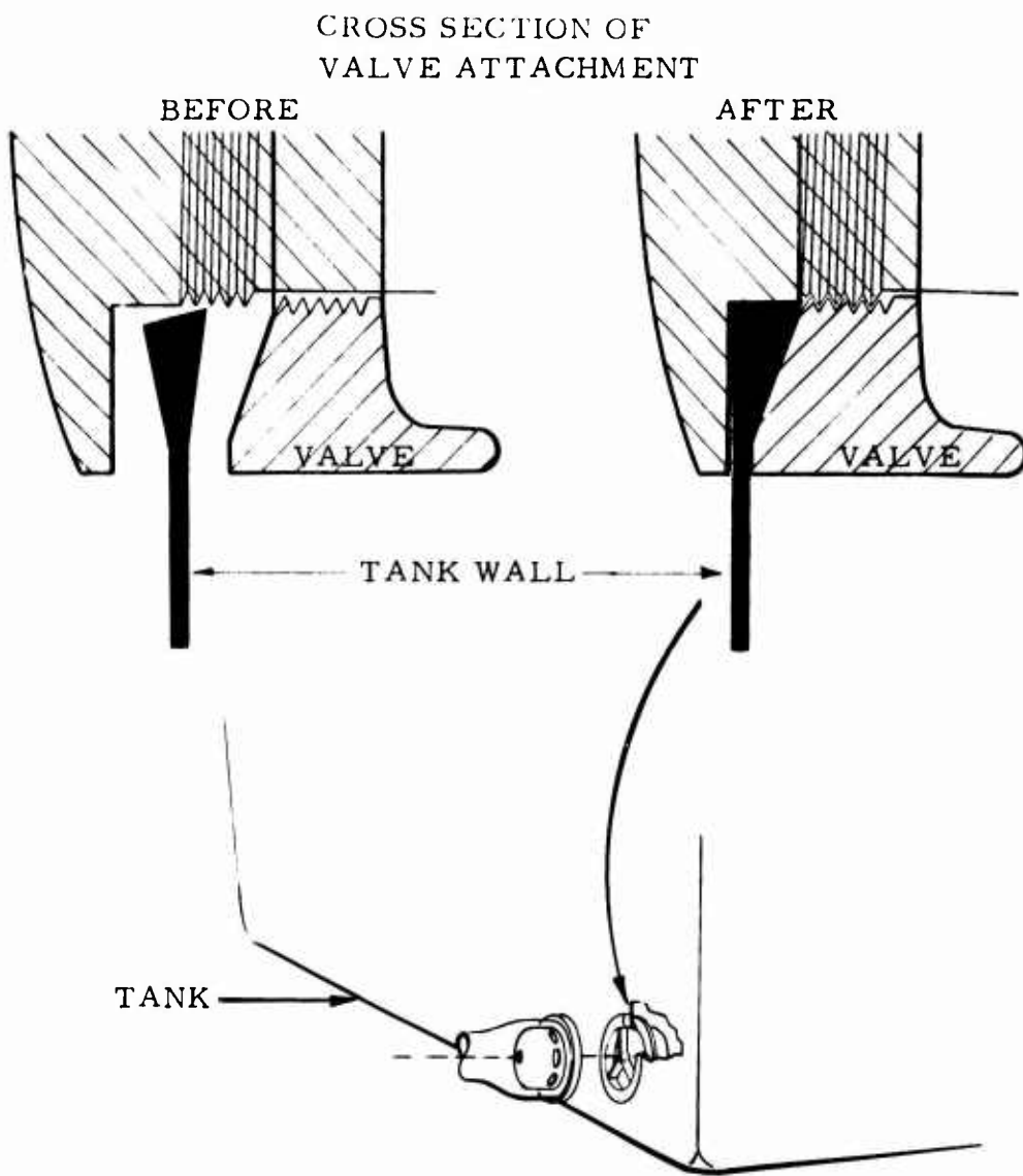
Figure 4. Wedge-Lock Retention Method.
