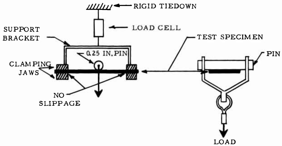
Figure 76. Bending Test.
