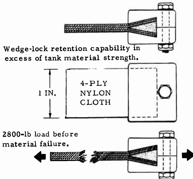
Figure 62. Wedge-Lock Fitting.
