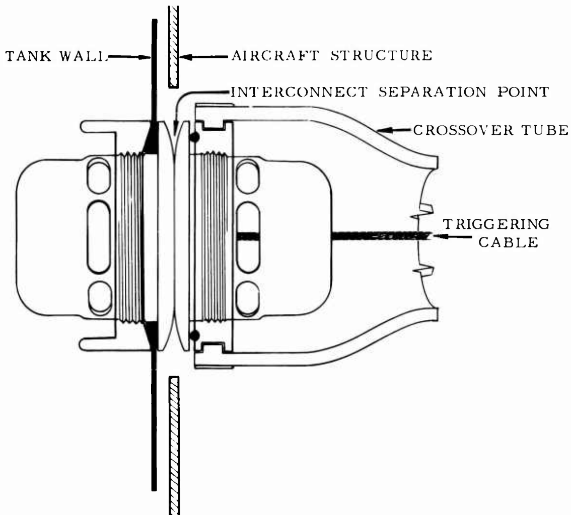
Figure 16. Type A Self-Sealing Breakaway Interconnect.
