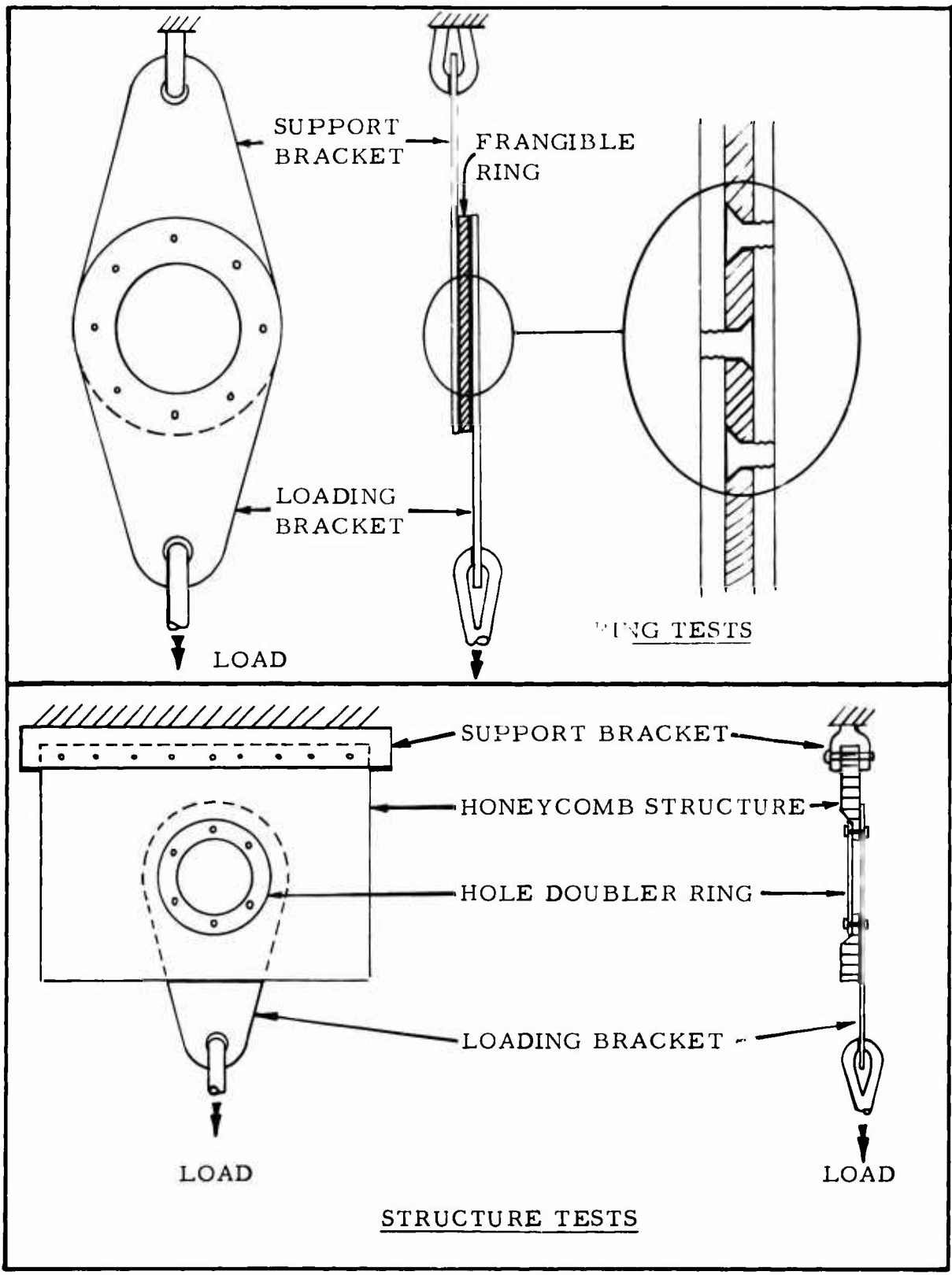
Figure 79. Shear Test.
