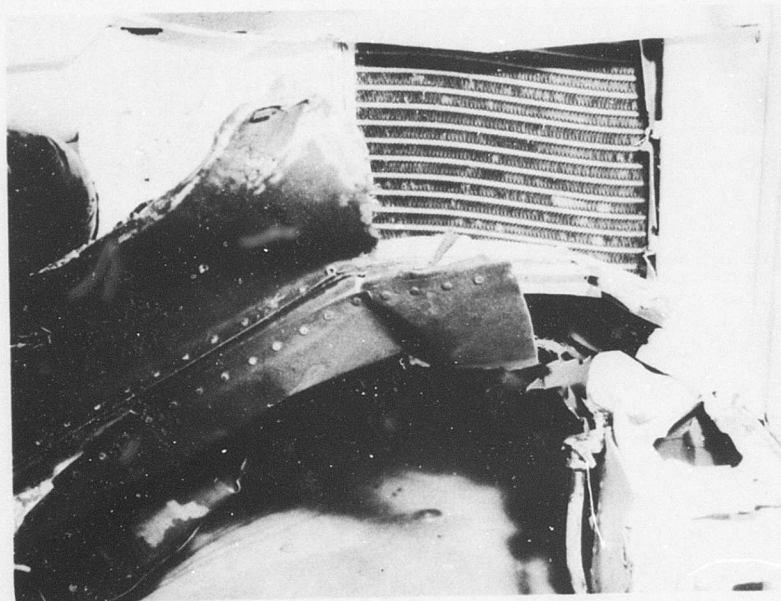
Figure 114. Posttest Front View of Oil Cooler.
