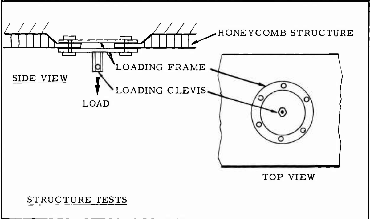
Figure 80. Tension Tests.
