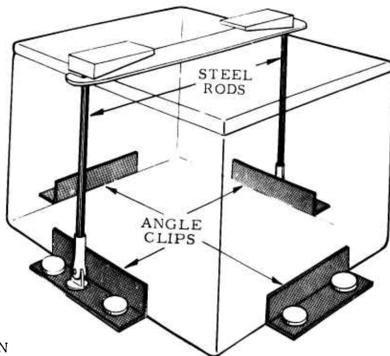
Figure 28. Battery Installation.
