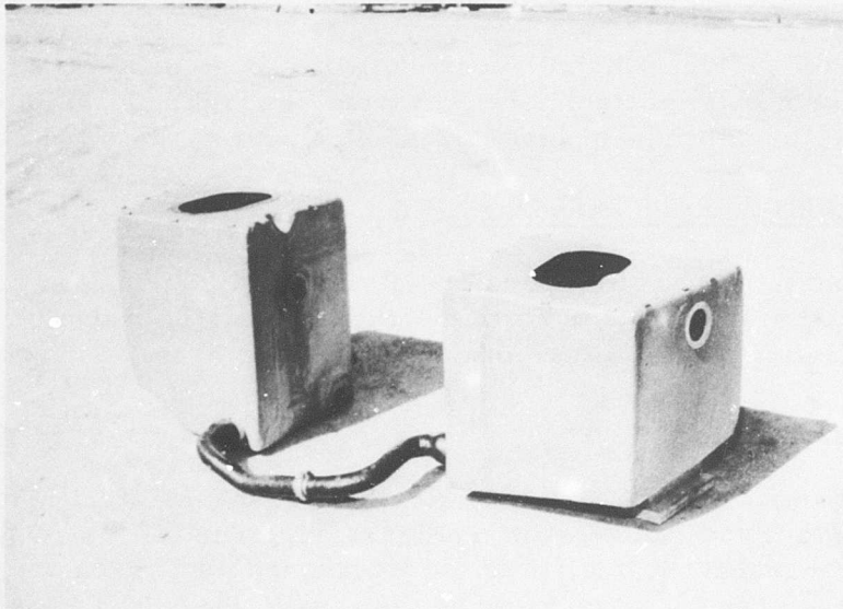
Figure 44. Tank System and Aft Crossover Assembly Reassembled After Test.
