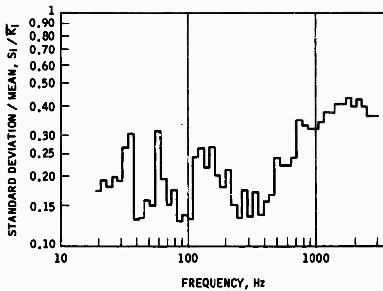
FIGURE 5 Ratio of Standard Deviation of Severity Factor to Mean Severity Factor - Accelerometer 36
