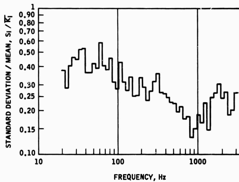
FIGURE 6 Ratio of Standard Deviation of Severity Factor to Mean Severity Factor using Modified Severity Factor ( K' = K/M ) - Accelerometer 36
