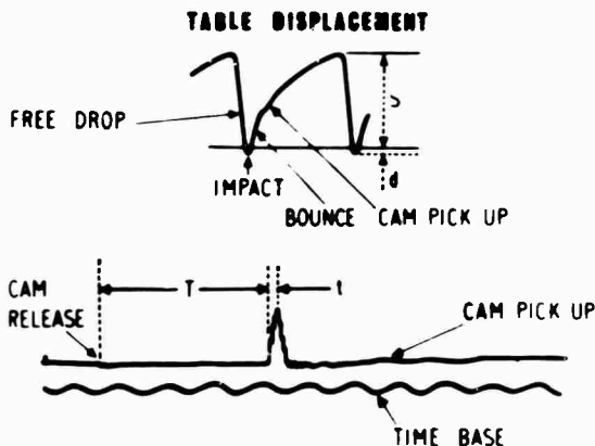
FIGURE 3. ACCELEROMETER RESPONSE
