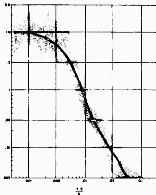
Figure 24 - RMS pressure and nondimensional pressure spectra for the microphones at the missile fuselage
