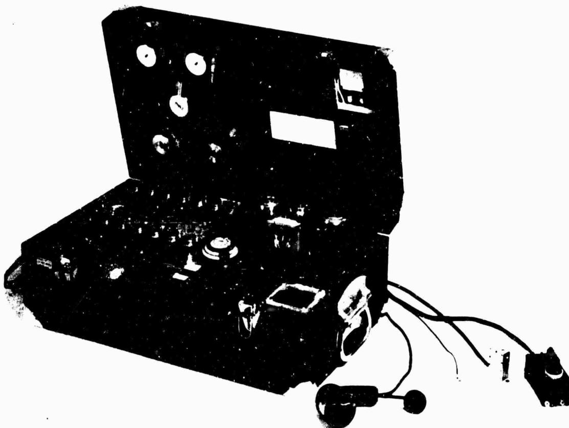
Fig. 4 - ELI 31 portable environmental sampler
