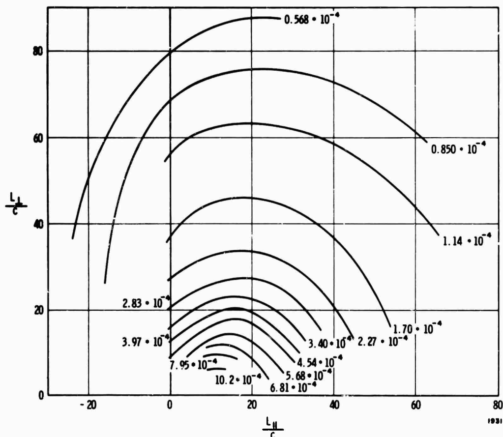
Fig. 4 - Isoclines of side-on pressure, \frac{Pc^2 I}{W}
