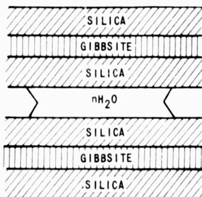
Figure H-2 MONTMORILLONITE SHOWN SCHEMATICALLY
