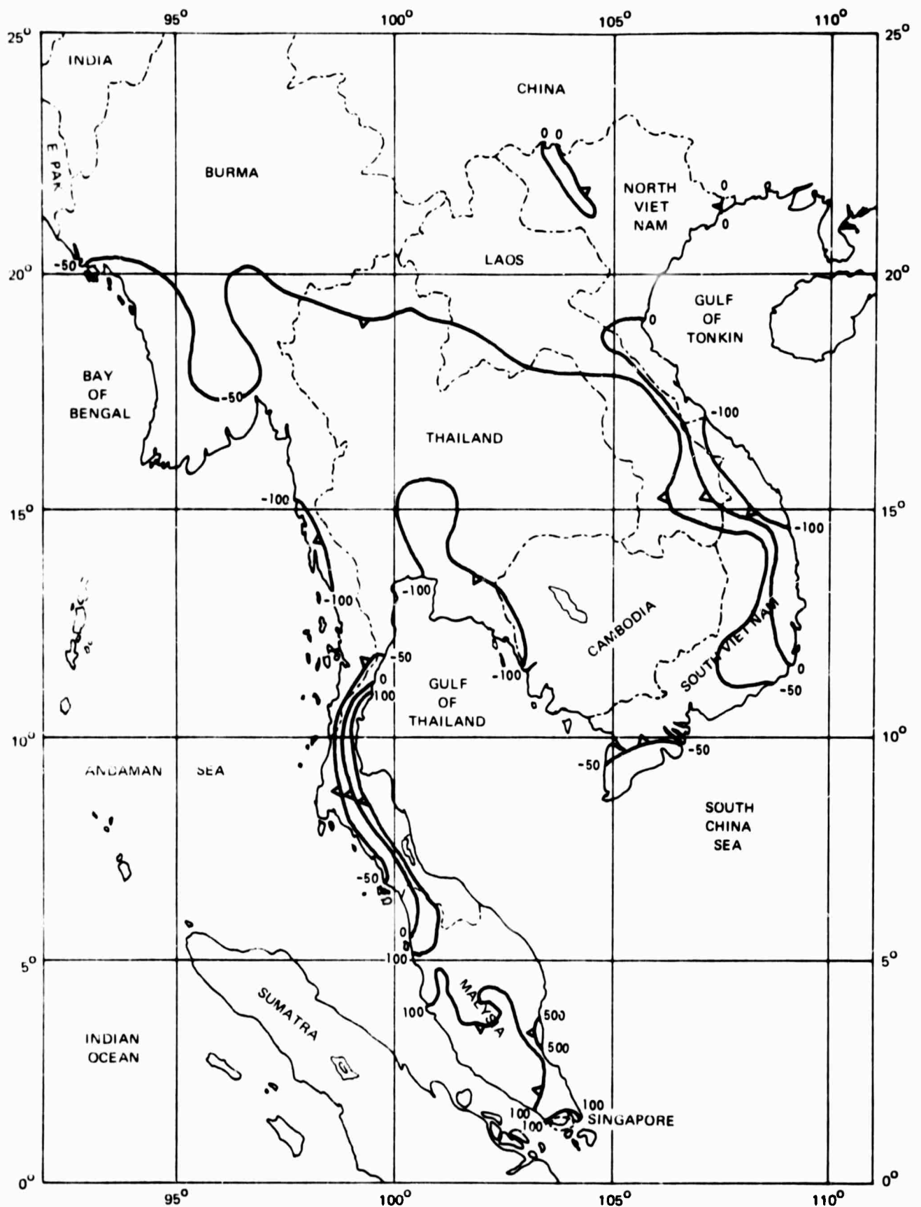
Figure D-1(i) PRECIPITATION MINUS POTENTIAL EVAPOTRANSPIRATION IN MILLIMETERS - DECEMBER
