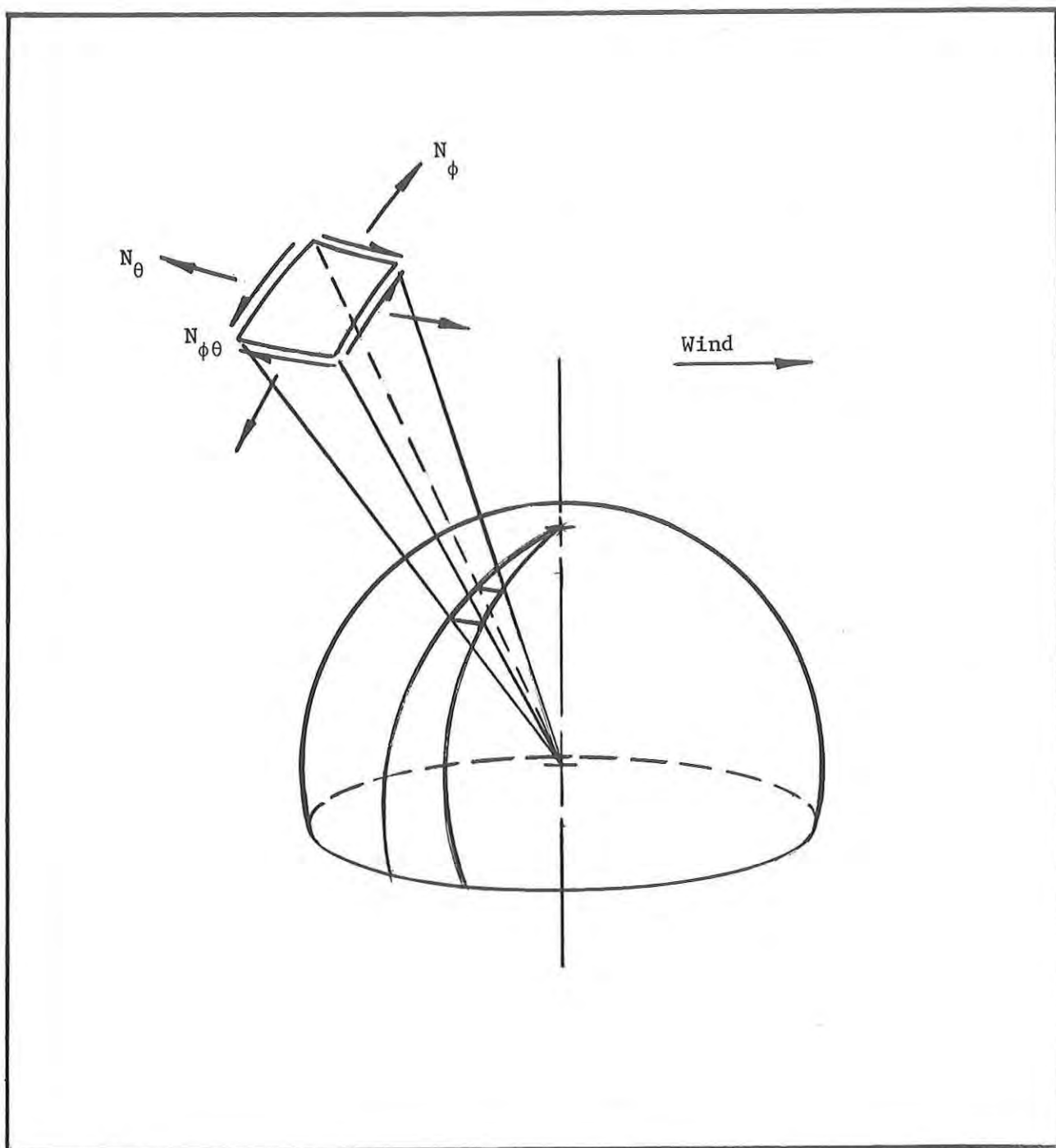
Figure 25. Coordinate System and Membrane Stresses for a Truncated Spherical Shell
