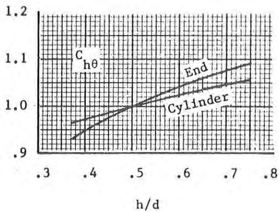
Figure 34. Correction Factors for Single-Wall Cylindrical Tents with Ellipsoidal Ends; \theta
