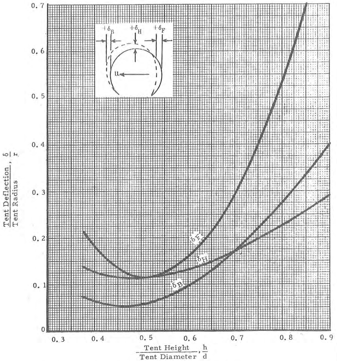
Figure 17. Variation of Tent Deflection with Shape (Non-Porous Cylindrical Single-Wall Tents, 1:4 W/\ell_h )
