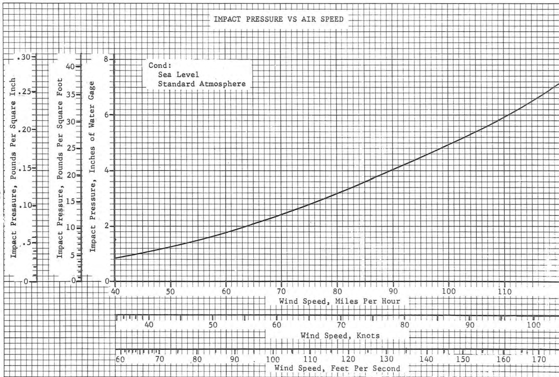
Figure 7. Variation of Impact Pressure with Air Speed, Sea Level Standard Atmosphere.
