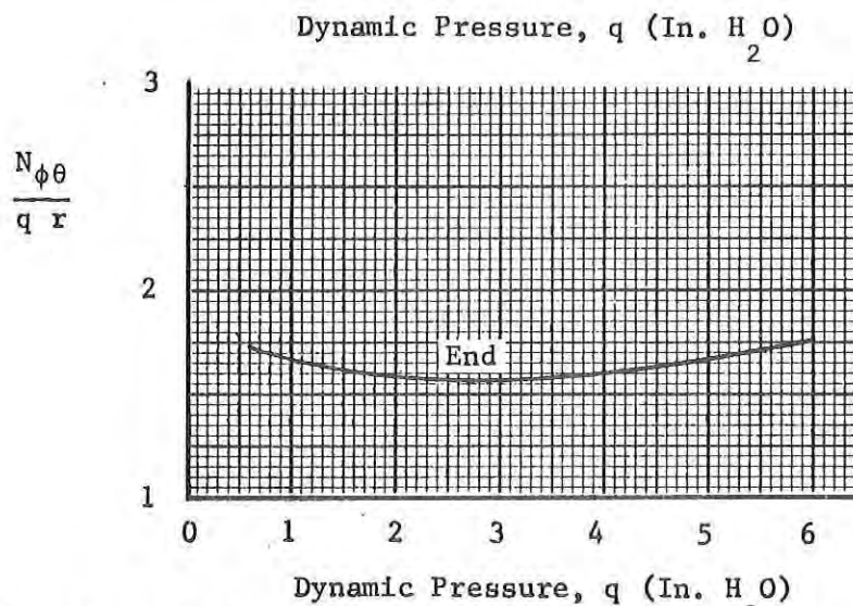
Figure 32. Basic Maximum Stress Coefficients for Single-Wall Cylindrical Tents with Ellipsoidal Ends
