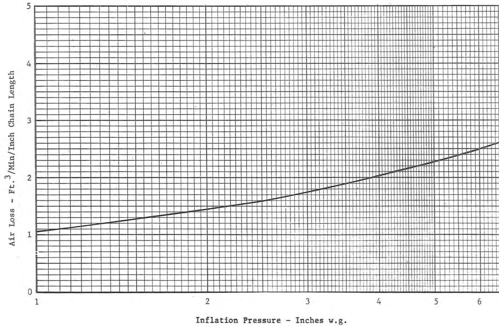
Figure 51. Air Loss through a #10 Crown Slide Fastener
