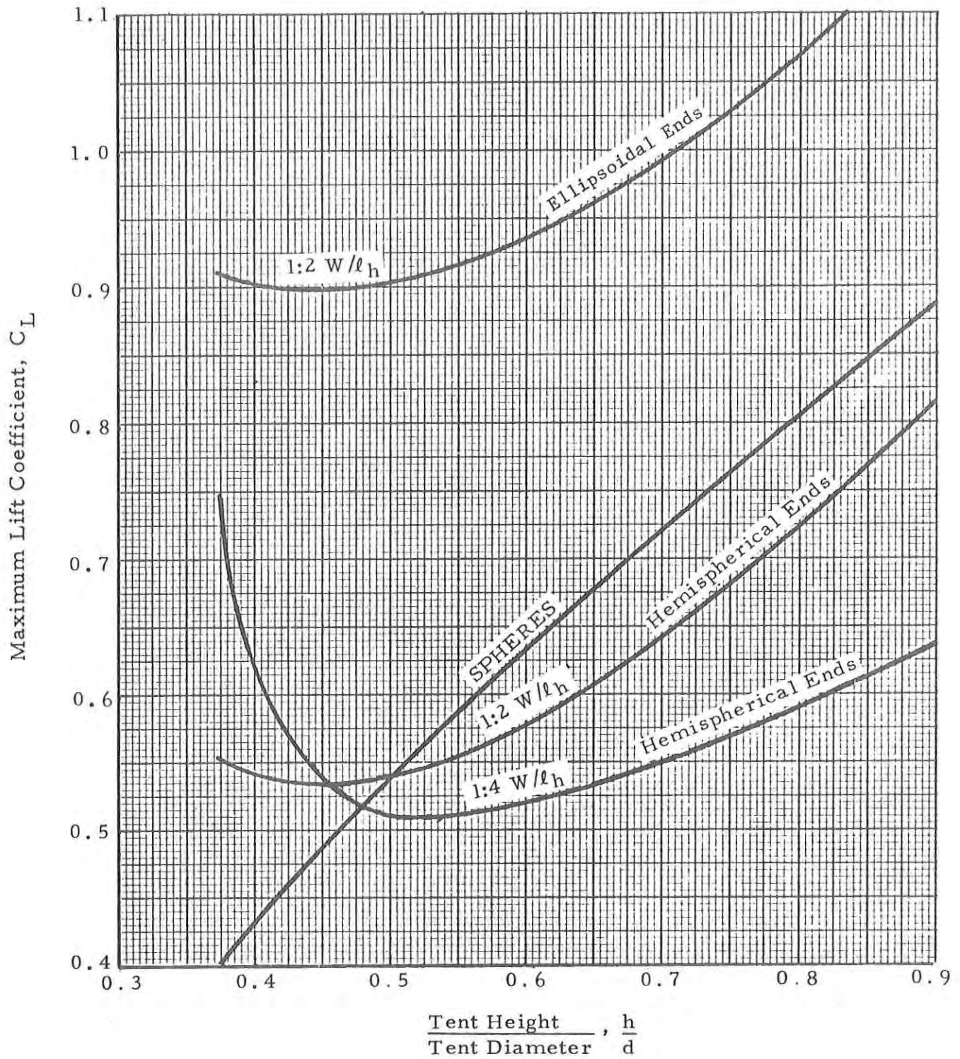
Figure 9. - Variation of Lift Coefficient with Shape (Non-Porous Spherical and Cylindrical Single-Wall Tents; 1:2, 1:4, W/l_h )
