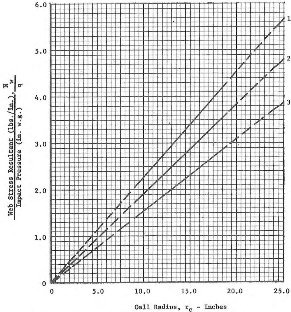
Figure 38. Variation of Web Stress Coefficient with Cell Radius.
