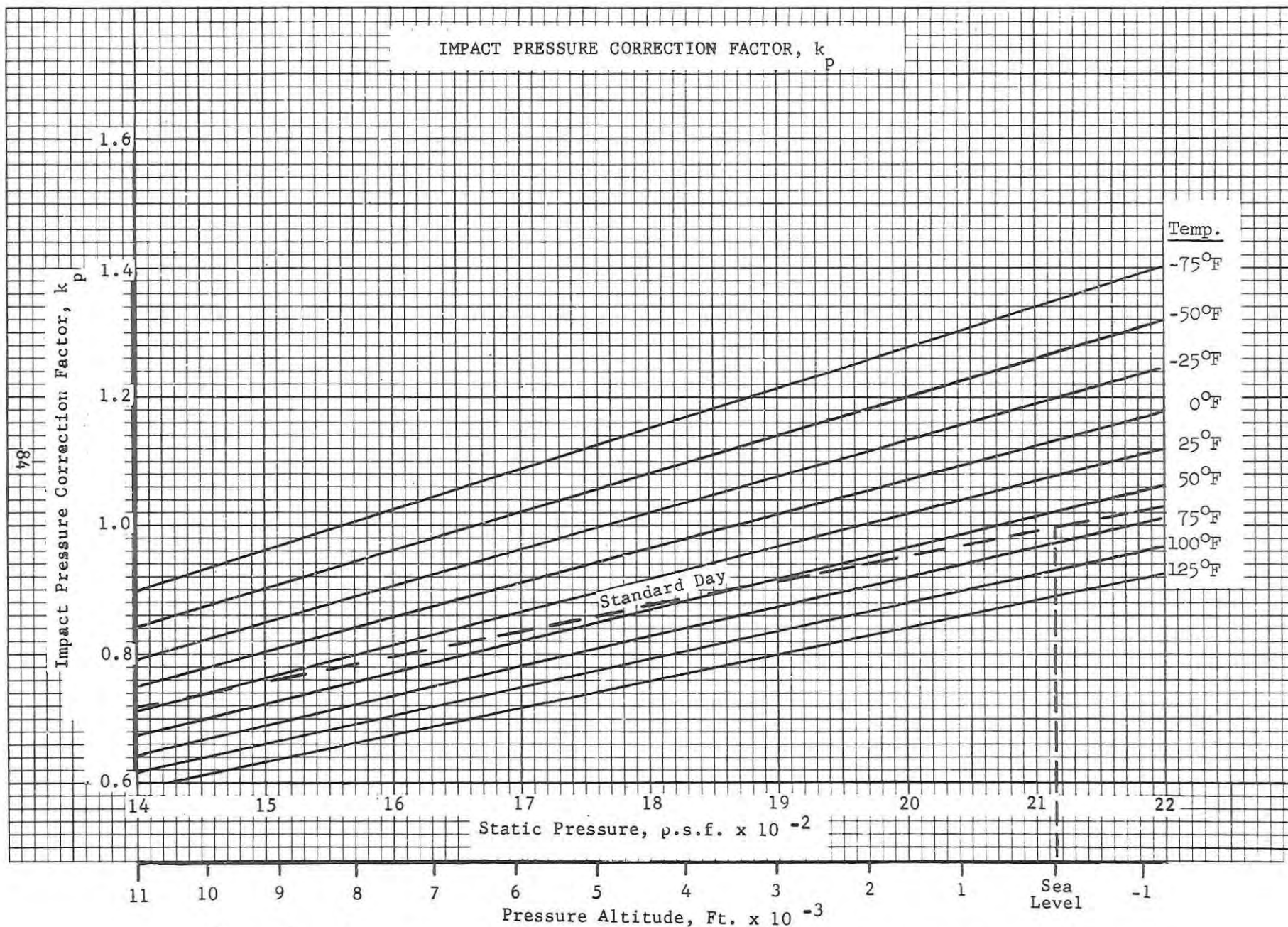
Figure 8. Impact Pressure Correction Factor, k_p , Variation With Altitude & Temperature
