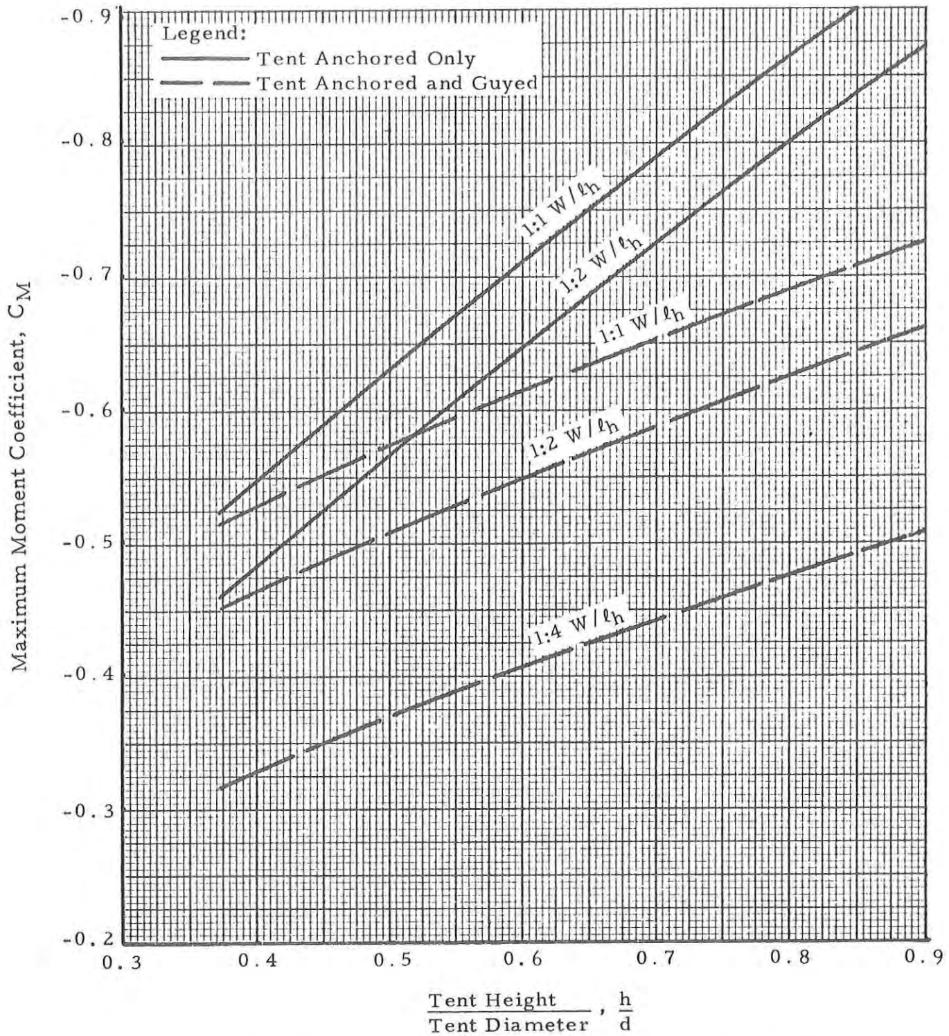
Figure 14. Variation of Moment Coefficient with Shape (Non-Porous Double-Wall Tents; 1:1, 1:2, 1:4 W/\ell_h )
