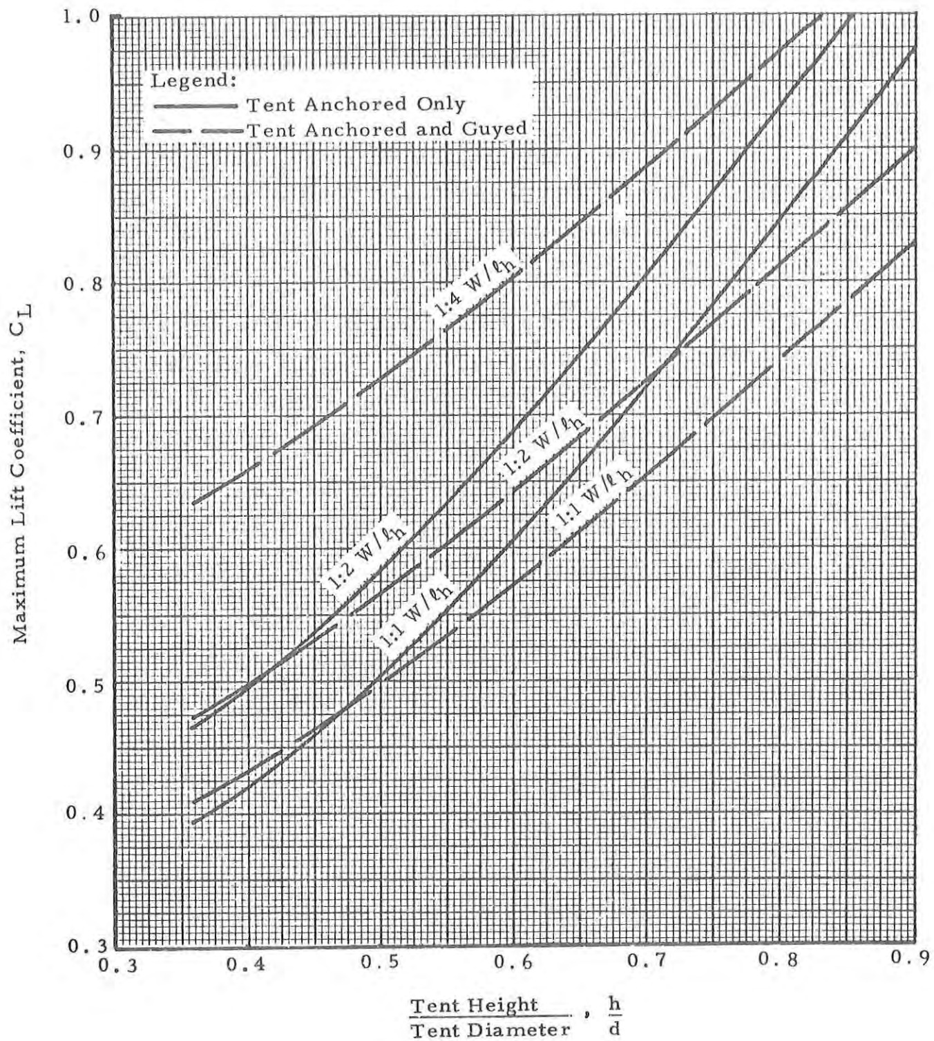
Figure 10. Variation of Lift Coefficient With Shape (Non-Porous Double-Wall Tents; 1:1, 1:2, 1:4 W/l_h )
