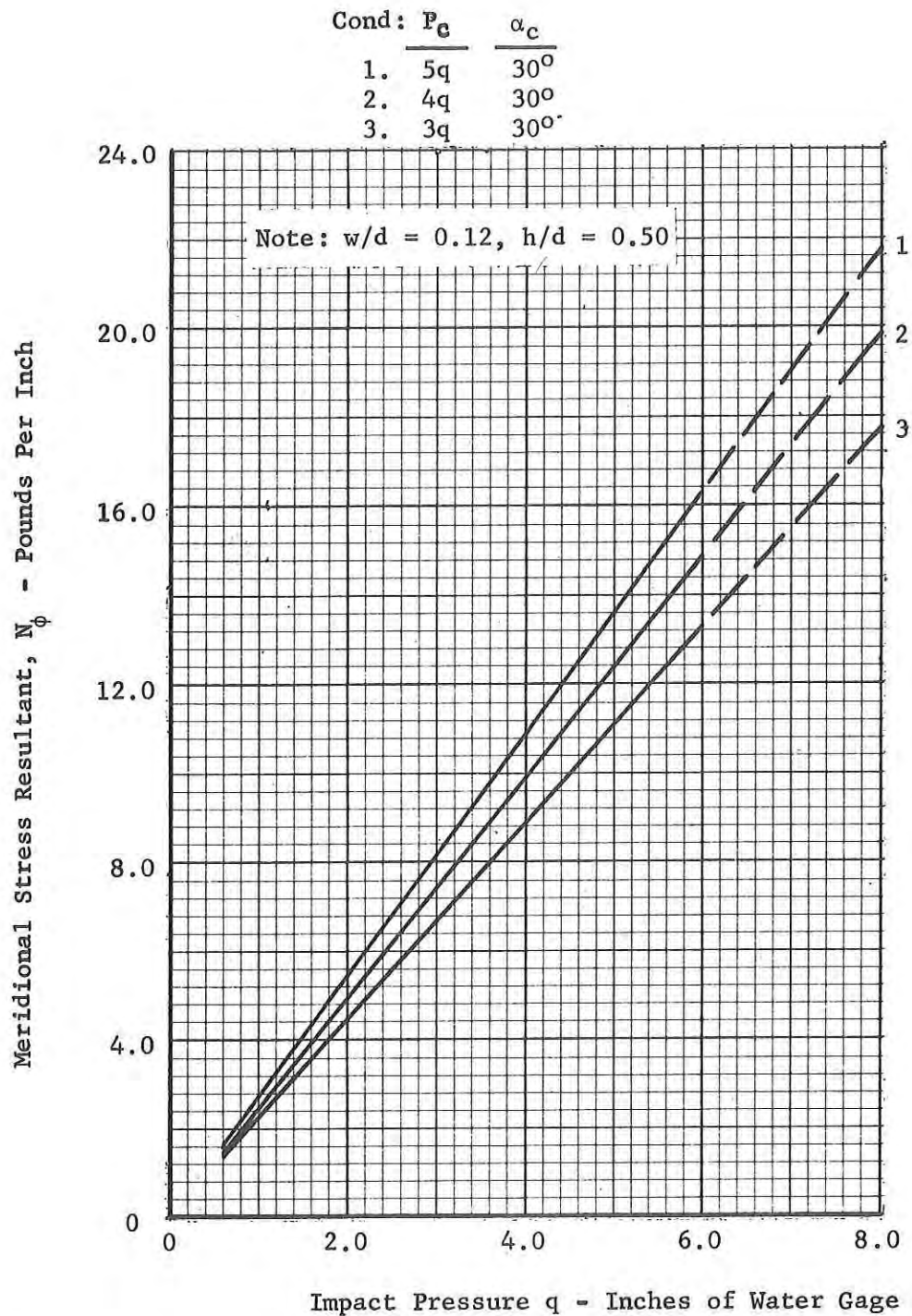
Figure 41. Variation of Meridional Stress Resultant with Impact Pressure, q ; w/d = 0.12 , h/d = 0.50
