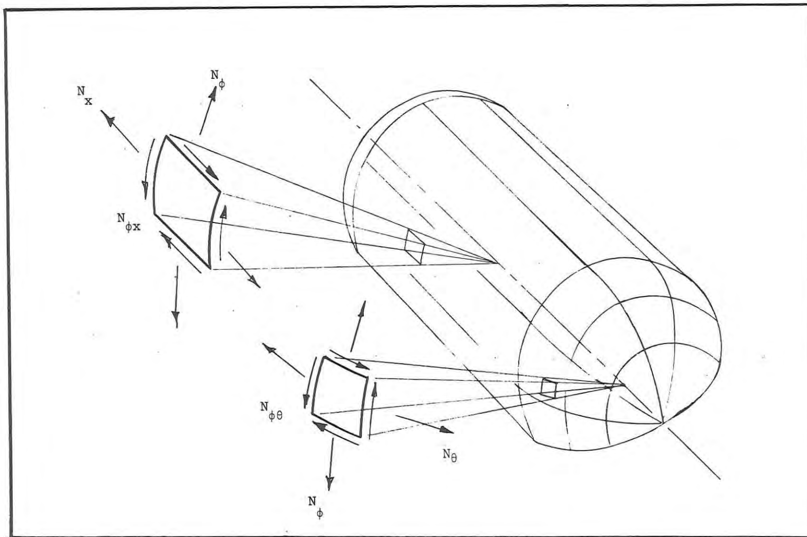
Figure 36. Coordinate System and Membrane Stresses for a Cylindrical Shell with Ellipsoidal Ends
