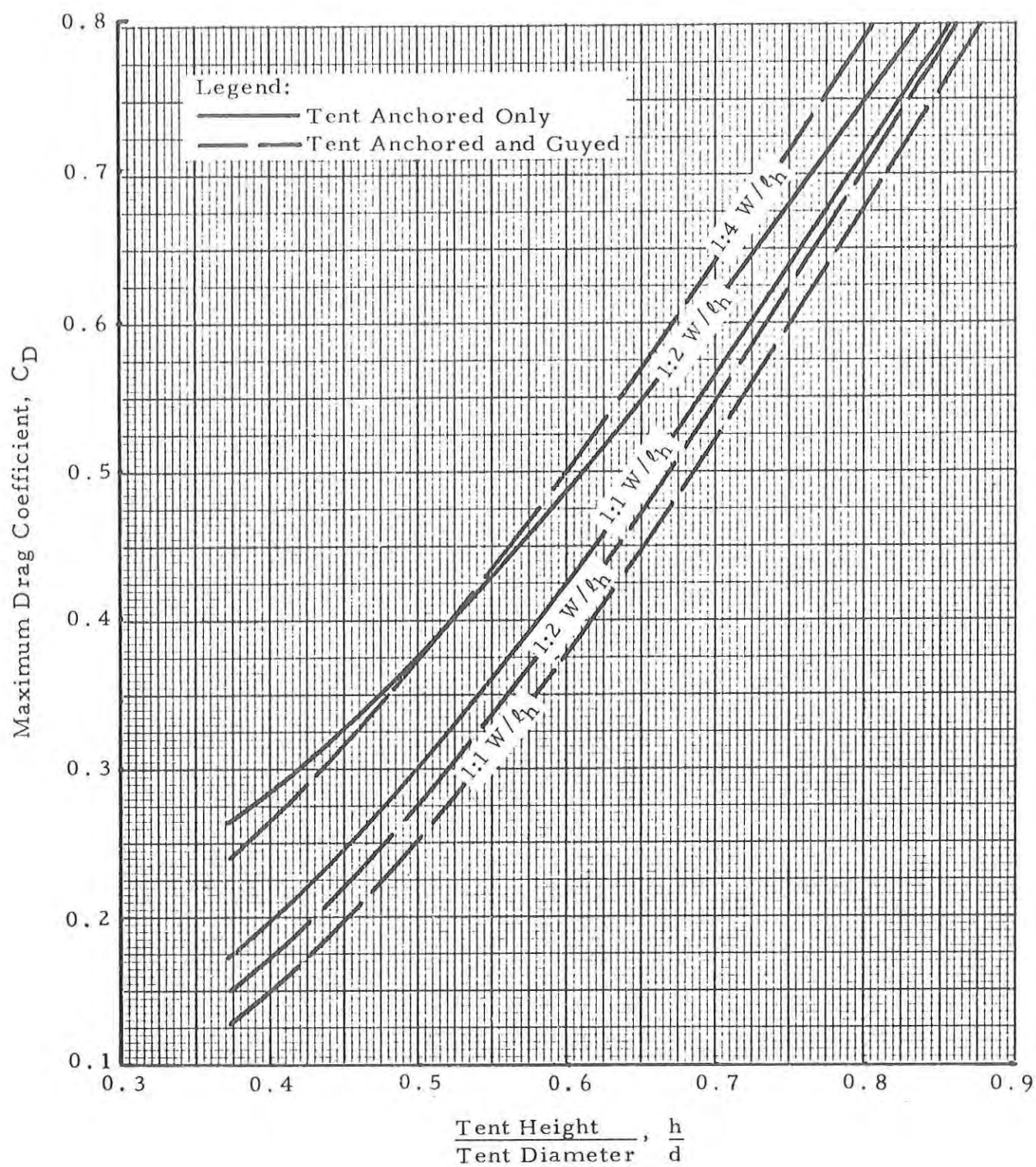
Figure 12. Variation of Drag Coefficient with Shape (Non-Porous Double-Wall Tents; 1:1, 1:2, 1:4 W/\ell_h )
