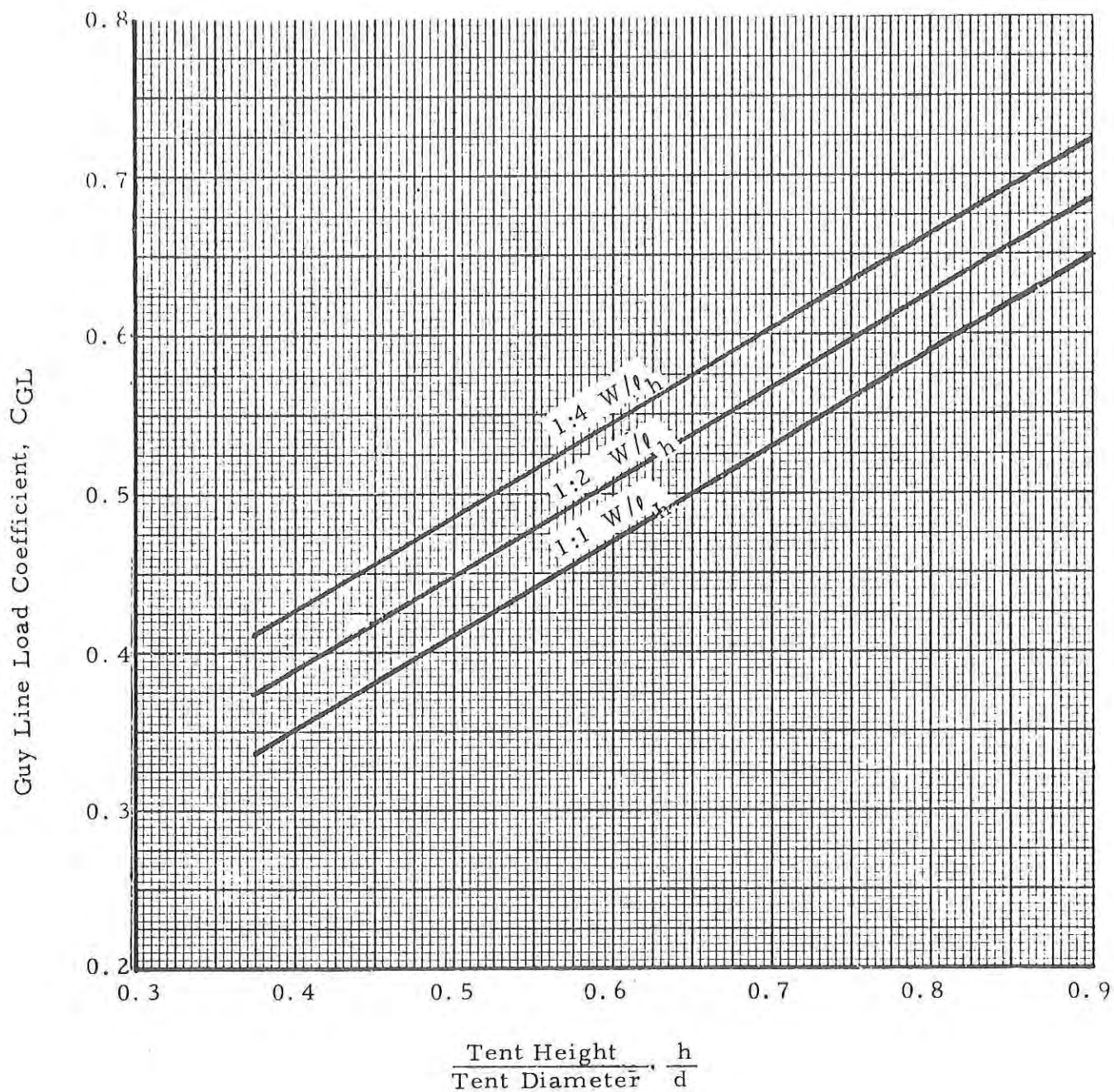
Figure 22. Variation of Guy Line Load Coefficient With Shape.
