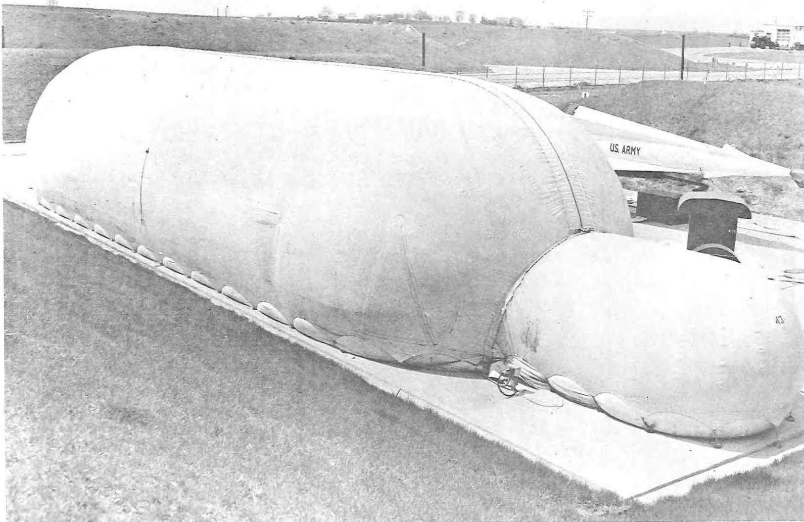
Figure 2. Single-Wall, Air-Supported Tent, Above-Ground, Launcher, Nike Hercules System.
