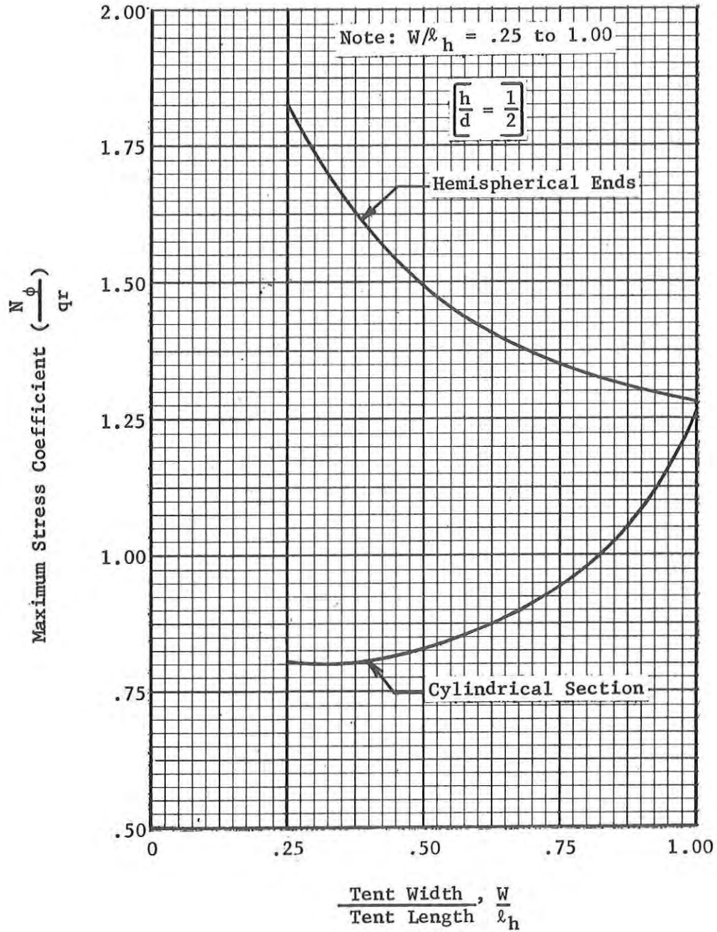
Figure 27. Variation of Maximum Design Stress Coefficient With Tent Width-to-Length Ratio; n/d = 1/2 , N_\phi/qr
