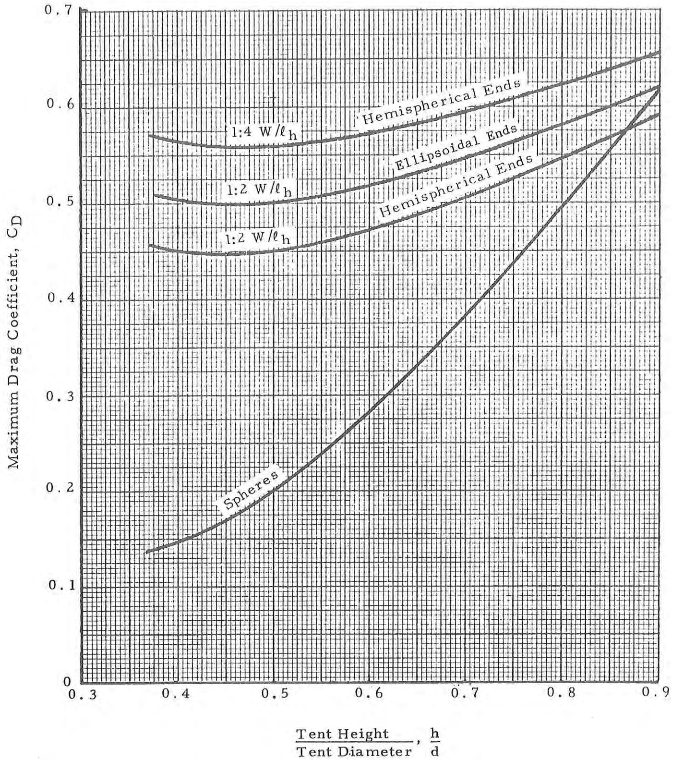
Figure 11. Variation of Drag Coefficient With Shape (Spherical and Cylindrical Single-Wall Tents; 1:2, 1:4 W/\ell_h )
