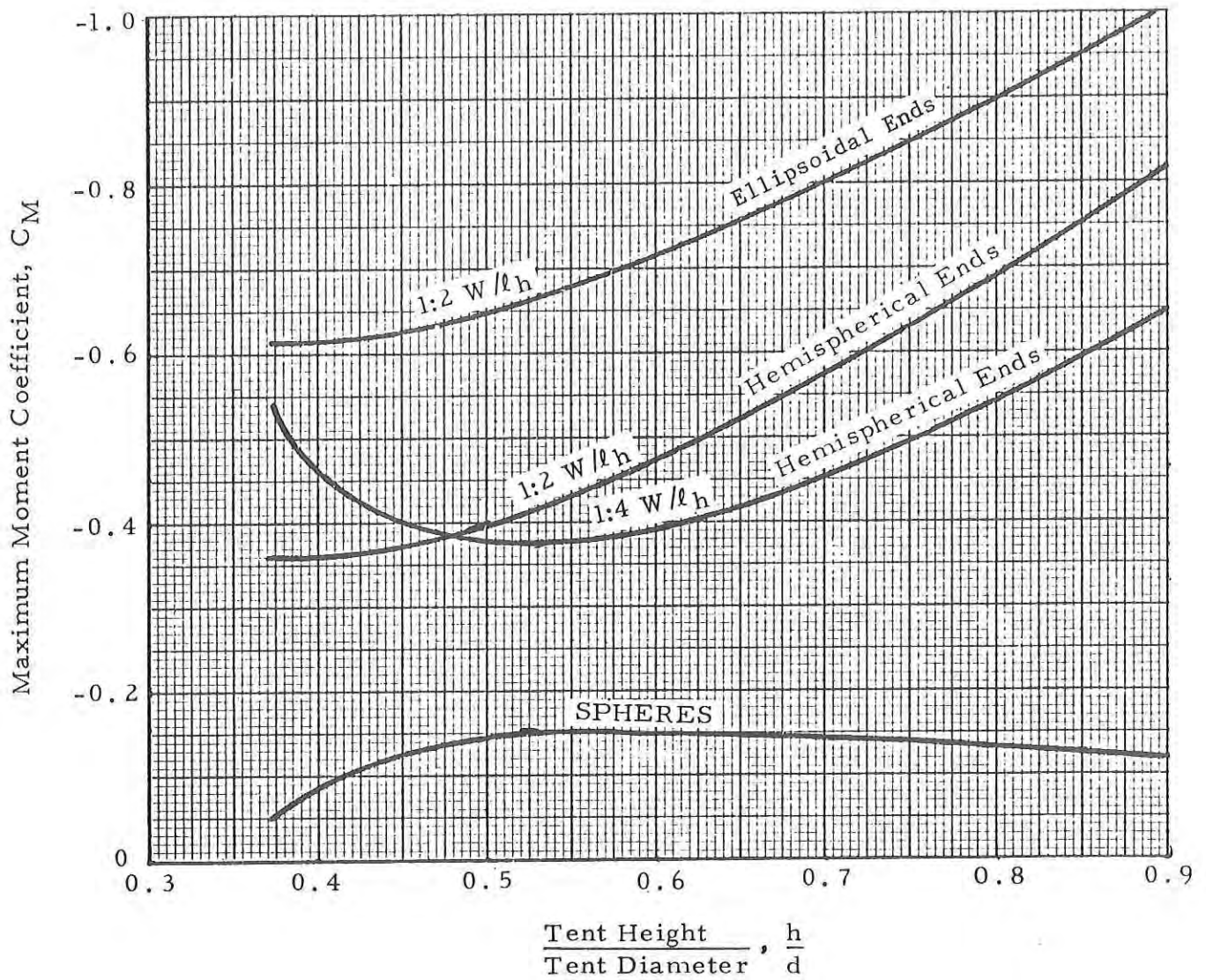
Figure 13. Variation of Moment Coefficient with Shape (Spherical and Cylindrical Single-Wall Tents; 1:2, 1:4, W/\ell_h )
