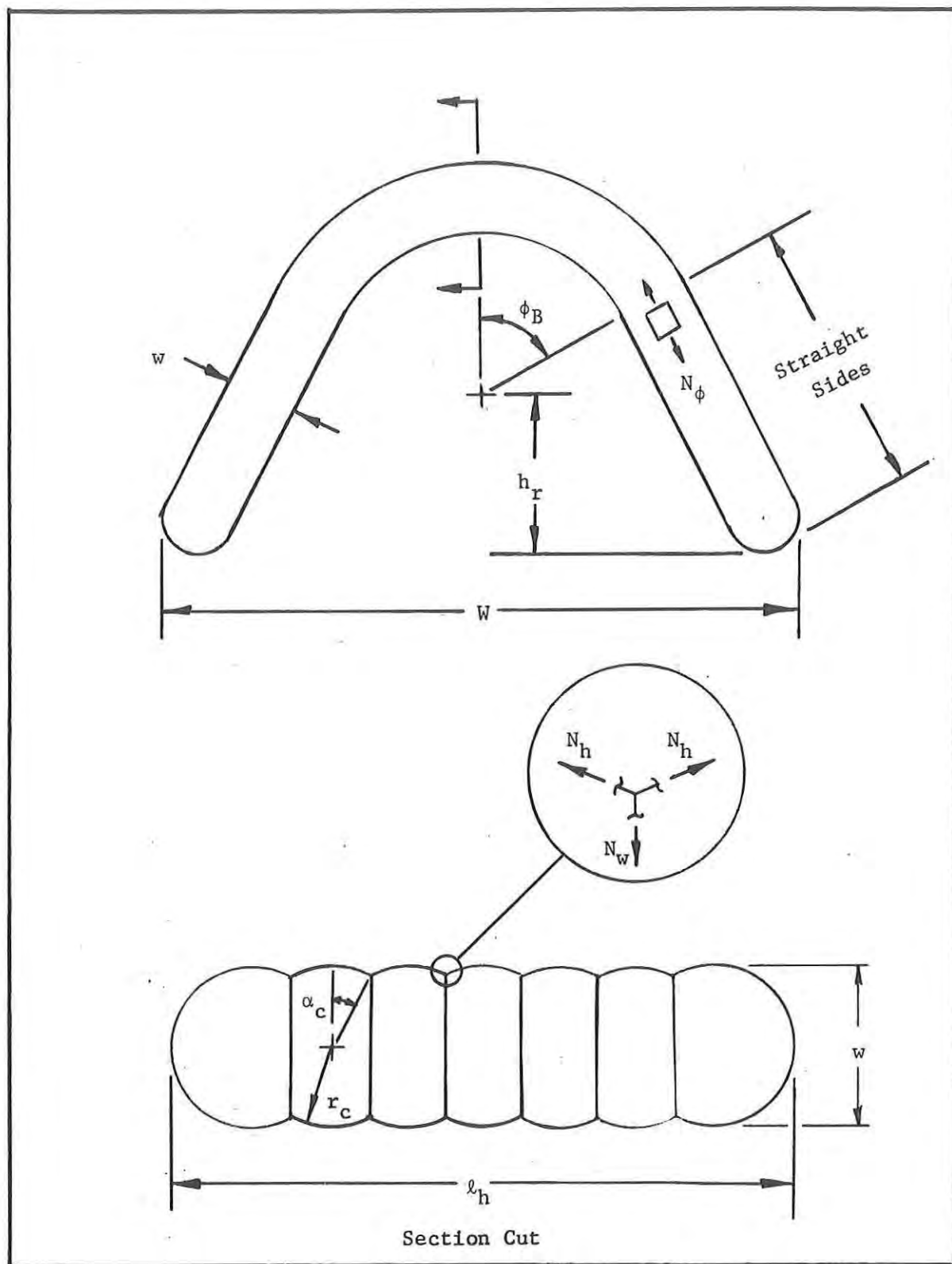
Figure 52. Coordinate System and Stress Resultants for a Double-Wall Cylindrical Tent with Straight Sides
